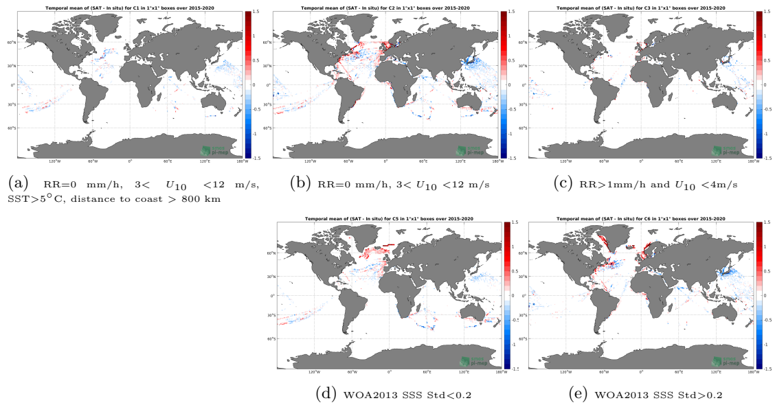
Figure 12: Temporal mean gridded over spatial boxes of size 1^\circ \times 1^\circ of \Delta SSS (SMAP SSS L3 v4 - 8-Day running (RSS) - TSG (LEGOS-DM)) for 5 different subdatasets corresponding to: RR=0 mm/h, 3 < U_{10} < 12 m/s, SST > 5°C, distance to coast > 800 km (a), RR=0 mm/h, 3 < U_{10} < 12 m/s (b), RR > 1mm/h and U_{10} < 4 m/s (c), WOA2013 SSS Std < 0.2 (d), WOA2013 SSS Std > 0.2 (e).
