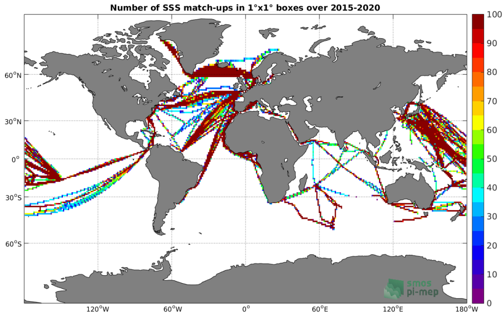
Figure 4: Number of SSS match-ups between TSG (LEGOS-DM) SSS and the SMAP SSS L3 v4 - 8-Day running (RSS) SSS product for the Global Ocean Pi-MEP region over 1^\circ \times 1^\circ boxes and for the full satellite product period.
