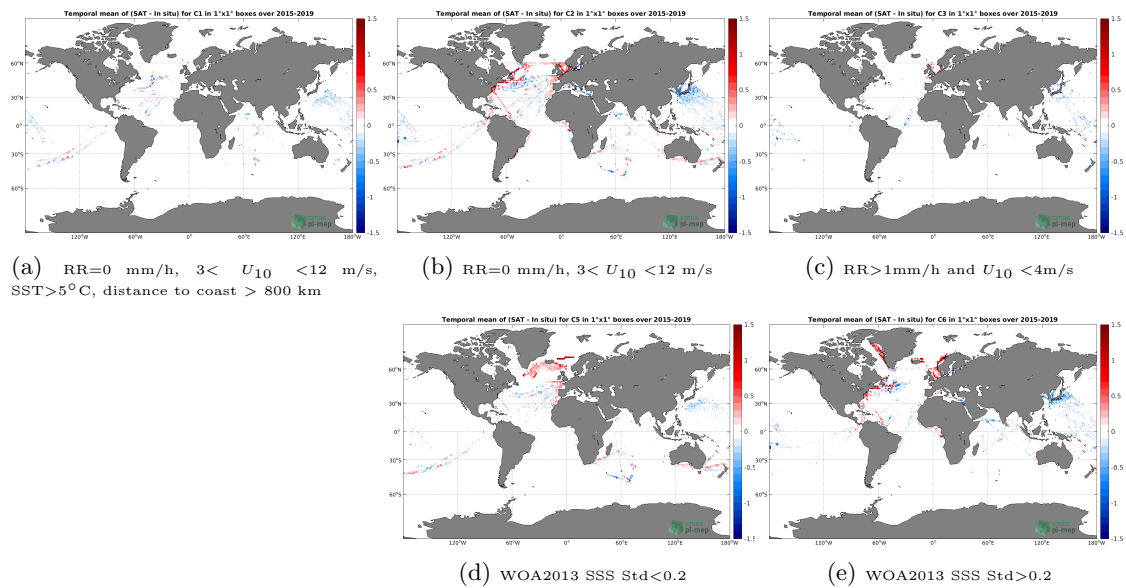
Figure 12: Temporal mean gridded over spatial boxes of size 1^\circ \times 1^\circ of \Delta\text{SSS} (SMAP SSS L3 v4 - 8-Day running (RSS) - TSG (LEGOS-DM)) for 5 different subdatasets corresponding to:RR=0 mm/h, 3 < U_{10} < 12 m/s, SST >5^\circ\text{C} , distance to coast > 800 km (a), RR=0 mm/h, 3 < U_{10} < 12 m/s (b), RR >1 mm/h and U_{10} < 4 m/s (c), WOA2013 SSS Std <0.2 (d), WOA2013 SSS Std >0.2 (e).
