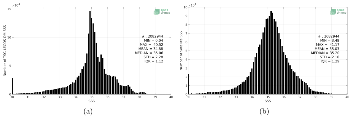
Figure 2: Histograms of SSS from TSG-LEGOS-DM (a) and SMAP-L3-RSS-V4-8DAY-RUNNING (b) considering all match-up pairs per bins of 0.1 over the Global Ocean Pi-MEP region and for the full satellite product period.
