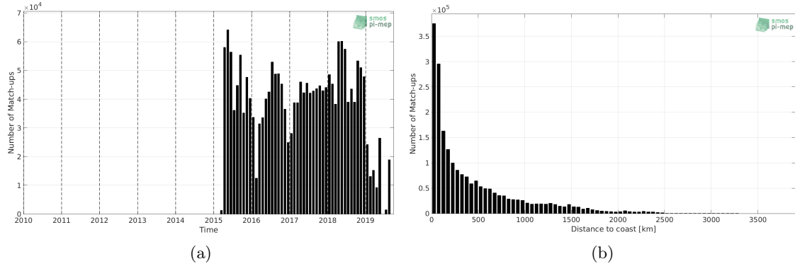
Figure 1: Number of match-ups between TSG-LEGOS-DM and SMAP-L3-RSS-V4-8DAY-RUNNING SSS as a function of time (a) and as function of the distance to coast (b) over the Global Ocean Pi-MEP region and for the full satellite product period.
