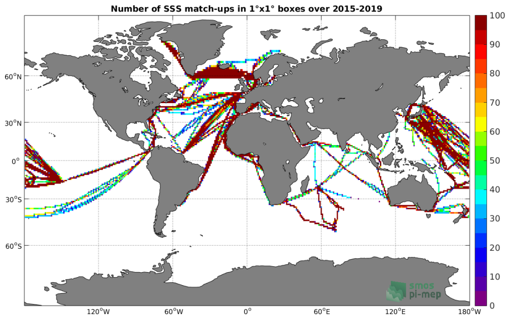
Figure 4: Number of SSS match-ups between TSG-LEGOS-DM SSS and the SMAP-L3-RSS-V4-8DAY-RUNNING SSS product for the Global Ocean Pi-MEP region over 1°x1° boxes and for the full satellite product period.
