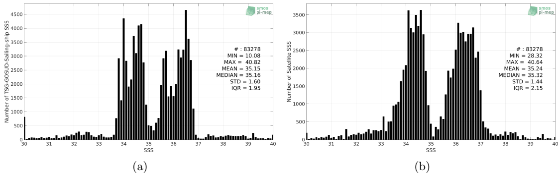
Figure 2: Histograms of SSS from TSG-GOSUD-Sailing-ship (a) and SMAP-L3-RSS-V4-8DAY-RUNNING (b) considering all match-up pairs per bins of 0.1 over the Global Ocean Pi-MEP region and for the full satellite product period.
