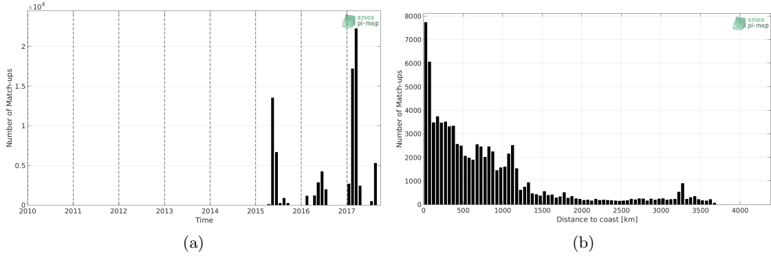
Figure 1: Number of match-ups between TSG-GOSUD-Sailing-ship and SMAP-L3-RSS-V4-8DAY-RUNNING SSS as a function of time (a) and as function of the distance to coast (b) over the Global Ocean Pi-MEP region and for the full satellite product period.
