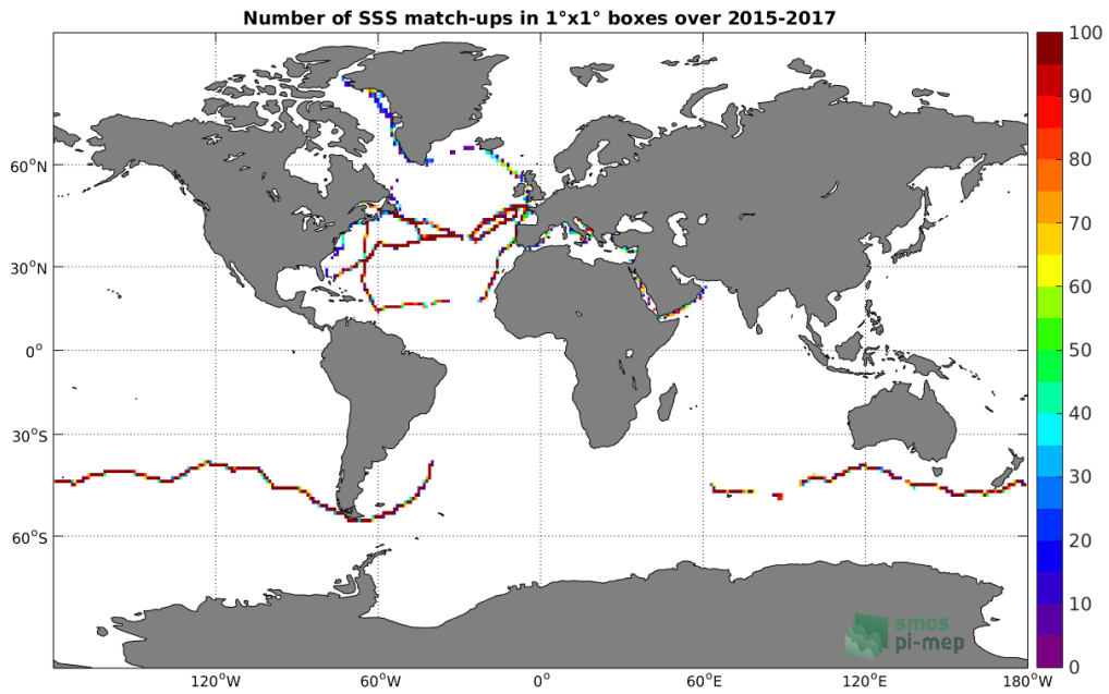
Figure 4: Number of SSS match-ups between TSG-GOSUD-Sailing-ship SSS and the SMAP-L3-RSS-V4-8DAY-RUNNING SSS product for the Global Ocean Pi-MEP region over 1^\circ \times 1^\circ boxes and for the full satellite product period.
