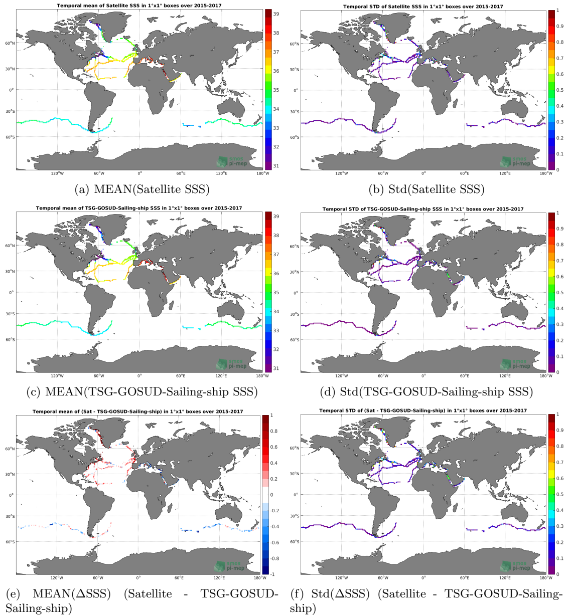
Figure 6: Temporal mean (left) and Std (right) of SSS from SMAP-L3-RSS-V4-8DAY-RUNNING (top), TSG-GOSUD-Sailing-ship (middle), and of \Delta SSS (Satellite - TSG-GOSUD-Sailing-ship). Only match-up pairs are used to generate these maps.
