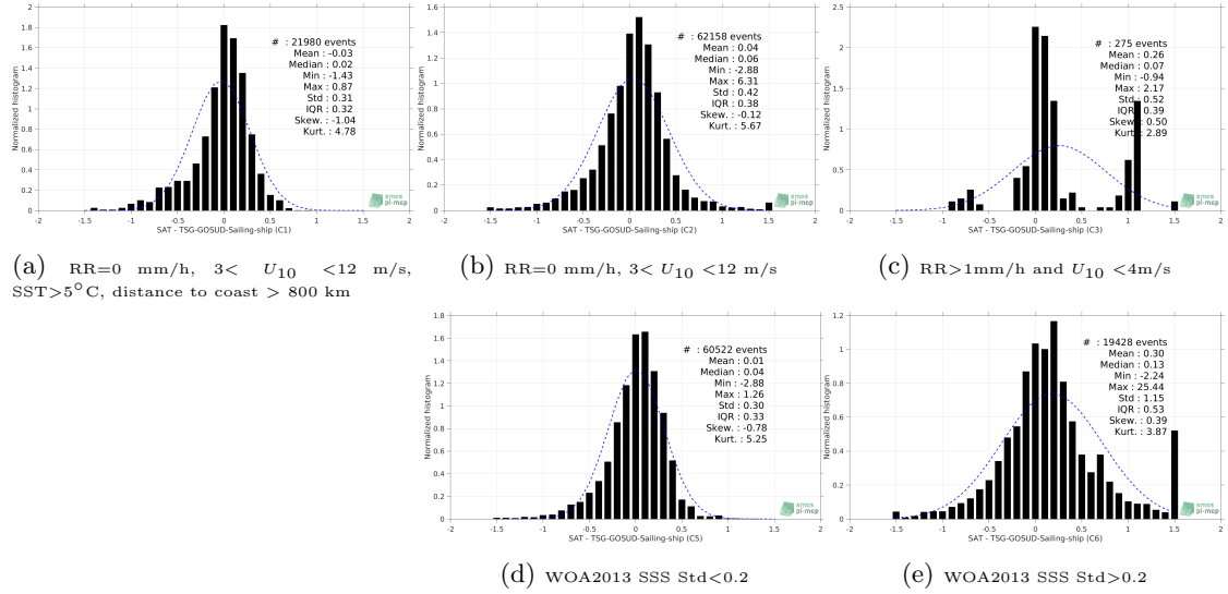
Figure 13: Normalized histogram of \Delta SSS (SMAP-L3-RSS-V4-8DAY-RUNNING - TSG-GOSUD-Sailing-ship) for 5 different subdatasets corresponding to: RR=0 mm/h, 3 < U_{10} < 12 m/s, SST >5^{\circ} C, distance to coast > 800 km (a), RR=0 mm/h, 3 < U_{10} < 12 m/s (b), RR >1 mm/h and U_{10} < 4 m/s (c), WOA2013 SSS Std <0.2 (d), WOA2013 SSS Std >0.2 (e).
