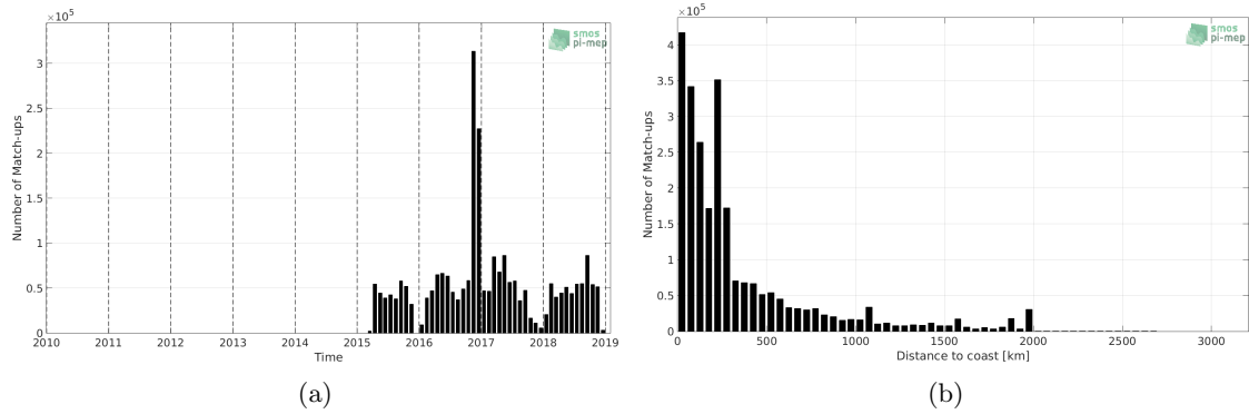
Figure 1: Number of match-ups between TSG-GOSUD-Research-vessel and SMAP-L3-RSS-V4-8DAY-RUNNING SSS as a function of time (a) and as function of the distance to coast (b) over the Global Ocean Pi-MEP region and for the full satellite product period.
