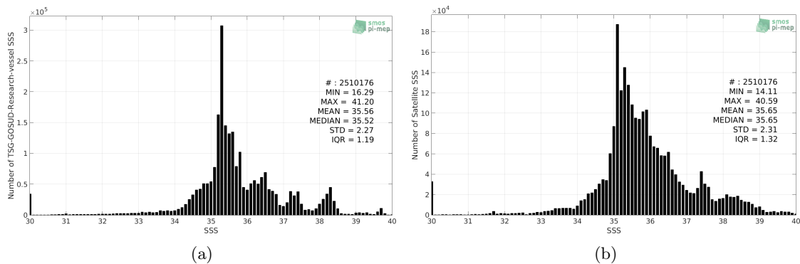
Figure 2: Histograms of SSS from TSG-GOSUD-Research-vessel (a) and SMAP-L3-RSS-V4-8DAY-RUNNING (b) considering all match-up pairs per bins of 0.1 over the Global Ocean Pi-MEP region and for the full satellite product period.
