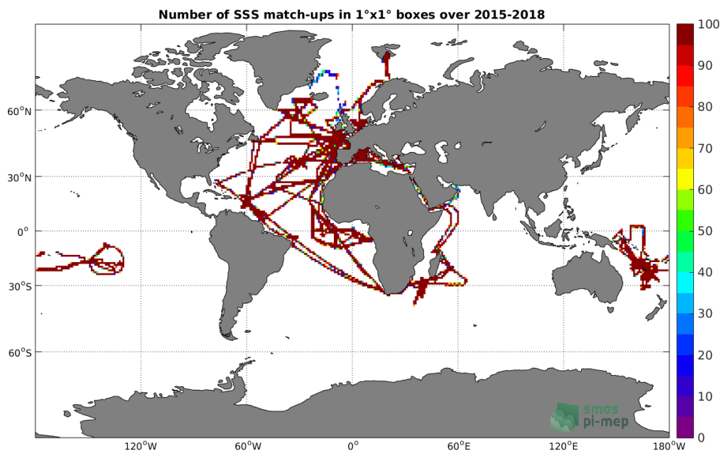
Figure 4: Number of SSS match-ups between TSG-GOSUD-Research-vessel SSS and the SMAP-L3-RSS-V4-8DAY-RUNNING SSS product for the Global Ocean Pi-MEP region over 1^\circ \times 1^\circ boxes and for the full satellite product period.
