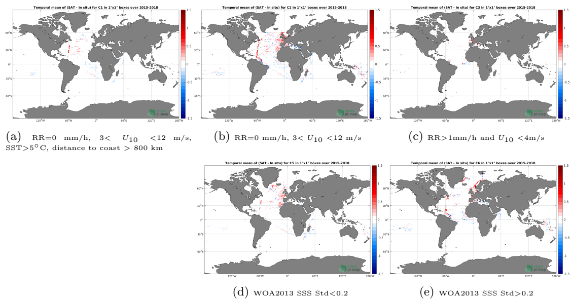
Figure 12: Temporal mean gridded over spatial boxes of size 1^\circ \times 1^\circ of \Delta SSS (SMAP-L3-RSS-V4-8DAY-RUNNING - TSG-GOSUD-Research-vessel) for 5 different subdatasets corresponding to:RR=0 mm/h, 3 < U_{10} < 12 m/s, SST >5^\circ C, distance to coast > 800 km (a), RR=0 mm/h, 3 < U_{10} < 12 m/s (b), RR >1 mm/h and U_{10} < 4 m/s (c), WOA2013 SSS Std <0.2 (d), WOA2013 SSS Std >0.2 (e).
