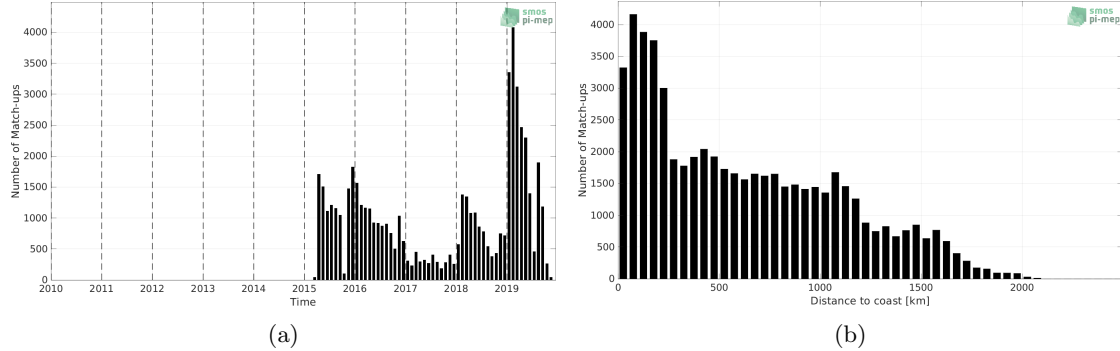
Figure 1: Number of match-ups between Marine mammals and SMAP SSS L3 v4 - 8-Day running (RSS) SSS as a function of time (a) and as function of the distance to coast (b) over the Global Ocean Pi-MEP region and for the full satellite product period.
