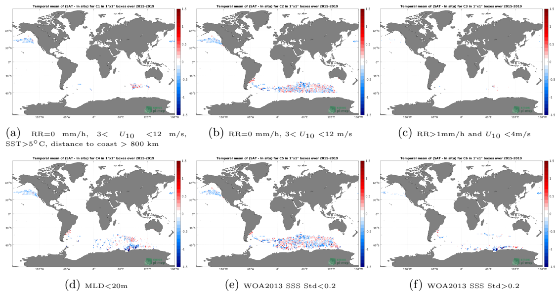
Figure 12: Temporal mean gridded over spatial boxes of size 1^\circ \times 1^\circ of \Delta SSS (SMAP SSS L3 v4 - 8-Day running (RSS) - Marine mammals) for 6 different subdatasets corresponding to:RR=0 mm/h, 3 < U_{10} < 12 m/s, SST >5^\circ C, distance to coast > 800 km (a), RR=0 mm/h, 3 < U_{10} < 12 m/s (b), RR >1 mm/h and U_{10} < 4 m/s (c),MLD <20 m (d),WOA2013 SSS Std <0.2 (e),WOA2013 SSS Std >0.2 (f).
