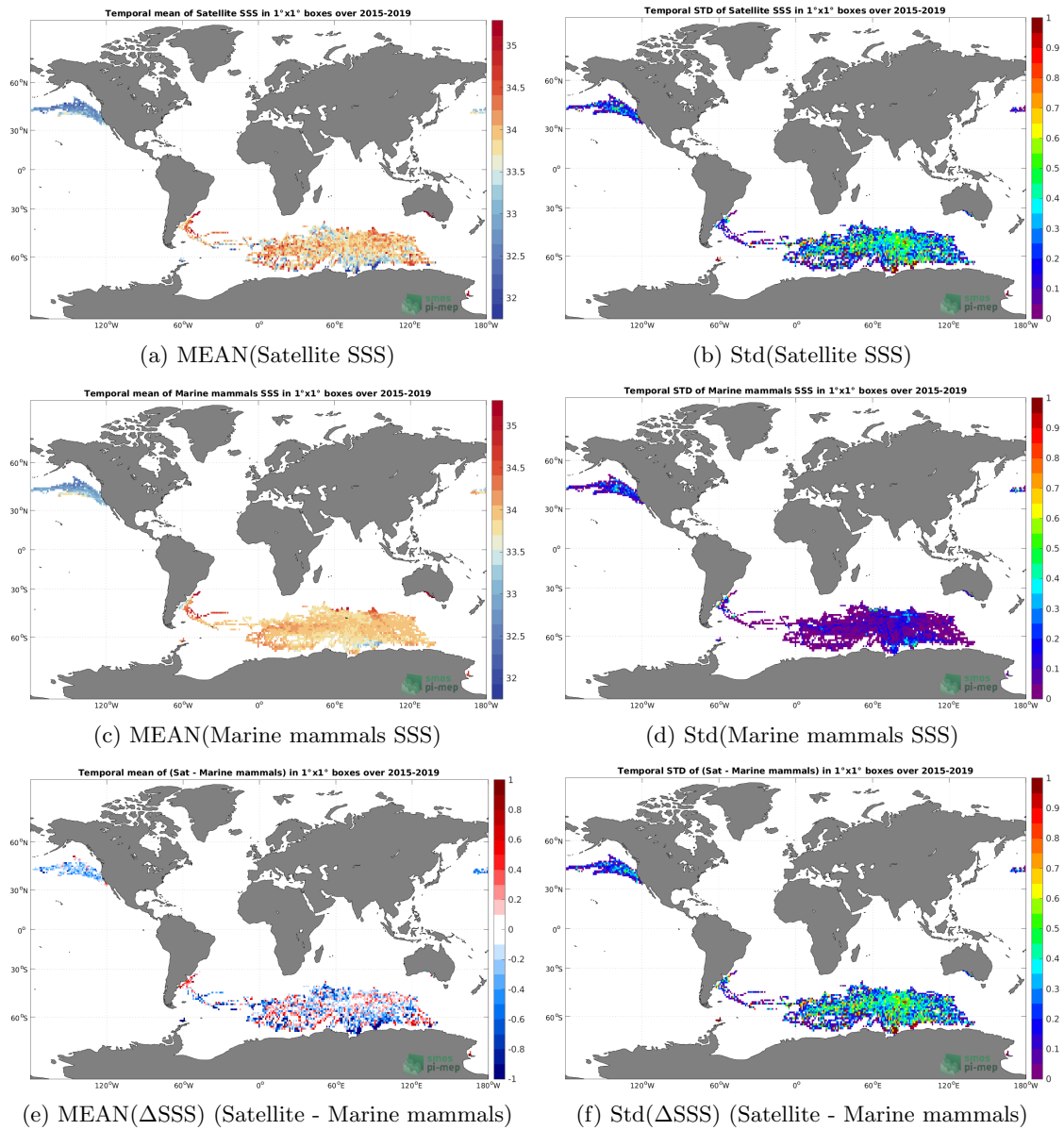
Figure 6: Temporal mean (left) and Std (right) of SSS from SMAP SSS L3 v4 - 8-Day running (RSS) (top), Marine mammals (middle), and of \Delta SSS (Satellite - Marine mammals). Only match-up pairs are used to generate these maps.
