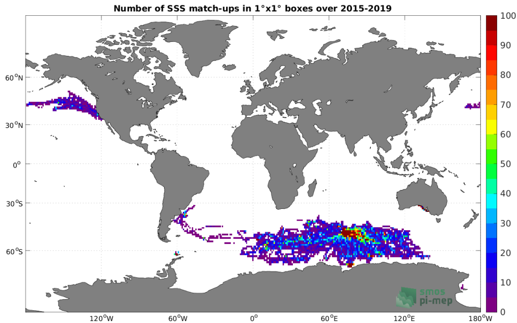
Figure 4: Number of SSS match-ups between Marine mammals SSS and the SMAP SSS L3 v4 - 8-Day running (RSS) SSS product for the Global Ocean Pi-MEP region over 1^\circ \times 1^\circ boxes and for the full satellite product period.
