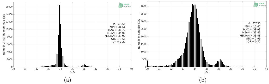
Figure 2: Histograms of SSS from Marine mammals (a) and SMAP SSS L3 v4 - 8-Day running (RSS) (b) considering all match-up pairs per bins of 0.1 over the Global Ocean Pi-MEP region and for the full satellite product period.
