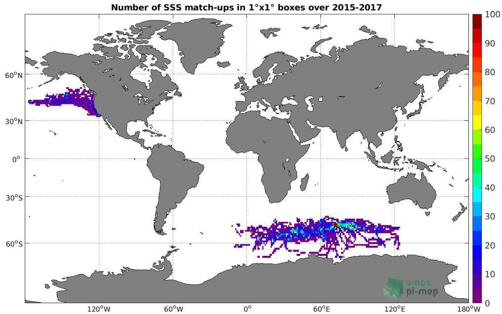
Figure 4: Number of SSS match-ups between Sea mammals SSS and the SMAP SSS L3 v4 - 8-Day running (RSS) SSS product for the Global Ocean Pi-MEP region over 1^\circ \times 1^\circ boxes and for the full satellite product period.
