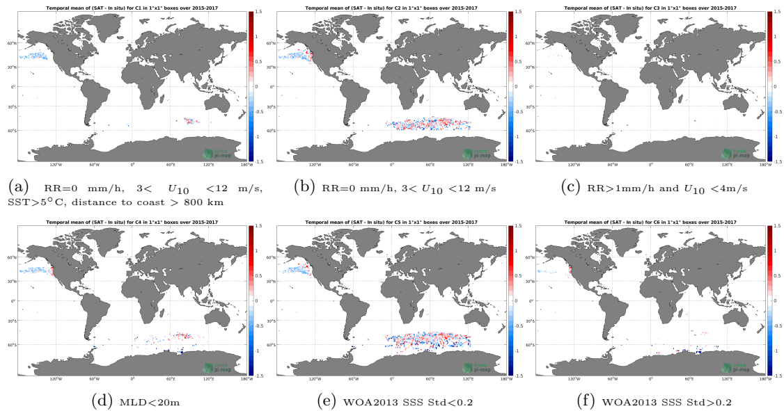
Figure 12: Temporal mean gridded over spatial boxes of size 1^\circ \times 1^\circ of \Delta SSS (SMAP SSS L3 v4 - 8-Day running (RSS) - Sea mammals) for 6 different subdatasets corresponding to:RR=0 mm/h, 3 < U_{10} < 12 m/s, SST > 5^\circ\text{C} , distance to coast > 800 km (a), RR=0 mm/h, 3 < U_{10} < 12 m/s (b), RR > 1 mm/h and U_{10} < 4 m/s (c),MLD < 20 m (d),WOA2013 SSS Std < 0.2 (e),WOA2013 SSS Std > 0.2 (f).
