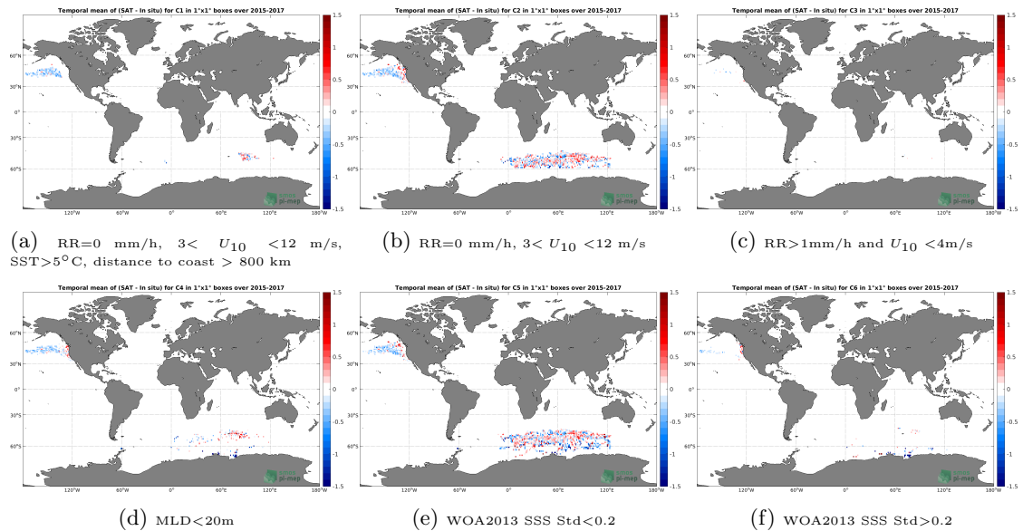
Figure 12: Temporal mean gridded over spatial boxes of size 1°x1° of \Delta SSS (SMAP SSS L3 v4 - 8-Day running (RSS) - Sea mammals) for 6 different subdatasets corresponding to:RR=0 mm/h, 3 < U_{10} < 12 m/s, SST>5°C, distance to coast > 800 km (a), RR=0 mm/h, 3 < U_{10} < 12 m/s (b), RR>1mm/h and U_{10} < 4 m/s (c),MLD<20m (d),WOA2013 SSS Std<0.2 (e),WOA2013 SSS Std>0.2 (f).
