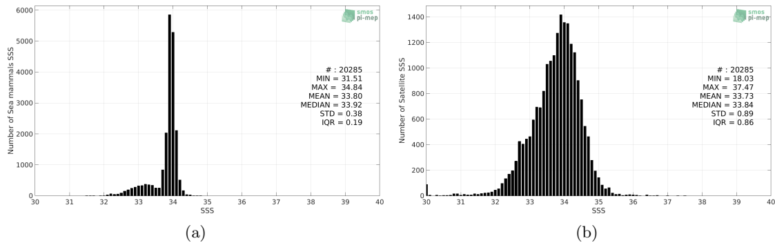
Figure 2: Histograms of SSS from Sea mammals (a) and SMAP SSS L3 v4 - 8-Day running (RSS) (b) considering all match-up pairs per bins of 0.1 over the Global Ocean Pi-MEP region and for the full satellite product period.
