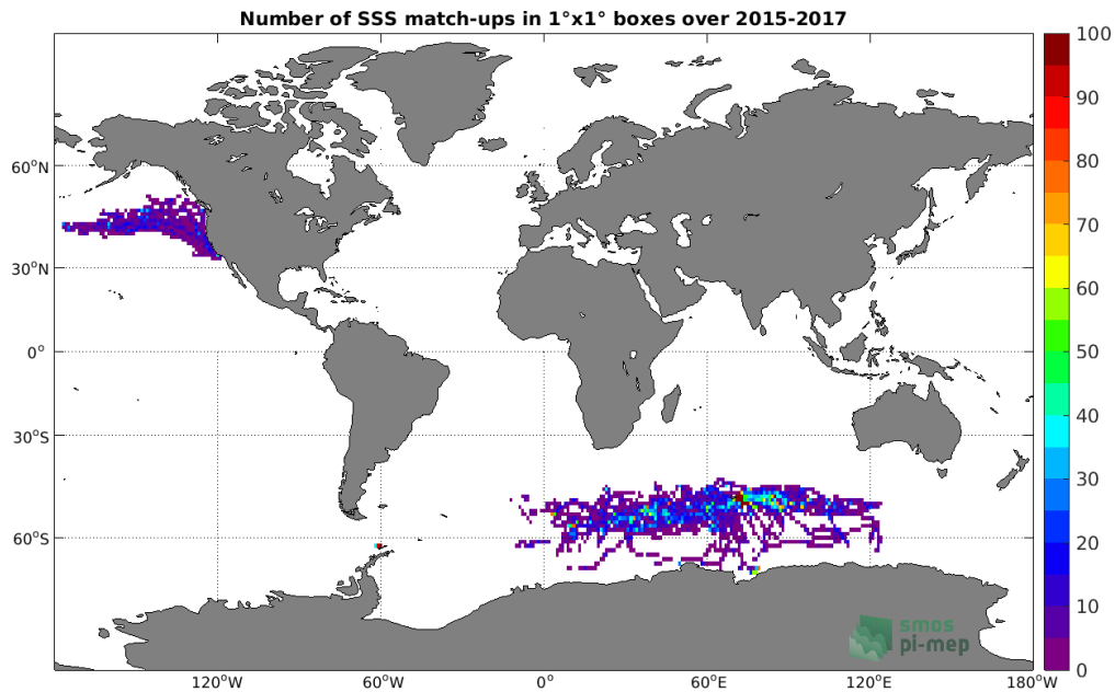
Figure 4: Number of SSS match-ups between Sea mammals SSS and the SMAP SSS L3 v4 - 8-Day running (RSS) SSS product for the Global Ocean Pi-MEP region over 1°x1° boxes and for the full satellite product period.
