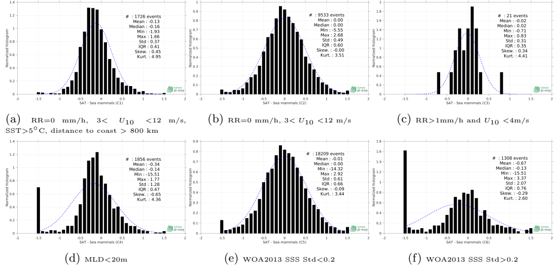
Figure 13: Normalized histogram of \Delta SSS (SMAP SSS L3 v4 - 8-Day running (RSS) - Sea mammals) for 6 different subdatasets corresponding to: RR=0 mm/h, 3 < U_{10} < 12 m/s, SST>5°C, distance to coast > 800 km (a), RR=0 mm/h, 3 < U_{10} < 12 m/s (b), RR>1mm/h and U_{10} < 4 m/s (c), MLD<20m (d), WOA2013 SSS Std<0.2 (e), WOA2013 SSS Std>0.2 (f).
