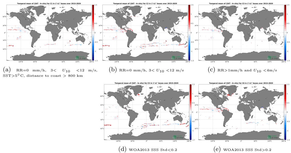
Figure 11: Temporal mean gridded over spatial boxes of size 1^\circ \times 1^\circ of \Delta\text{SSS} (SMAP SSS L3 v4 - 8-Day running (RSS) - Surface drifters) for 5 different subdatasets corresponding to:RR=0 mm/h, 3 < U_{10} < 12 m/s, SST > 5^\circ\text{C} , distance to coast > 800 km (a), RR=0 mm/h, 3 < U_{10} < 12 m/s (b), RR > 1 mm/h and U_{10} < 4 m/s (c), WOA2013 SSS Std < 0.2 (d), WOA2013 SSS Std > 0.2 (e).
