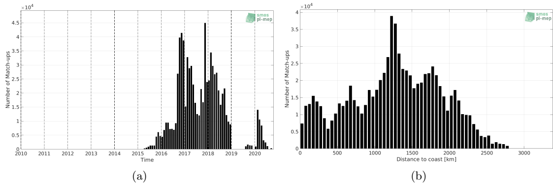
Figure 1: Number of match-ups between Surface drifters and SMAP SSS L3 v4 - 8-Day running (RSS) SSS as a function of time (a) and as function of the distance to coast (b) over the Global Ocean Pi-MEP region and for the full satellite product period.
