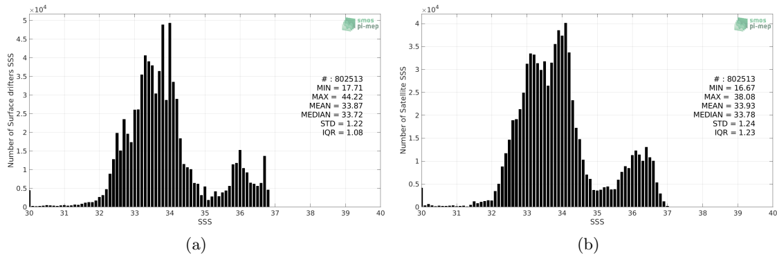
Figure 2: Histograms of SSS from Surface drifters (a) and SMAP SSS L3 v4 - 8-Day running (RSS) (b) considering all match-up pairs per bins of 0.1 over the Global Ocean Pi-MEP region and for the full satellite product period.
