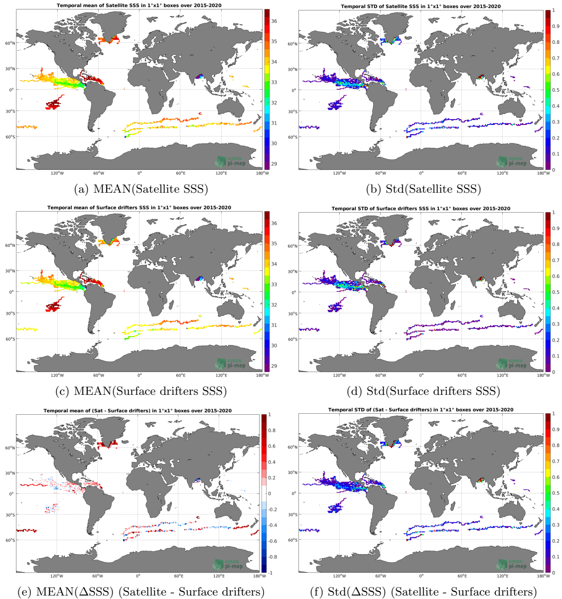
Figure 5: Temporal mean (left) and Std (right) of SSS from SMAP SSS L3 v4 - 8-Day running (RSS) (top), Surface drifters (middle), and of \Delta SSS (Satellite - Surface drifters). Only match-up pairs are used to generate these maps.
