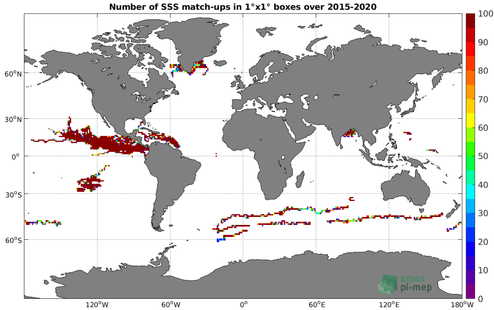
Figure 3: Number of SSS match-ups between Surface drifters SSS and the SMAP SSS L3 v4 - 8-Day running (RSS) SSS product for the Global Ocean Pi-MEP region over 1^\circ \times 1^\circ boxes and for the full satellite product period.
