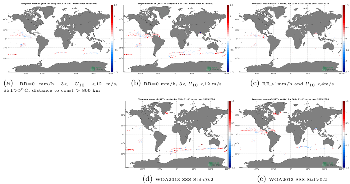
Figure 11: Temporal mean gridded over spatial boxes of size 1^\circ \times 1^\circ of \Delta SSS (SMAP SSS L3 v4 - 8-Day running (RSS) - Surface drifters) for 5 different subdatasets corresponding to:RR=0 mm/h, 3 < U_{10} < 12 m/s, SST > 5^\circ\text{C} , distance to coast > 800 km (a), RR=0 mm/h, 3 < U_{10} < 12 m/s (b), RR > 1 mm/h and U_{10} < 4 m/s (c), WOA2013 SSS Std < 0.2 (d), WOA2013 SSS Std > 0.2 (e).
