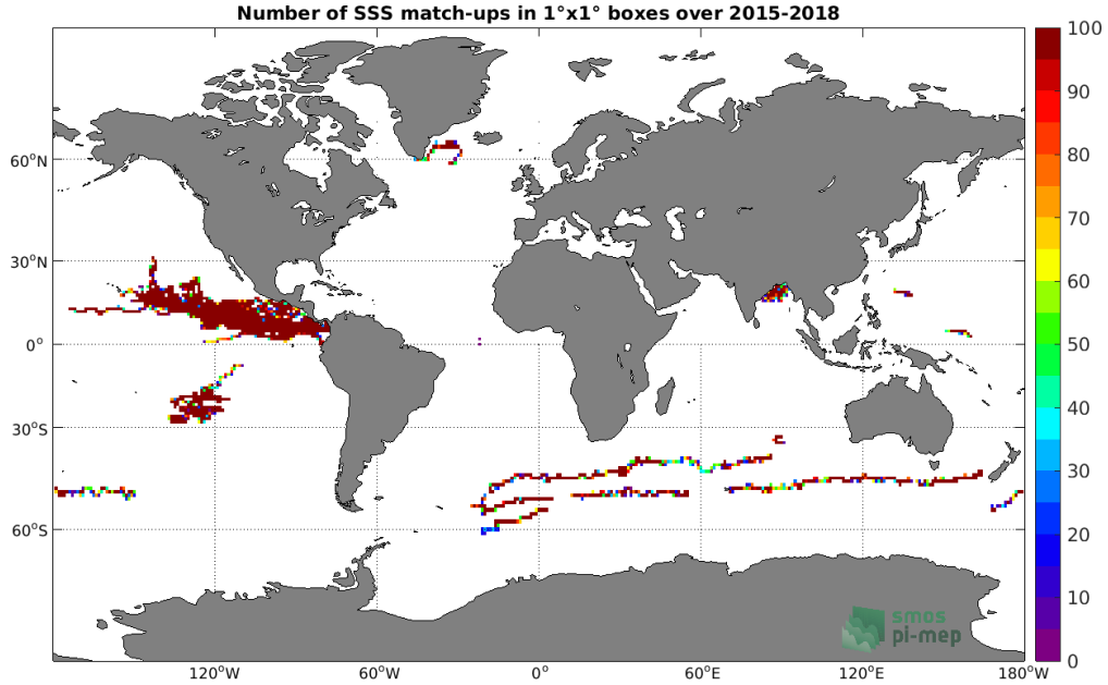
Figure 3: Number of SSS match-ups between Surface drifters SSS and the SMAP SSS L3 v4 - 8-Day running (RSS) SSS product for the Global Ocean Pi-MEP region over 1°x1° boxes and for the full satellite product period.
