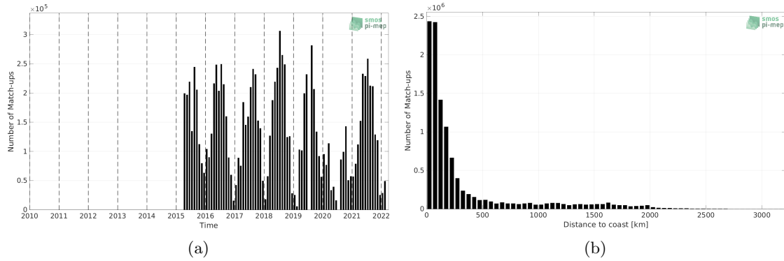
Figure 1: Number of match-ups between TSG (SAMOS) and SMAP SSS L3 v4 - Monthly (RSS) SSS as a function of time (a) and as function of the distance to coast (b) over the Global Ocean Pi-MEP region and for the full satellite product period.
