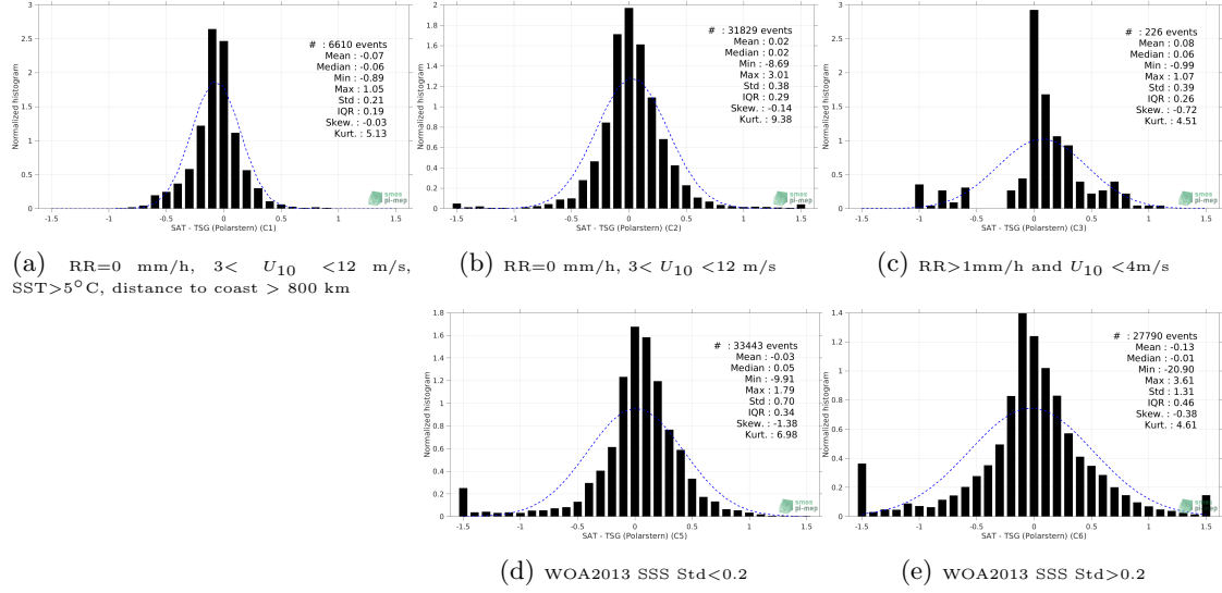
Figure 13: Normalized histogram of \Delta SSS (SMAP SSS L3 v4 - Monthly (RSS) - TSG (Polarstern)) for 5 different subdatasets corresponding to: RR=0 mm/h, 3 < U_{10} < 12 m/s, SST>5°C, distance to coast > 800 km (a), RR=0 mm/h, 3 < U_{10} < 12 m/s (b), RR>1mm/h and U_{10} < 4 m/s (c), WOA2013 SSS Std<0.2 (d), WOA2013 SSS Std>0.2 (e).
