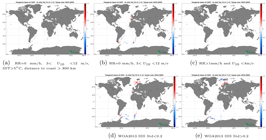
Figure 12: Temporal mean gridded over spatial boxes of size 1^\circ \times 1^\circ of \Delta SSS (SMAP SSS L3 v4 - Monthly (RSS) - TSG (Polarstern)) for 5 different subdatasets corresponding to: RR=0 mm/h, 3 < U_{10} < 12 m/s, SST > 5^\circ C , distance to coast > 800 km (a), RR=0 mm/h, 3 < U_{10} < 12 m/s (b), RR > 1 mm/h and U_{10} < 4 m/s (c), WOA2013 SSS Std < 0.2 (d), WOA2013 SSS Std > 0.2 (e).
