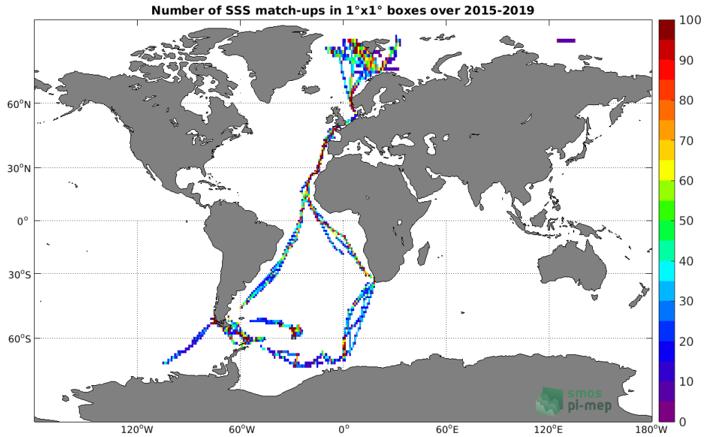
Figure 4: Number of SSS match-ups between TSG (Polarstern) SSS and the SMAP SSS L3 v4 - Monthly (RSS) SSS product for the Global Ocean Pi-MEP region over 1^\circ \times 1^\circ boxes and for the full satellite product period.
