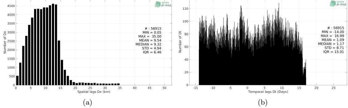
Figure 5: Histograms of the spatial (a) and temporal (b) lags between the time of the TSG (Polarstern) measurements and the date of the corresponding SMAP SSS L3 v4 - Monthly (RSS) SSS product.
