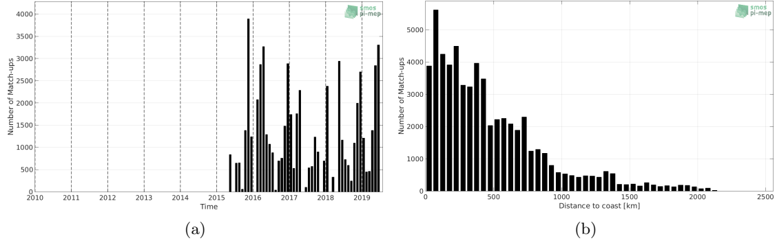
Figure 1: Number of match-ups between TSG-POLARSTERN and SMAP-L3-RSS-V4-MONTHLY SSS as a function of time (a) and as function of the distance to coast (b) over the Global Ocean Pi-MEP region and for the full satellite product period.
