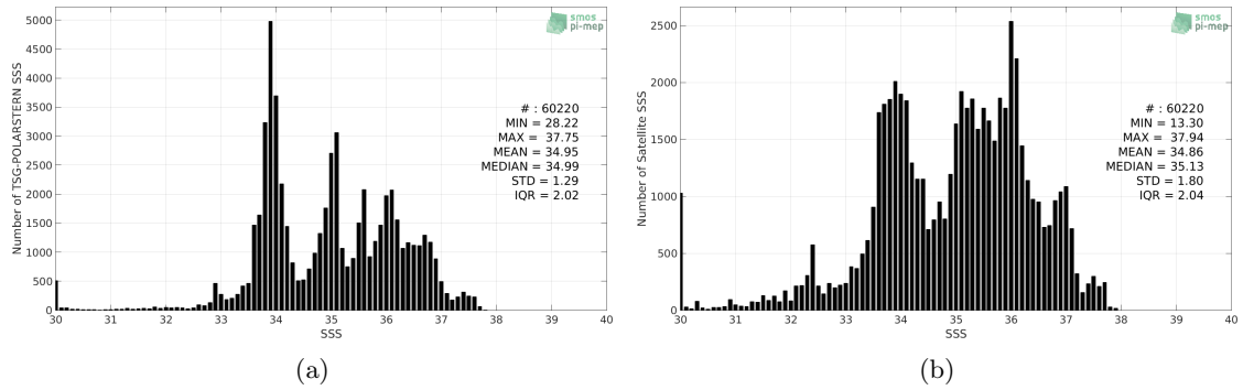
Figure 2: Histograms of SSS from TSG-POLARSTERN (a) and SMAP-L3-RSS-V4-MONTHLY (b) considering all match-up pairs per bins of 0.1 over the Global Ocean Pi-MEP region and for the full satellite product period.
