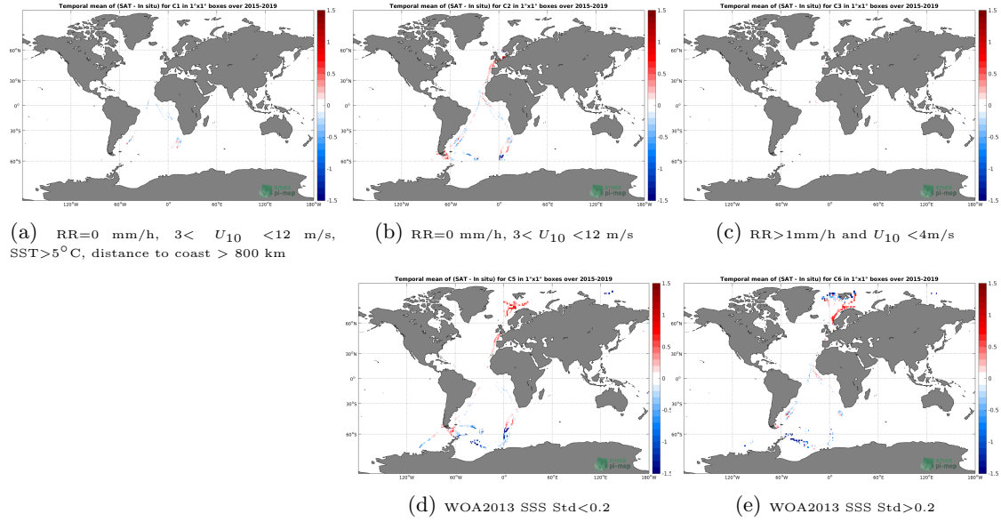
Figure 12: Temporal mean gridded over spatial boxes of size 1^\circ \times 1^\circ of \Delta SSS (SMAP-L3-RSS-V4-MONTHLY - TSG-POLARSTERN) for 5 different subdatasets corresponding to: RR=0 mm/h, 3 < U_{10} < 12 m/s, SST > 5^\circ C , distance to coast > 800 km (a), RR=0 mm/h, 3 < U_{10} < 12 m/s (b), RR > 1 mm/h and U_{10} < 4 m/s (c), WOA2013 SSS Std < 0.2 (d), WOA2013 SSS Std > 0.2 (e).
