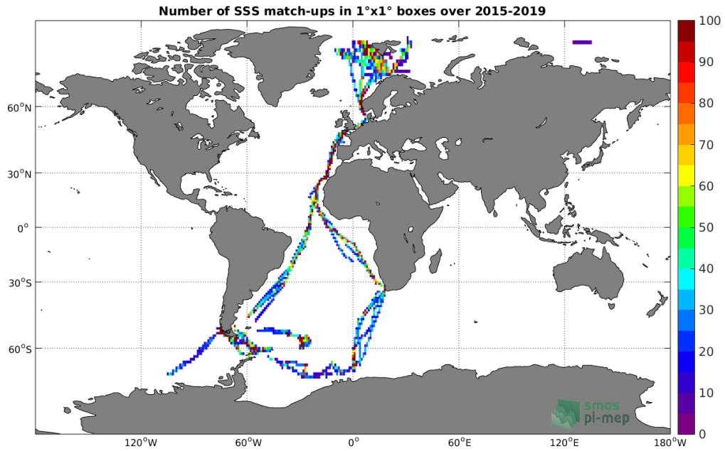
Figure 4: Number of SSS match-ups between TSG-POLARSTERN SSS and the SMAP-L3-RSS-V4-MONTHLY SSS product for the Global Ocean Pi-MEP region over 1^\circ \times 1^\circ boxes and for the full satellite product period.
