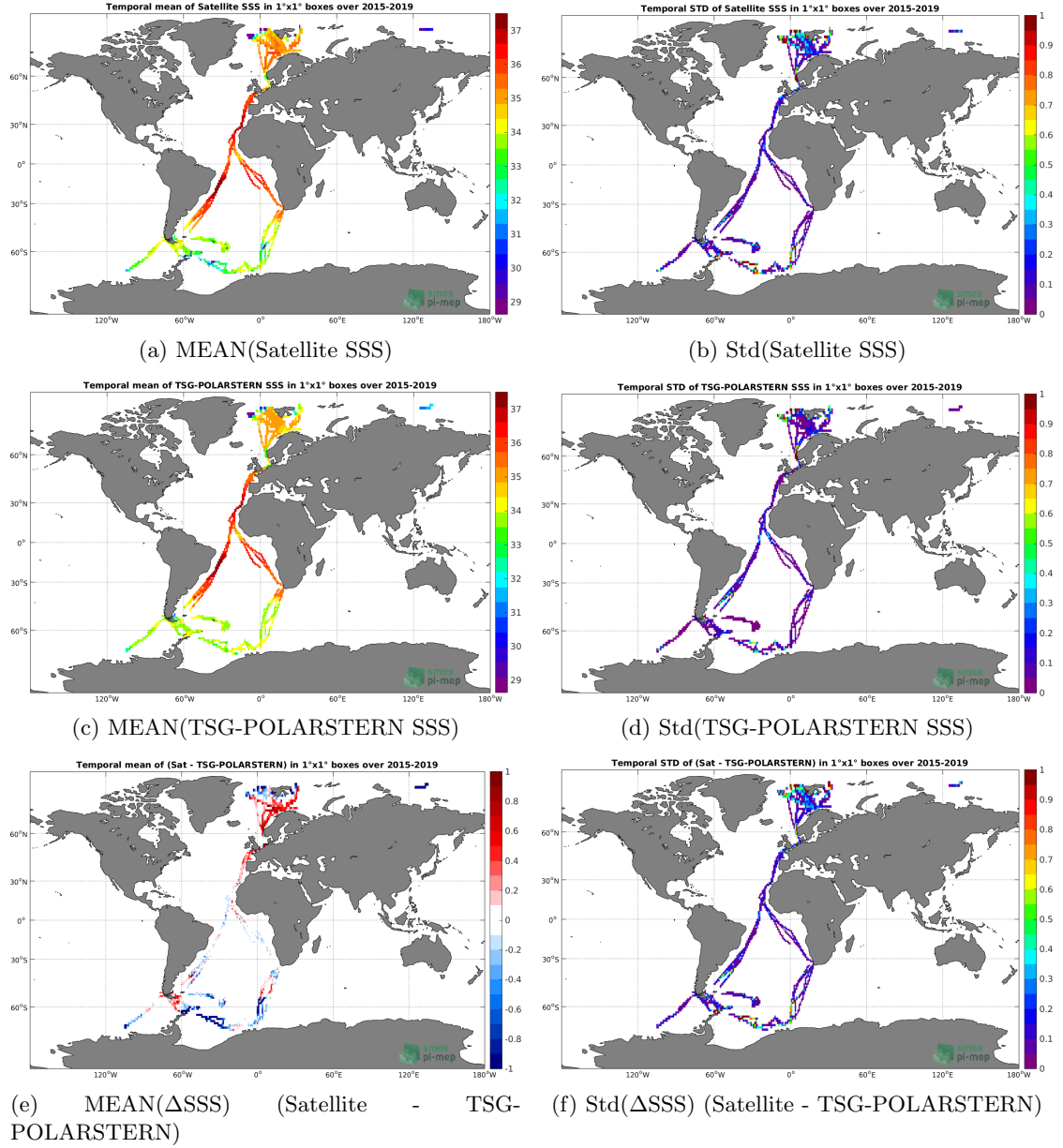
Figure 6: Temporal mean (left) and Std (right) of SSS from SMAP-L3-RSS-V4-MONTHLY (top), TSG-POLARSTERN (middle), and of \Delta SSS (Satellite - TSG-POLARSTERN). Only match-up pairs are used to generate these maps.
