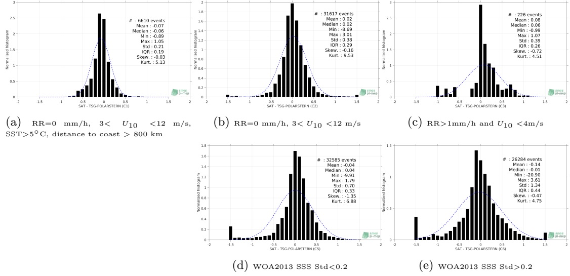
Figure 13: Normalized histogram of \Delta SSS (SMAP-L3-RSS-V4-MONTHLY - TSG-POLARSTERN) for 5 different subdatasets corresponding to: RR=0 mm/h, 3 < U_{10} < 12 m/s, SST>5°C, distance to coast > 800 km (a), RR=0 mm/h, 3 < U_{10} < 12 m/s (b), RR>1mm/h and U_{10} < 4 m/s (c), WOA2013 SSS Std<0.2 (d), WOA2013 SSS Std>0.2 (e).
