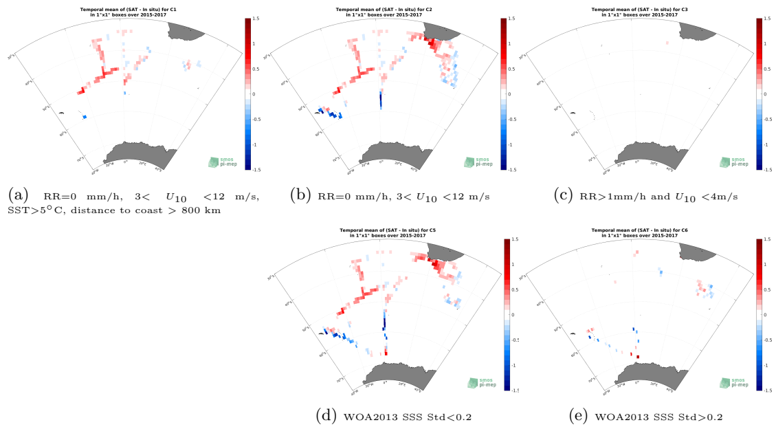
Figure 12: Temporal mean gridded over spatial boxes of size 1^\circ \times 1^\circ of \Delta SSS (SMAP SSS L3 v4 - Monthly (RSS) - TSG (NCEI-0170743)) for 5 different subdatasets corresponding to:RR=0 mm/h, 3 < U_{10} < 12 m/s, SST >5^\circ C, distance to coast > 800 km (a), RR=0 mm/h, 3 < U_{10} < 12 m/s (b), RR >1 mm/h and U_{10} < 4 m/s (c), WOA2013 SSS Std <0.2 (d), WOA2013 SSS Std >0.2 (e).
