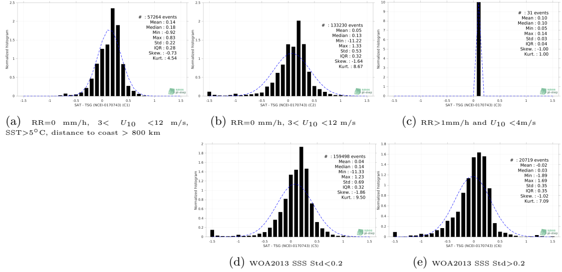
Figure 13: Normalized histogram of \Delta SSS (SMAP SSS L3 v4 - Monthly (RSS) - TSG (NCEI-0170743)) for 5 different subdatasets corresponding to: RR=0 mm/h, 3 < U_{10} < 12 m/s, SST > 5°C, distance to coast > 800 km (a), RR=0 mm/h, 3 < U_{10} < 12 m/s (b), RR > 1mm/h and U_{10} < 4 m/s (c), WOA2013 SSS Std < 0.2 (d), WOA2013 SSS Std > 0.2 (e).
