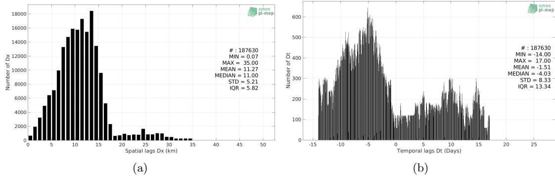
Figure 5: Histograms of the spatial (a) and temporal (b) lags between the location/time of the TSG (NCEI-0170743) measurement and the date of the corresponding SMAP SSS L3 v4 - Monthly (RSS) SSS pixel.
