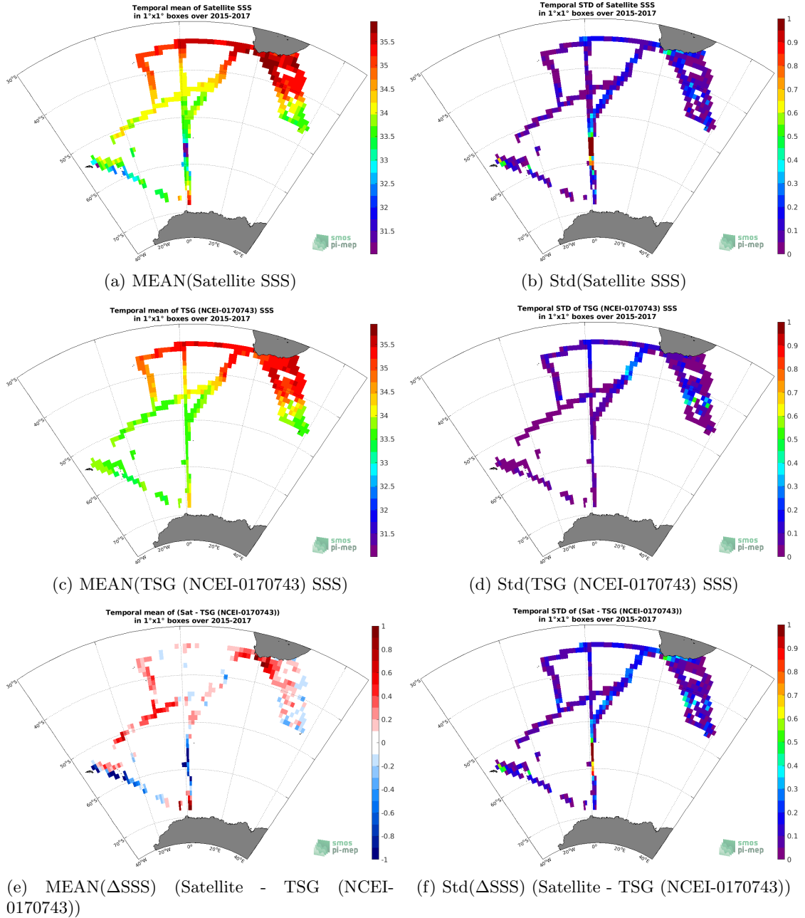
Figure 6: Temporal mean (left) and Std (right) of SSS from SMAP SSS L3 v4 - Monthly (RSS) (top), TSG (NCEI-0170743) (middle), and of \Delta SSS (Satellite - TSG (NCEI-0170743)). Only match-up pairs are used to generate these maps.
