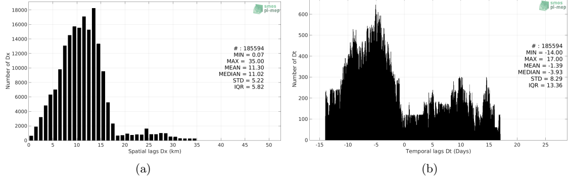
Figure 5: Histograms of the spatial (a) and temporal (b) lags between the time of the TSG (NCEI-0170743) measurements and the date of the corresponding SMAP SSS L3 v4 - Monthly (RSS) SSS product.
