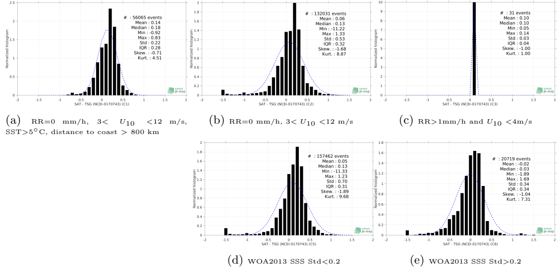
Figure 13: Normalized histogram of \Delta SSS (SMAP SSS L3 v4 - Monthly (RSS) - TSG (NCEI-0170743)) for 5 different subdatasets corresponding to: RR=0 mm/h, 3 < U_{10} < 12 m/s, SST>5°C, distance to coast > 800 km (a), RR=0 mm/h, 3 < U_{10} < 12 m/s (b), RR>1mm/h and U_{10} < 4 m/s (c), WOA2013 SSS Std<0.2 (d), WOA2013 SSS Std>0.2 (e).
