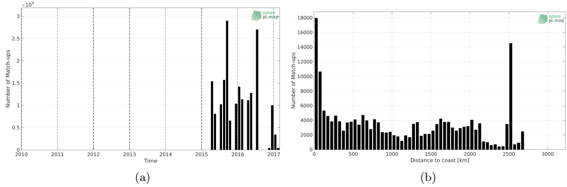
Figure 1: Number of match-ups between TSG (NCEI-0170743) and SMAP SSS L3 v4 - Monthly (RSS) SSS as a function of time (a) and as function of the distance to coast (b) over the Global Ocean Pi-MEP region and for the full satellite product period.
