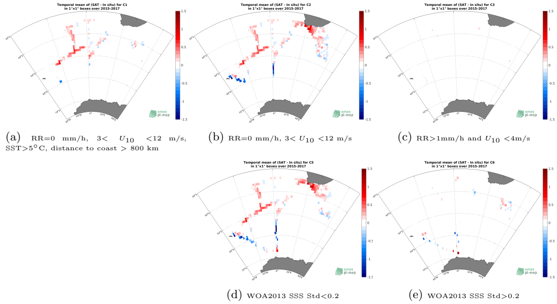
Figure 12: Temporal mean gridded over spatial boxes of size 1^\circ \times 1^\circ of \Delta SSS (SMAP SSS L3 v4 - Monthly (RSS) - TSG (NCEI-0170743)) for 5 different subdatasets corresponding to: RR=0 mm/h, 3 < U_{10} < 12 m/s, SST > 5^\circ\text{C} , distance to coast > 800 km (a), RR=0 mm/h, 3 < U_{10} < 12 m/s (b), RR > 1 mm/h and U_{10} < 4 m/s (c), WOA2013 SSS Std < 0.2 (d), WOA2013 SSS Std > 0.2 (e).
