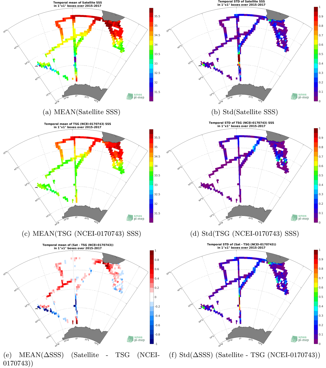
Figure 6: Temporal mean (left) and Std (right) of SSS from SMAP SSS L3 v4 - Monthly (RSS) (top), TSG (NCEI-0170743) (middle), and of \Delta SSS (Satellite - TSG (NCEI-0170743)). Only match-up pairs are used to generate these maps.
