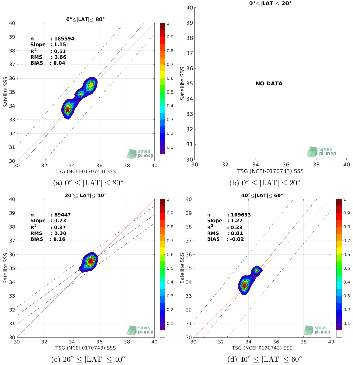
Figure 9: Contour maps of the concentration of SMAP SSS L3 v4 - Monthly (RSS) SSS (y-axis) versus TSG (NCEI-0170743) SSS (x-axis) at match-up pairs for different latitude bands. For each plot, the red line shows x=y . The black thin and dashed lines indicate a linear fit through the data cloud and the \pm 95\% confidence levels, respectively. The number match-up pairs n , the slope and R^2 coefficient of the linear fit, the root mean square (RMS) and the mean bias between satellite and in situ data are indicated for each latitude band in each plots.
