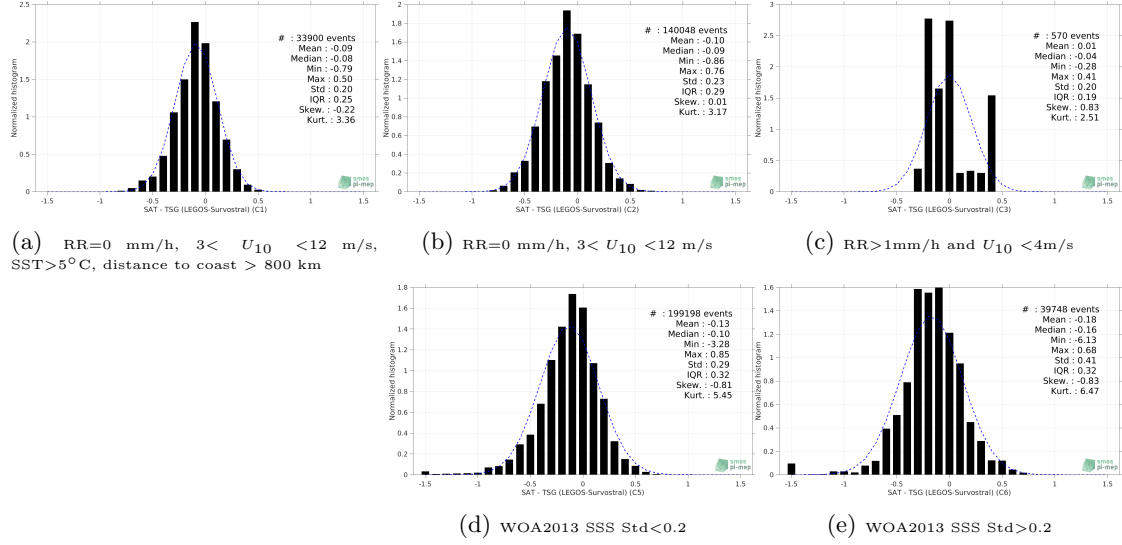
Figure 13: Normalized histogram of \Delta SSS (SMAP SSS L3 v4 - Monthly (RSS) - TSG (LEGOS-Survostral)) for 5 different subdatasets corresponding to: RR=0 mm/h, 3 < U_{10} < 12 m/s, SST>5°C, distance to coast > 800 km (a), RR=0 mm/h, 3 < U_{10} < 12 m/s (b), RR>1mm/h and U_{10} < 4 m/s (c), WOA2013 SSS Std<0.2 (d), WOA2013 SSS Std>0.2 (e).
