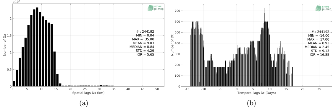
Figure 5: Histograms of the spatial (a) and temporal (b) lags between the location/time of the TSG (LEGOS-Survostral) measurement and the date of the corresponding SMAP SSS L3 v4 - Monthly (RSS) SSS pixel.
