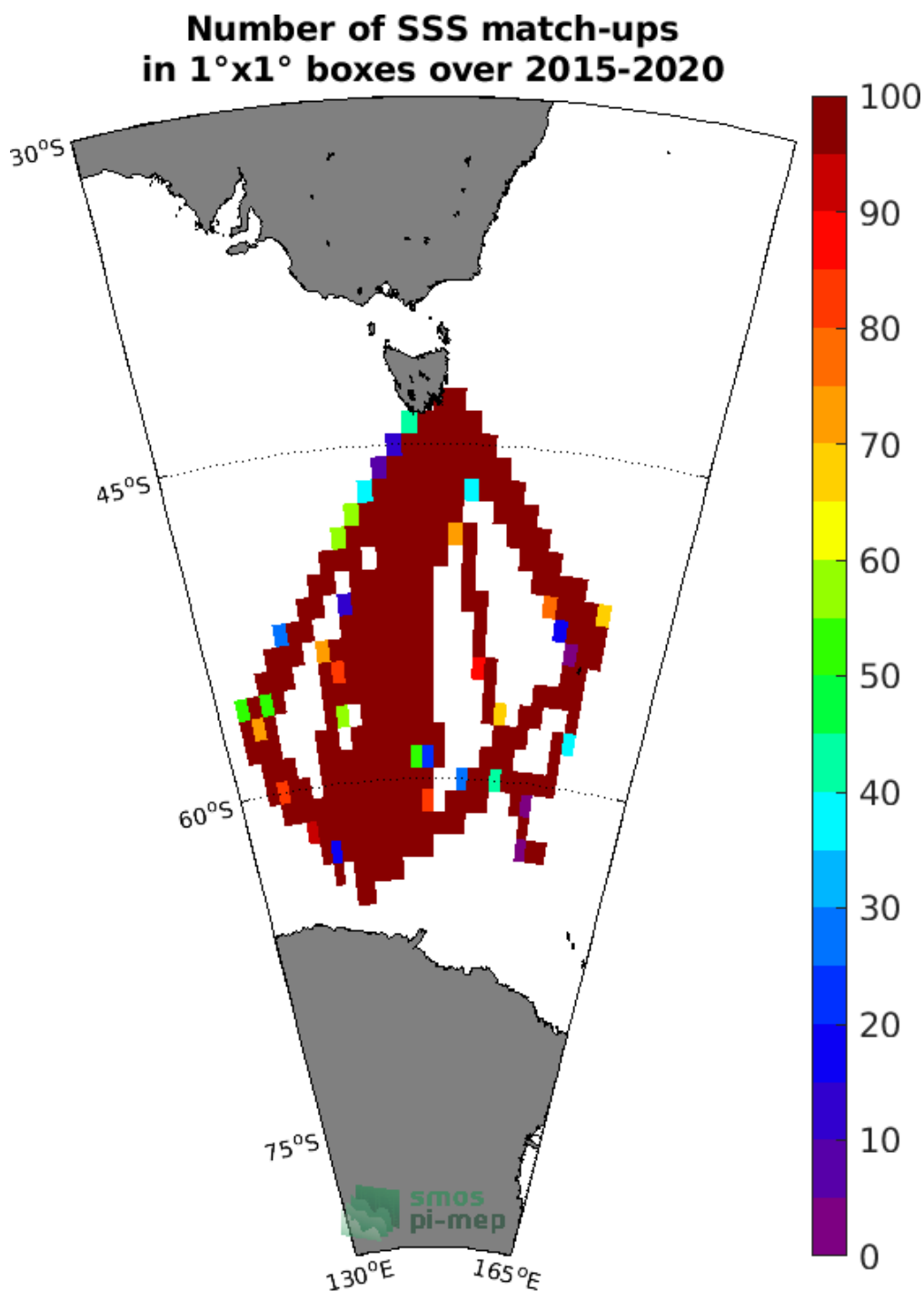
Figure 4: Number of SSS match-ups between TSG (LEGOS-Survostral) SSS and the SMAP SSS L3 v4 - Monthly (RSS) SSS product for the Global Ocean Pi-MEP region over 1°x1° boxes and for the full satellite product period.
