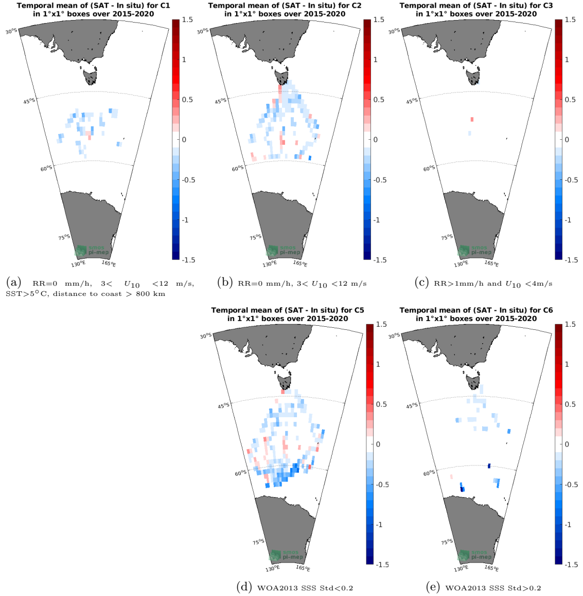
Figure 12: Temporal mean gridded over spatial boxes of size 1^\circ \times 1^\circ of \Delta\text{SSS} (SMAP SSS L3 v4 - Monthly (RSS) - TSG (LEGOS-Survostral)) for 5 different subdatasets corresponding to: RR=0 mm/h, 3 < U_{10} < 12 m/s, SST > 5^\circ\text{C} , distance to coast > 800 km (a), RR=0 mm/h, 3 < U_{10} < 12 m/s (b), RR > 1 mm/h and U_{10} < 4 m/s (c), WOA2013 SSS Std < 0.2 (d), WOA2013 SSS Std > 0.2 (e).
