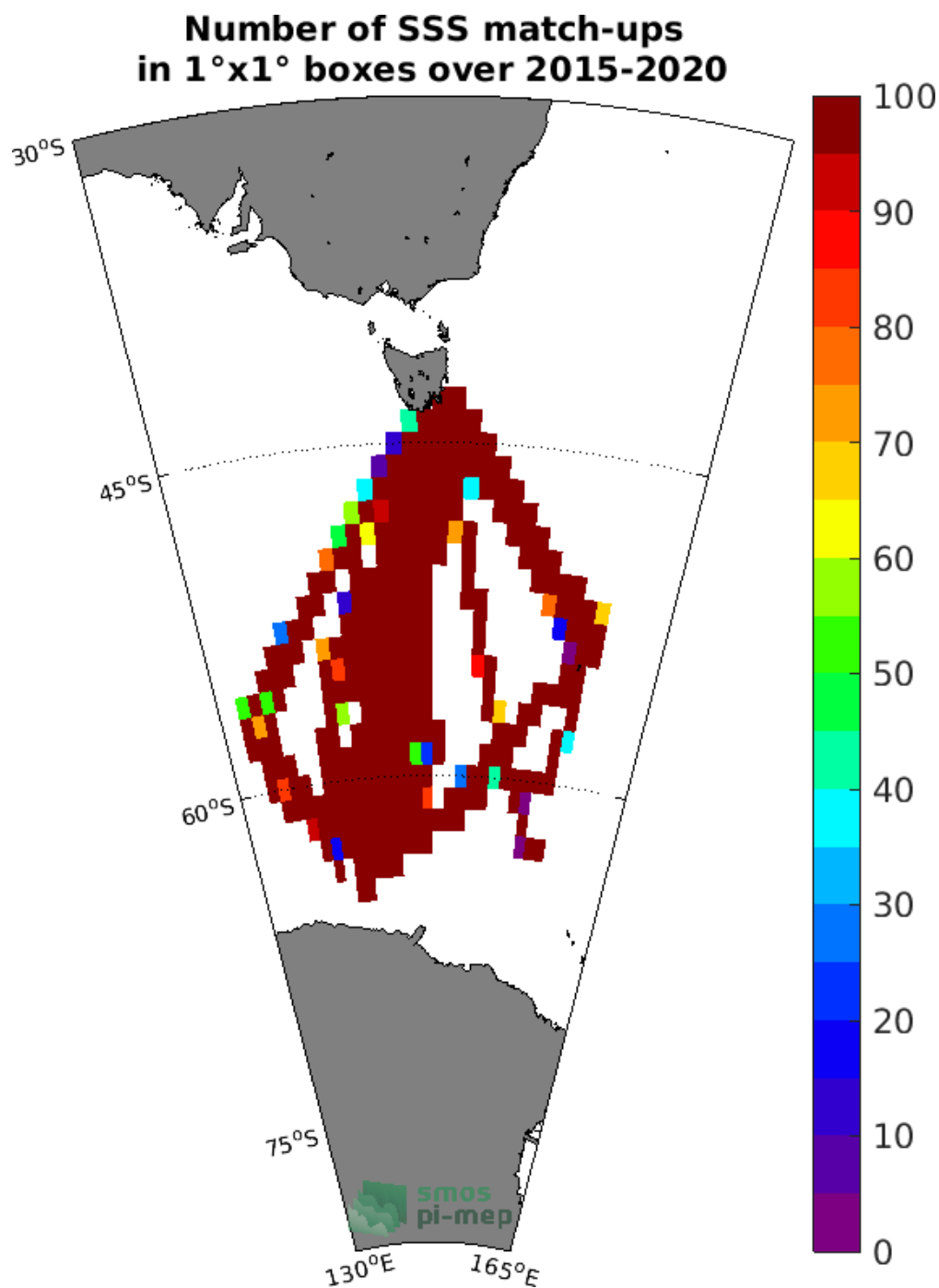
Figure 4: Number of SSS match-ups between TSG (LEGOS-Survostral) SSS and the SMAP SSS L3 v4 - Monthly (RSS) SSS product for the Global Ocean Pi-MEP region over 1°x1° boxes and for the full satellite product period.
