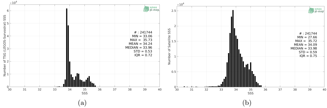
Figure 2: Histograms of SSS from TSG (LEGOS-Survostral) (a) and SMAP SSS L3 v4 - Monthly (RSS) (b) considering all match-up pairs per bins of 0.1 over the Global Ocean Pi-MEP region and for the full satellite product period.
