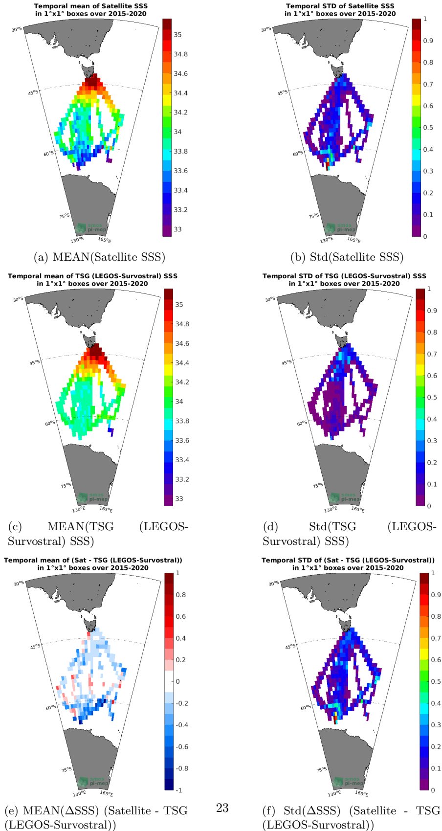
Figure 6: Temporal mean (left) and Std (right) of SSS from SMAP SSS L3 v4 - Monthly (RSS) (top), TSG (LEGOS-Survostral) (middle), and of \Delta SSS (Satellite - TSG (LEGOS-Survostral)). Only match-up pairs are used to generate these maps.
