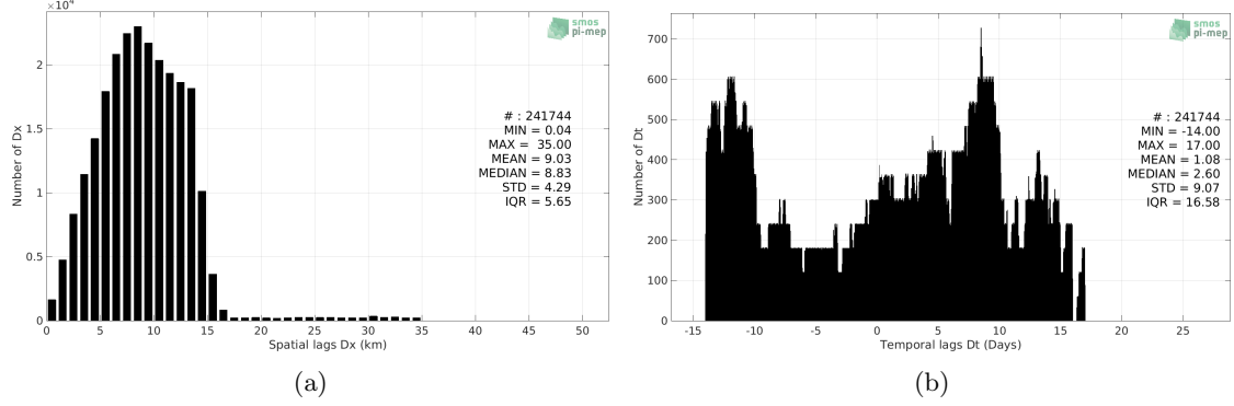
Figure 5: Histograms of the spatial (a) and temporal (b) lags between the time of the TSG (LEGOS-Survostral) measurements and the date of the corresponding SMAP SSS L3 v4 - Monthly (RSS) SSS product.
