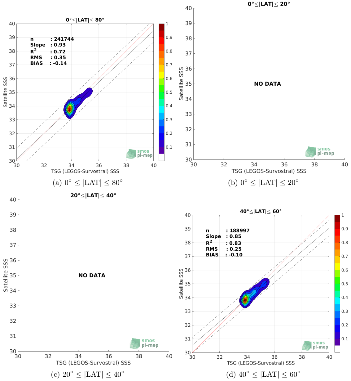
Figure 9: Contour maps of the concentration of SMAP SSS L3 v4 - Monthly (RSS) SSS (y-axis) versus TSG (LEGOS-Survostral) SSS (x-axis) at match-up pairs for different latitude bands. For each plot, the red line shows x=y . The black thin and dashed lines indicate a linear fit through the data cloud and the \pm 95\% confidence levels, respectively. The number match-up pairs n , the slope and R^2 coefficient of the linear fit, the root mean square (RMS) and the mean bias between satellite and in situ data are indicated for each latitude band in each plots.
