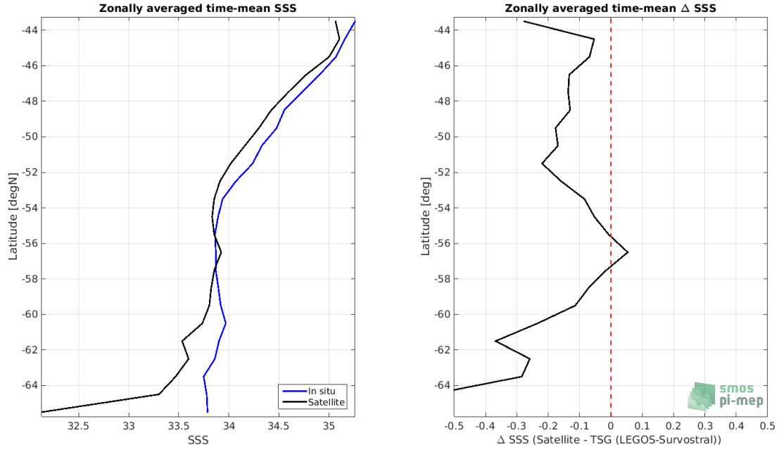
Figure 8: Left panel: Zonal mean SSS from SMAP SSS L3 v4 - Monthly (RSS) satellite product (black) and from TSG (LEGOS-Survostral) (blue). Right panel: Zonal mean of \Delta SSS (Satellite - TSG (LEGOS-Survostral)) for all the collected Pi-MEP match-up pairs estimated over the full satellite product period.
