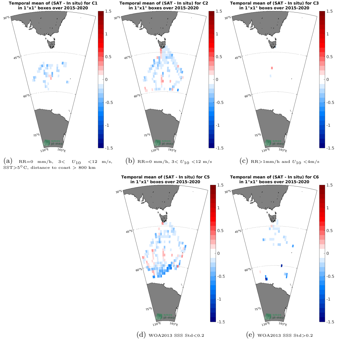
Figure 12: Temporal mean gridded over spatial boxes of size 1°x1° of \Delta\text{SSS} (SMAP SSS L3 v4 - Monthly (RSS) - TSG (LEGOS-Survostral)) for 5 different subdatasets corresponding to: RR=0 mm/h, 3 < U_{10} < 12 m/s, SST > 5^\circ\text{C} , distance to coast > 800 km (a), RR=0 mm/h, 3 < U_{10} < 12 m/s (b), RR > 1 mm/h and U_{10} < 4 m/s (c), WOA2013 SSS Std < 0.2 (d), WOA2013 SSS Std > 0.2 (e).
