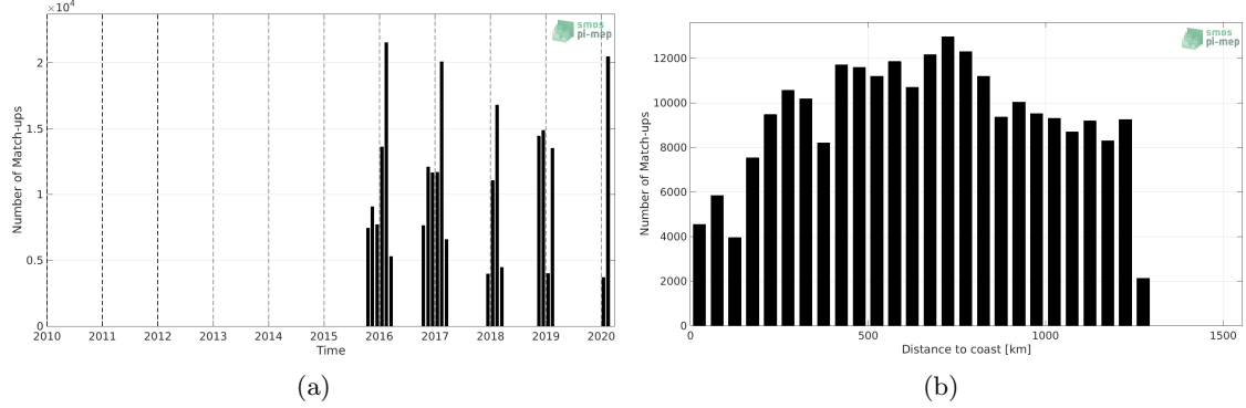
Figure 1: Number of match-ups between TSG (LEGOS-Survostral) and SMAP SSS L3 v4 - Monthly (RSS) SSS as a function of time (a) and as function of the distance to coast (b) over the Global Ocean Pi-MEP region and for the full satellite product period.
