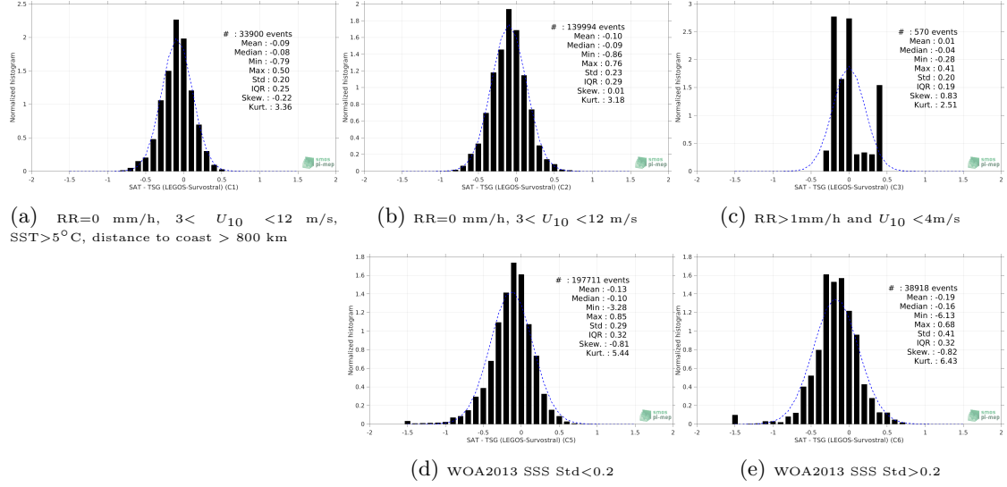
Figure 13: Normalized histogram of \Delta SSS (SMAP SSS L3 v4 - Monthly (RSS) - TSG (LEGOS-Survostral)) for 5 different subdatasets corresponding to: RR=0 mm/h, 3 < U_{10} < 12 m/s, SST>5°C, distance to coast > 800 km (a), RR=0 mm/h, 3 < U_{10} < 12 m/s (b), RR>1mm/h and U_{10} < 4 m/s (c), WOA2013 SSS Std<0.2 (d), WOA2013 SSS Std>0.2 (e).
