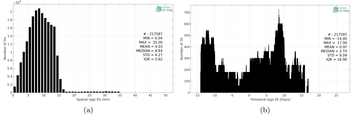
Figure 5: Histograms of the spatial (a) and temporal (b) lags between the time of the TSG-LEGOS-Survostral measurements and the date of the corresponding SMAP-L3-RSS-V4-MONTHLY SSS product.
