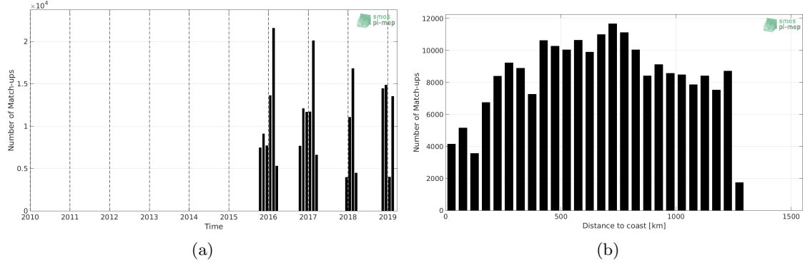
Figure 1: Number of match-ups between TSG-LEGOS-Survostral and SMAP-L3-RSS-V4-MONTHLY SSS as a function of time (a) and as function of the distance to coast (b) over the Global Ocean Pi-MEP region and for the full satellite product period.
