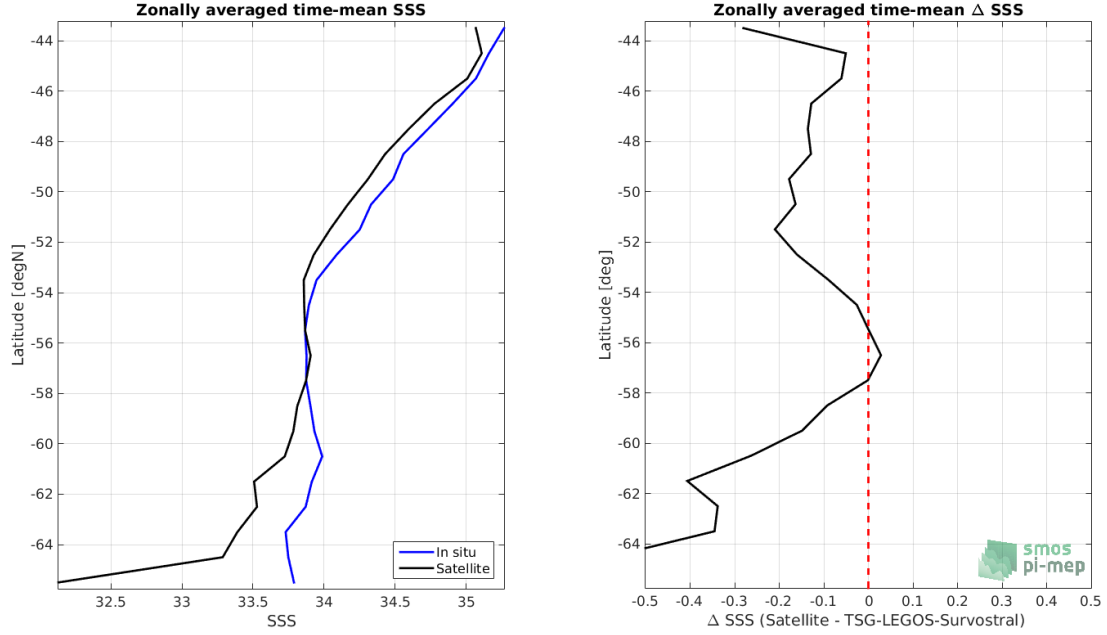
Figure 8: Left panel: Zonal mean SSS from SMAP-L3-RSS-V4-MONTHLY satellite product (black) and from TSG-LEGOS-Survostral (blue). Right panel: Zonal mean of \Delta SSS (Satellite - TSG-LEGOS-Survostral) for all the collected Pi-MEP match-up pairs estimated over the full satellite product period.
