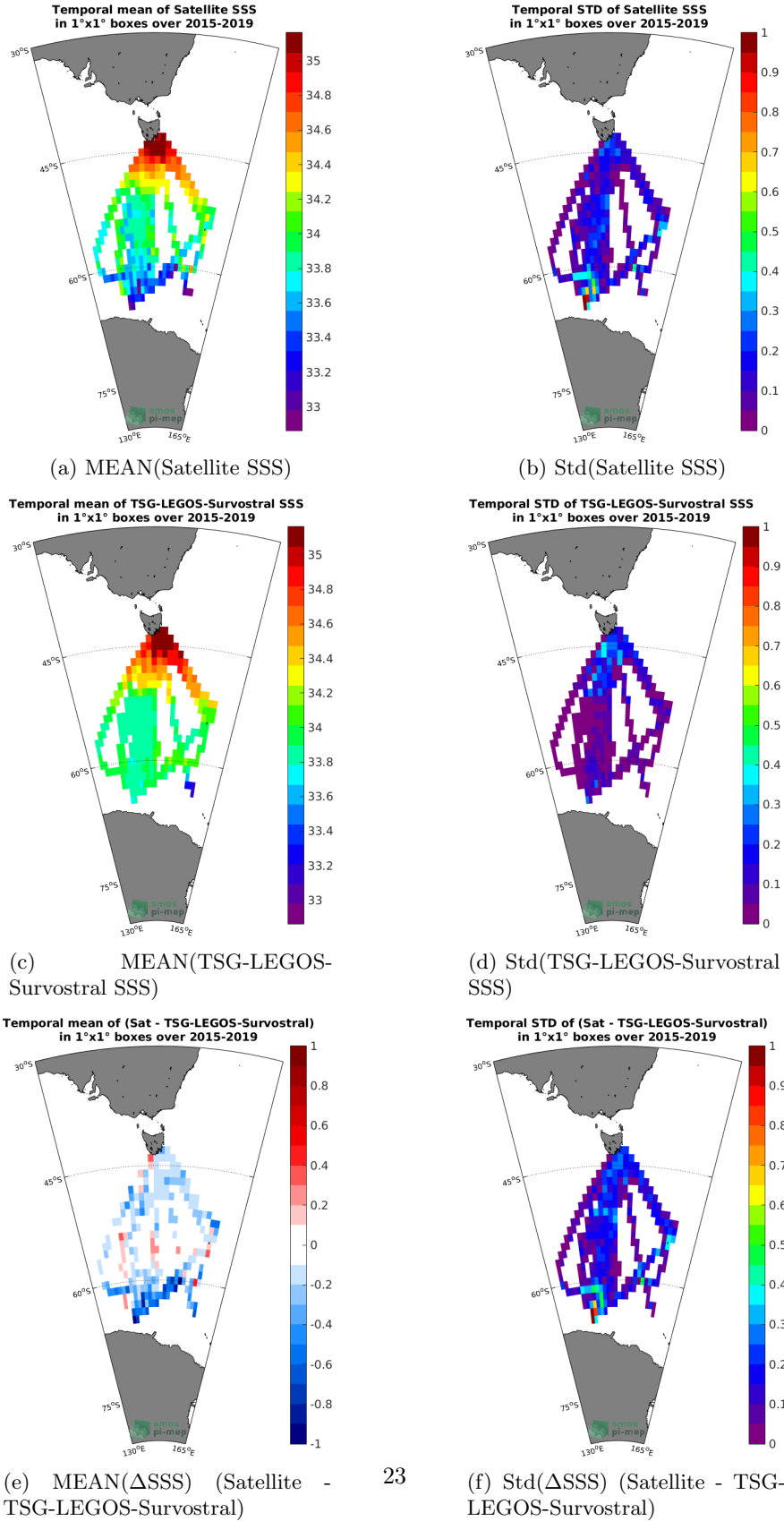
Figure 6: Temporal mean (left) and Std (right) of SSS from SMAP-L3-RSS-V4-MONTHLY (top), TSG-LEGOS-Survostral (middle), and of \Delta SSS (Satellite - TSG-LEGOS-Survostral). Only match-up pairs are used to generate these maps.
