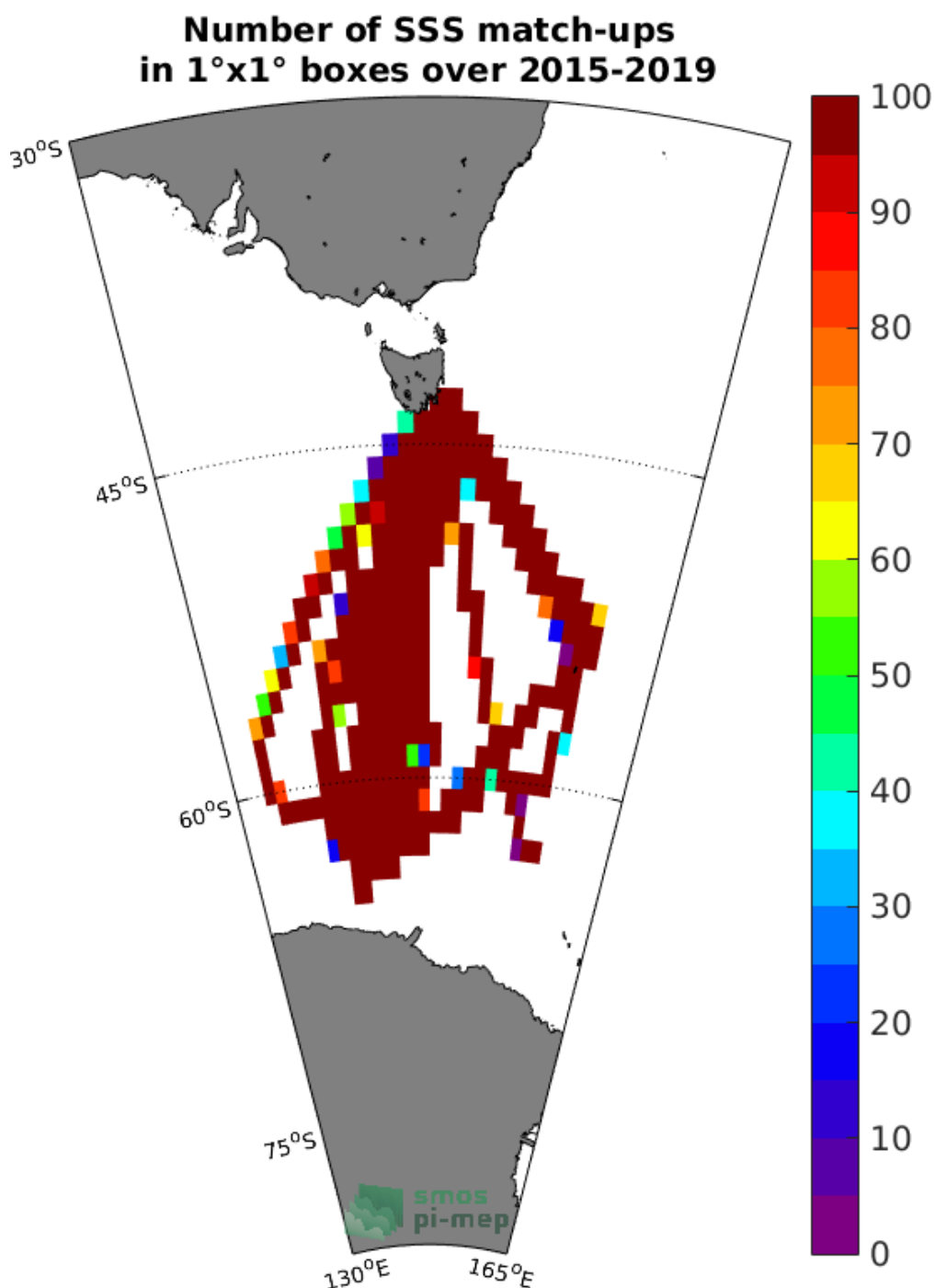
Figure 4: Number of SSS match-ups between TSG-LEGOS-Survostral SSS and the SMAP-L3-RSS-V4-MONTHLY SSS product for the Global Ocean Pi-MEP region over 1°x1° boxes and for the full satellite product period.
