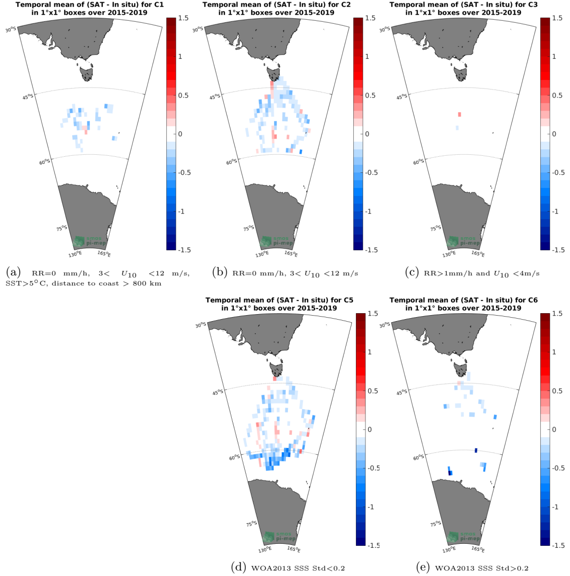
Figure 12: Temporal mean gridded over spatial boxes of size 1°x1° of \Delta\text{SSS} (SMAP-L3-RSS-V4-MONTHLY - TSG-LEGOS-Survostral) for 5 different subdatasets corresponding to: RR=0 mm/h, 3 < U_{10} < 12 m/s, SST > 5^\circ\text{C} , distance to coast > 800 km (a), RR=0 mm/h, 3 < U_{10} < 12 m/s (b), RR > 1\text{mm/h} and U_{10} < 4\text{m/s} (c), WOA2013 SSS Std < 0.2 (d), WOA2013 SSS Std > 0.2 (e).
