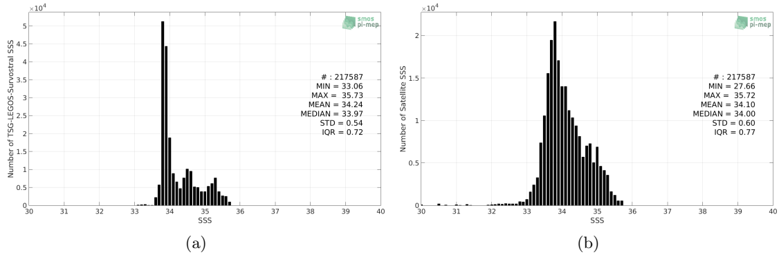
Figure 2: Histograms of SSS from TSG-LEGOS-Survostral (a) and SMAP-L3-RSS-V4-MONTHLY (b) considering all match-up pairs per bins of 0.1 over the Global Ocean Pi-MEP region and for the full satellite product period.
