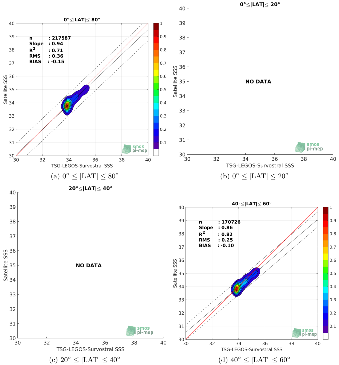
Figure 9: Contour maps of the concentration of SMAP-L3-RSS-V4-MONTHLY SSS (y-axis) versus TSG-LEGOS-Survostral SSS (x-axis) at match-up pairs for different latitude bands. For each plot, the red line shows x=y . The black thin and dashed lines indicate a linear fit through the cloud and the \pm 95\% confidence levels, respectively. The number match-up pairs n , the slope and R^2 coefficient of the linear fit, the root mean square (RMS) and the mean bias between satellite and in situ data are indicated for each latitude band in each plots.
