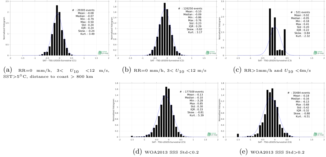
Figure 13: Normalized histogram of \Delta SSS (SMAP-L3-RSS-V4-MONTHLY - TSG-LEGOS-Survostral) for 5 different subdatasets corresponding to: RR=0 mm/h, 3 < U_{10} < 12 m/s, SST>5°C, distance to coast > 800 km (a), RR=0 mm/h, 3 < U_{10} < 12 m/s (b), RR>1mm/h and U_{10} < 4 m/s (c), WOA2013 SSS Std<0.2 (d), WOA2013 SSS Std>0.2 (e).
