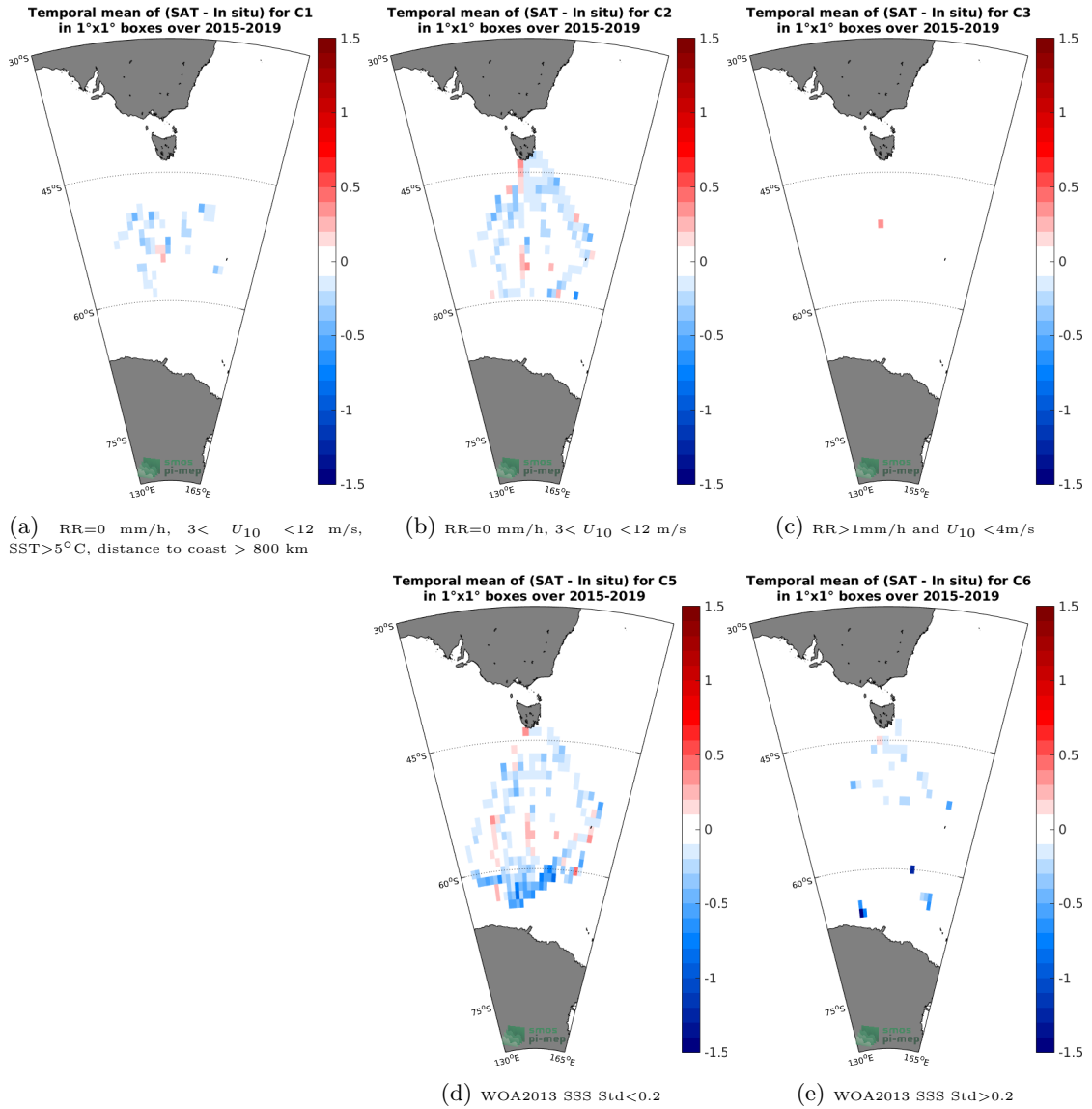
Figure 12: Temporal mean gridded over spatial boxes of size 1°x1° of \Delta SSS (SMAP-L3-RSS-V4-MONTHLY - TSG-LEGOS-Survostral) for 5 different subdatasets corresponding to:RR=0 mm/h, 3 < U_{10} < 12 m/s, SST > 5°C, distance to coast > 800 km (a), RR=0 mm/h, 3 < U_{10} < 12 m/s (b), RR > 1mm/h and U_{10} < 4 m/s (c), WOA2013 SSS Std < 0.2 (d), WOA2013 SSS Std > 0.2 (e).
