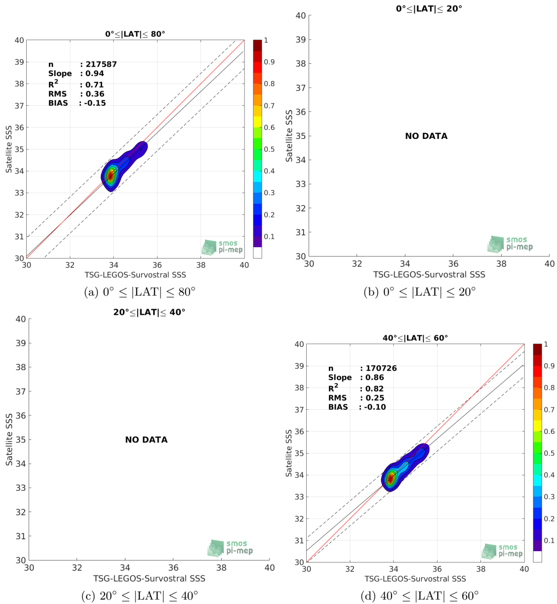
Figure 9: Contour maps of the concentration of SMAP-L3-RSS-V4-MONTHLY SSS (y-axis) versus TSG-LEGOS-Survostral SSS (x-axis) at match-up pairs for different latitude bands. For each plot, the red line shows x=y . The black thin and dashed lines indicate a linear fit through the data cloud and the \pm 95\% confidence levels, respectively. The number match-up pairs n , the slope and R^2 coefficient of the linear fit, the root mean square (RMS) and the mean bias between satellite and in situ data are indicated for each latitude band in each plots.
