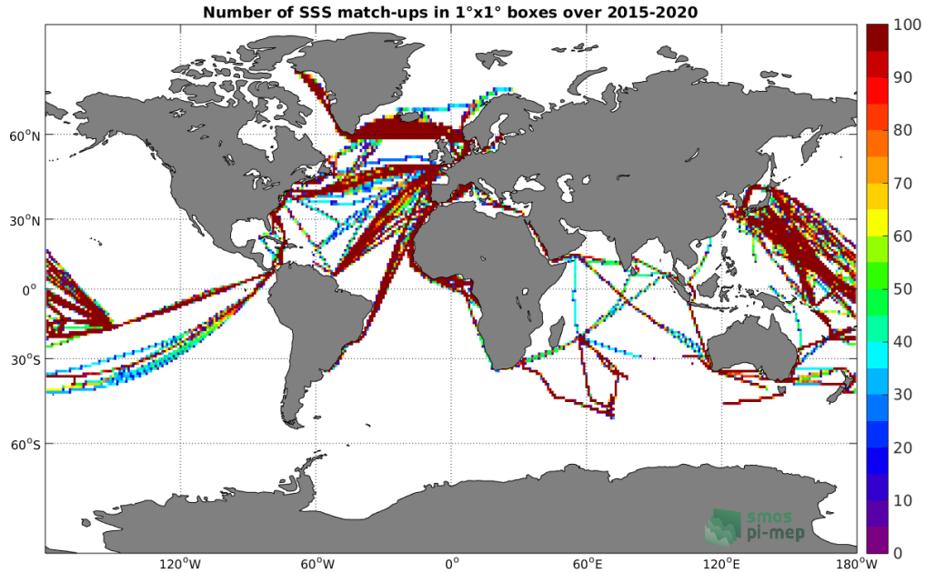
Figure 4: Number of SSS match-ups between TSG (LEGOS-DM) SSS and the SMAP SSS L3 v4 - Monthly (RSS) SSS product for the Global Ocean Pi-MEP region over 1^\circ \times 1^\circ boxes and for the full satellite product period.
