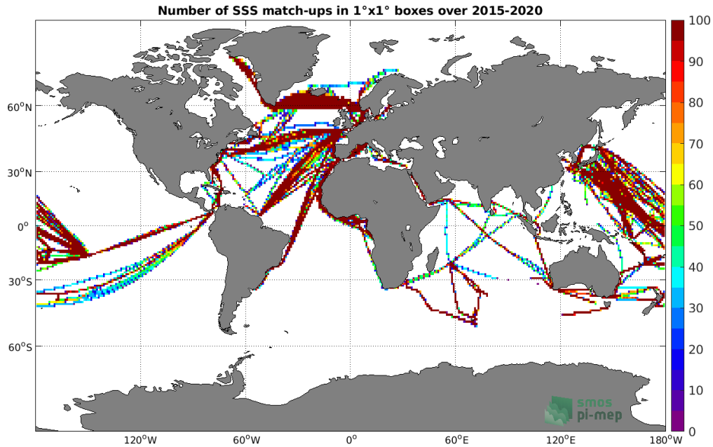
Figure 4: Number of SSS match-ups between TSG (LEGOS-DM) SSS and the SMAP SSS L3 v4 - Monthly (RSS) SSS product for the Global Ocean Pi-MEP region over 1^\circ \times 1^\circ boxes and for the full satellite product period.
