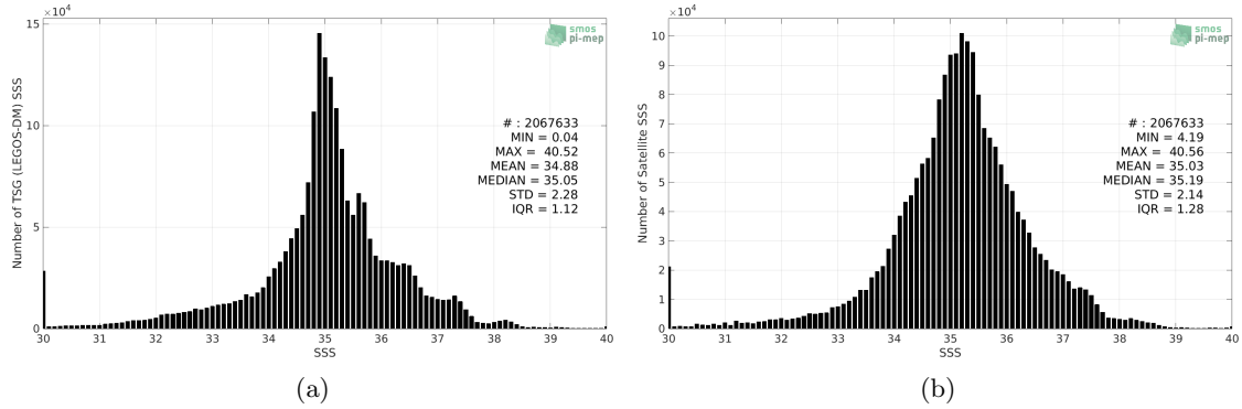
Figure 2: Histograms of SSS from TSG (LEGOS-DM) (a) and SMAP SSS L3 v4 - Monthly (RSS) (b) considering all match-up pairs per bins of 0.1 over the Global Ocean Pi-MEP region and for the full satellite product period.
