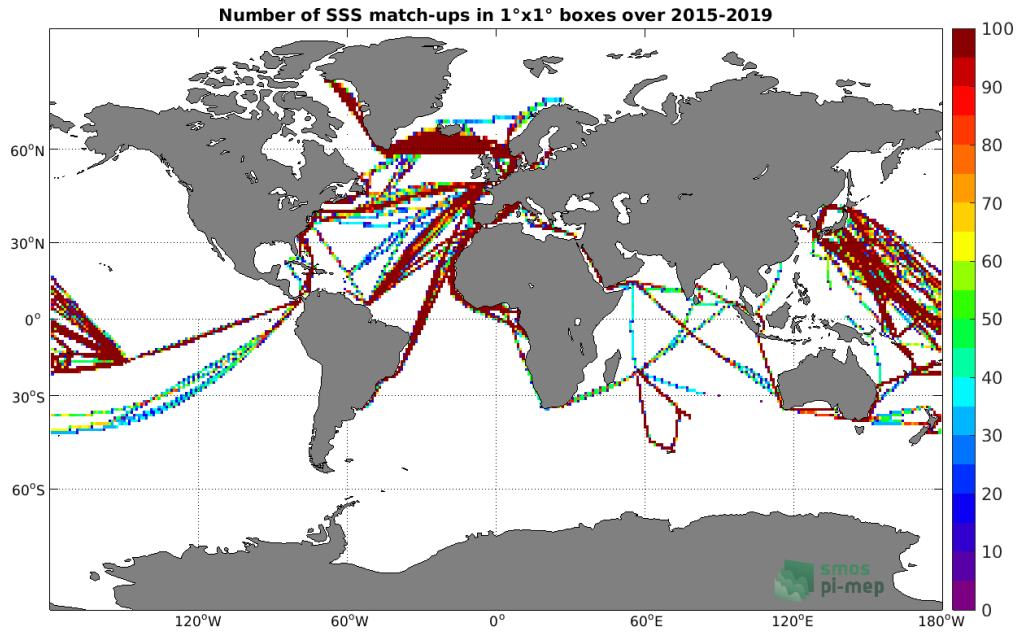
Figure 4: Number of SSS match-ups between TSG (LEGOS-DM) SSS and the SMAP SSS L3 v4 - Monthly (RSS) SSS product for the Global Ocean Pi-MEP region over 1°x1° boxes and for the full satellite product period.
