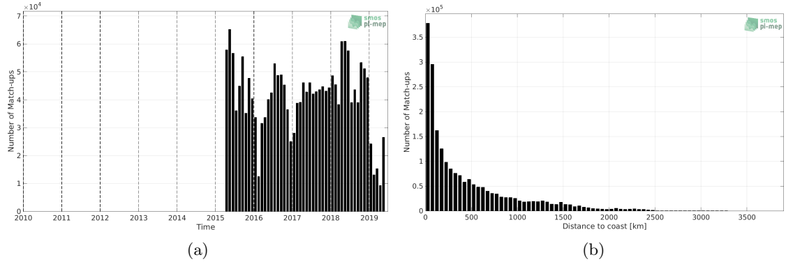
Figure 1: Number of match-ups between TSG (LEGOS-DM) and SMAP SSS L3 v4 - Monthly (RSS) SSS as a function of time (a) and as function of the distance to coast (b) over the Global Ocean Pi-MEP region and for the full satellite product period.
