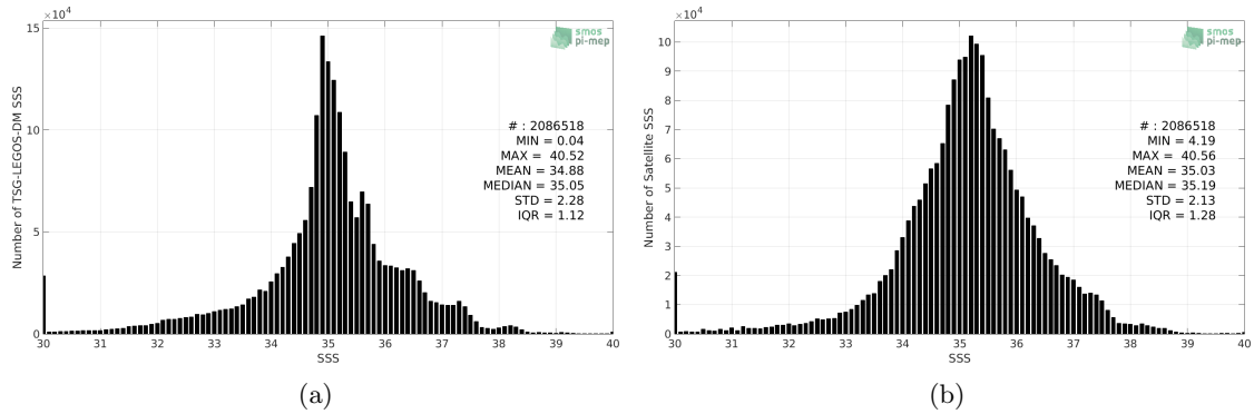
Figure 2: Histograms of SSS from TSG-LEGOS-DM (a) and SMAP-L3-RSS-V4-MONTHLY (b) considering all match-up pairs per bins of 0.1 over the Global Ocean Pi-MEP region and for the full satellite product period.
