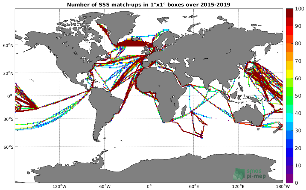
Figure 4: Number of SSS match-ups between TSG-LEGOS-DM SSS and the SMAP-L3-RSS-V4-MONTHLY SSS product for the Global Ocean Pi-MEP region over 1°x1° boxes and for the full satellite product period.
