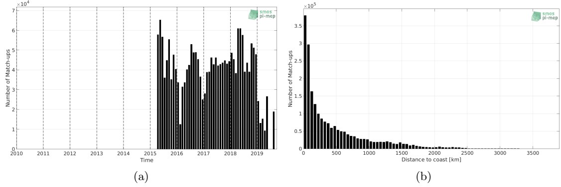
Figure 1: Number of match-ups between TSG-LEGOS-DM and SMAP-L3-RSS-V4-MONTHLY SSS as a function of time (a) and as function of the distance to coast (b) over the Global Ocean Pi-MEP region and for the full satellite product period.
