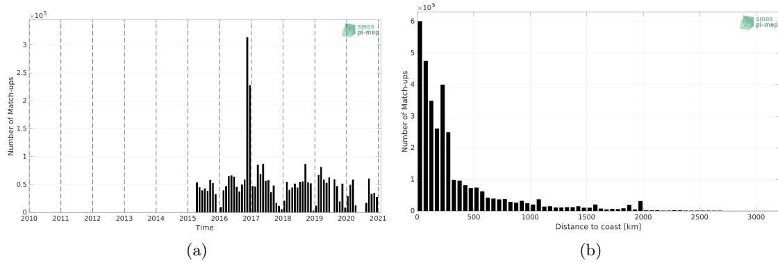
Figure 1: Number of match-ups between TSG (GOSUD-Research-vessel) and SMAP SSS L3 v4 - Monthly (RSS) SSS as a function of time (a) and as function of the distance to coast (b) over the Global Ocean Pi-MEP region and for the full satellite product period.
