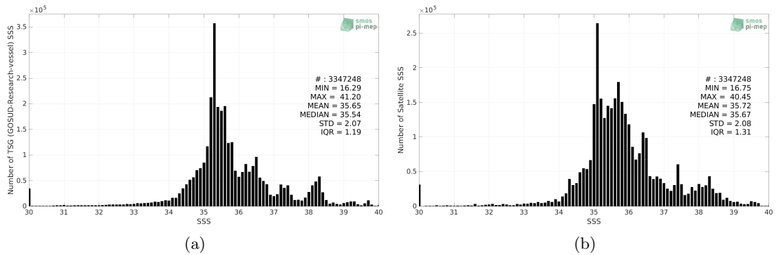
Figure 2: Histograms of SSS from TSG (GOSUD-Research-vessel) (a) and SMAP SSS L3 v4 - Monthly (RSS) (b) considering all match-up pairs per bins of 0.1 over the Global Ocean Pi-MEP region and for the full satellite product period.
