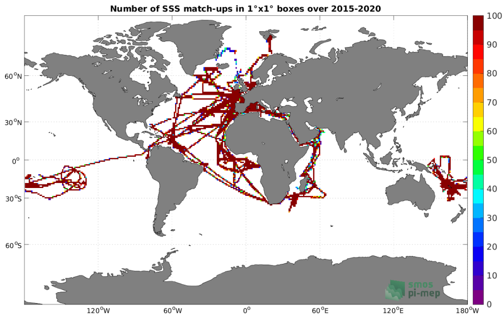
Figure 4: Number of SSS match-ups between TSG (GOSUD-Research-vessel) SSS and the SMAP SSS L3 v4 - Monthly (RSS) SSS product for the Global Ocean Pi-MEP region over 1^\circ \times 1^\circ boxes and for the full satellite product period.
