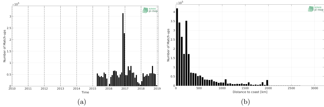
Figure 1: Number of match-ups between TSG-GOSUD-Research-vessel and SMAP-L3-RSS-V4-MONTHLY SSS as a function of time (a) and as function of the distance to coast (b) over the Global Ocean Pi-MEP region and for the full satellite product period.
