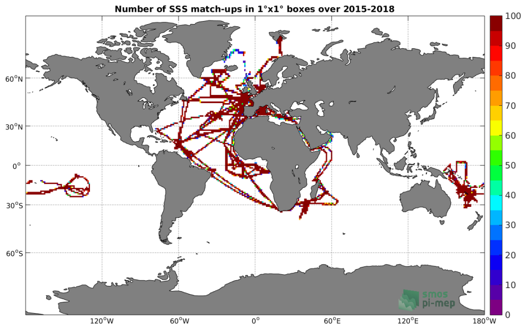
Figure 4: Number of SSS match-ups between TSG-GOSUD-Research-vessel SSS and the SMAP-L3-RSS-V4-MONTHLY SSS product for the Global Ocean Pi-MEP region over 1^\circ \times 1^\circ boxes and for the full satellite product period.
