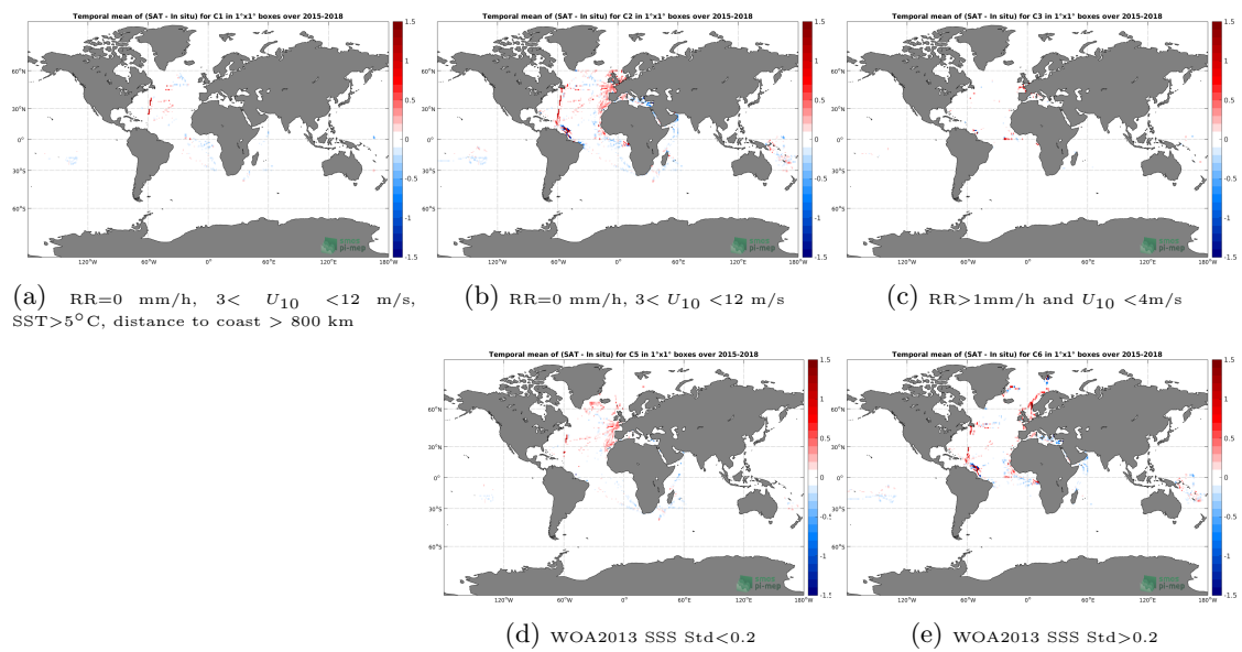
Figure 12: Temporal mean gridded over spatial boxes of size 1^\circ \times 1^\circ of \Delta SSS (SMAP-L3-RSS-V4-MONTHLY - TSG-GOSUD-Research-vessel) for 5 different subdatasets corresponding to:RR=0 mm/h, 3 < U_{10} < 12 m/s, SST > 5^\circ\text{C} , distance to coast > 800 km (a), RR=0 mm/h, 3 < U_{10} < 12 m/s (b), RR > 1 mm/h and U_{10} < 4 m/s (c), WOA2013 SSS Std < 0.2 (d), WOA2013 SSS Std > 0.2 (e).
