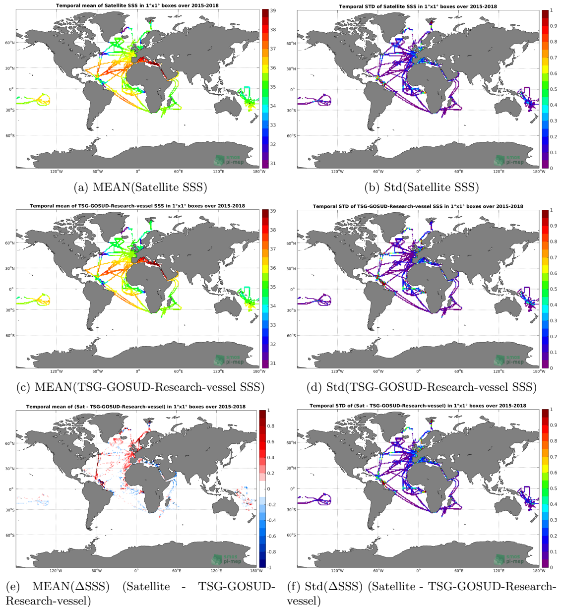
Figure 6: Temporal mean (left) and Std (right) of SSS from SMAP-L3-RSS-V4-MONTHLY (top), TSG-GOSUD-Research-vessel (middle), and of \Delta SSS (Satellite - TSG-GOSUD-Research-vessel). Only match-up pairs are used to generate these maps.
