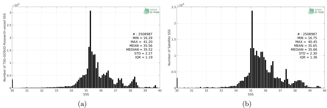
Figure 2: Histograms of SSS from TSG-GOSUD-Research-vessel (a) and SMAP-L3-RSS-V4-MONTHLY (b) considering all match-up pairs per bins of 0.1 over the Global Ocean Pi-MEP region and for the full satellite product period.
