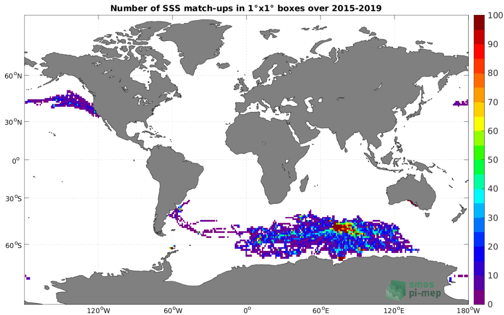
Figure 4: Number of SSS match-ups between Marine mammals SSS and the SMAP SSS L3 v4 - Monthly (RSS) SSS product for the Global Ocean Pi-MEP region over 1^\circ \times 1^\circ boxes and for the full satellite product period.
