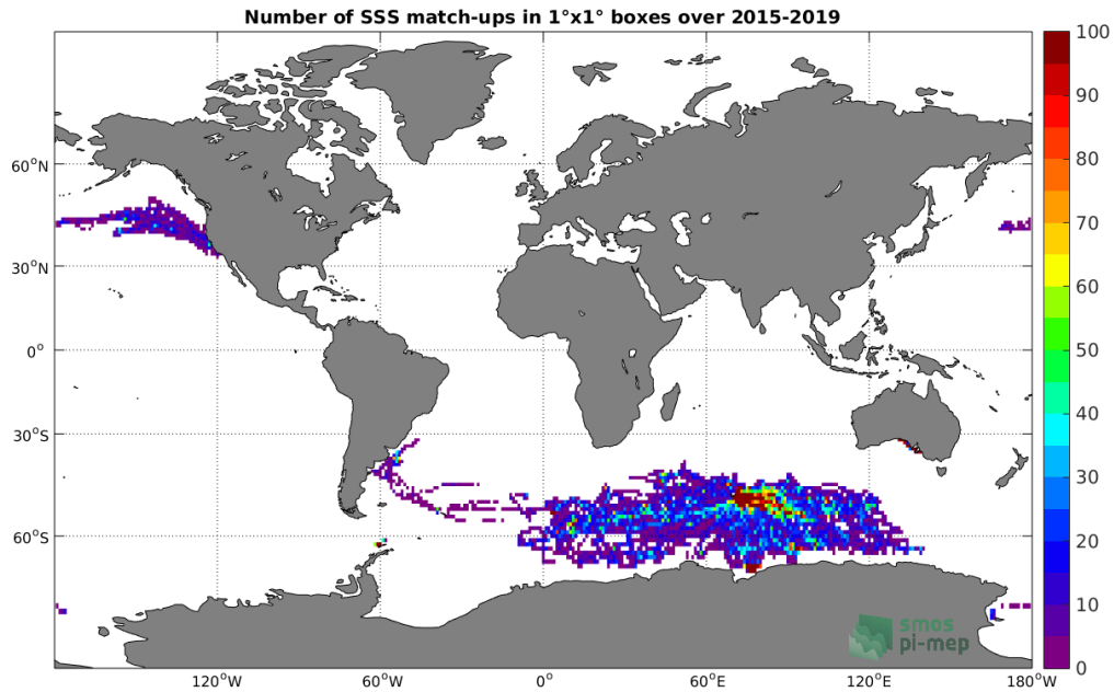
Figure 4: Number of SSS match-ups between Marine mammals SSS and the SMAP SSS L3 v4 - Monthly (RSS) SSS product for the Global Ocean Pi-MEP region over 1^\circ \times 1^\circ boxes and for the full satellite product period.
