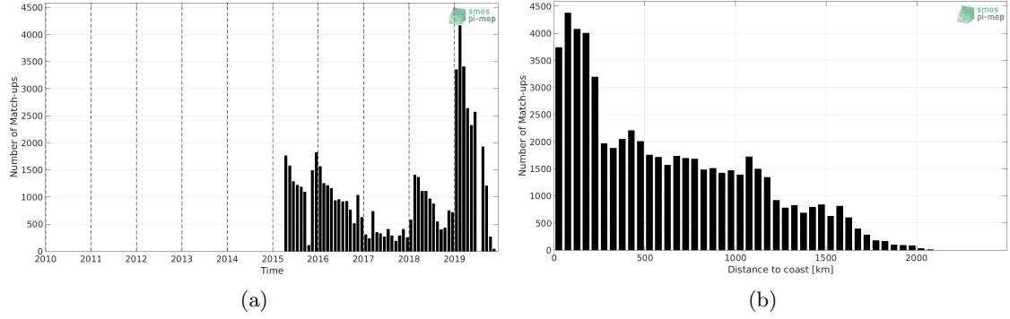
Figure 1: Number of match-ups between Marine mammals and SMAP SSS L3 v4 - Monthly (RSS) SSS as a function of time (a) and as function of the distance to coast (b) over the Global Ocean Pi-MEP region and for the full satellite product period.
