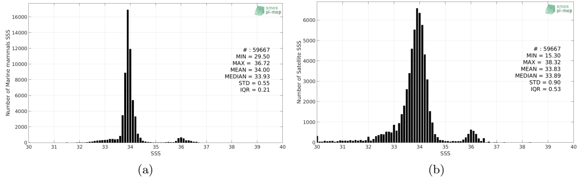
Figure 2: Histograms of SSS from Marine mammals (a) and SMAP SSS L3 v4 - Monthly (RSS) (b) considering all match-up pairs per bins of 0.1 over the Global Ocean Pi-MEP region and for the full satellite product period.
