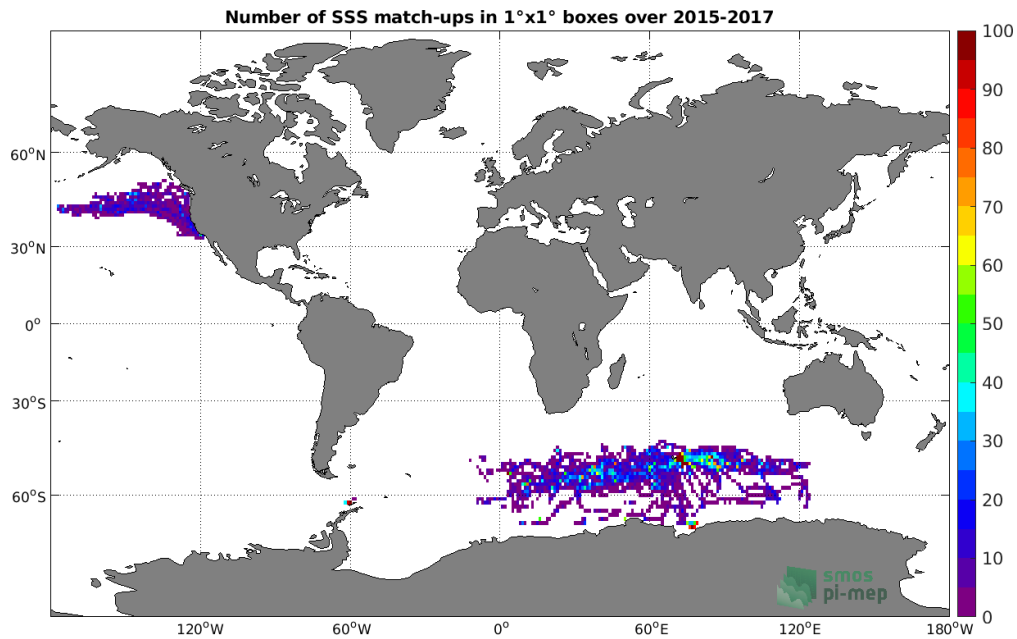
Figure 4: Number of SSS match-ups between Sea mammals SSS and the SMAP SSS L3 v4 - Monthly (RSS) SSS product for the Global Ocean Pi-MEP region over 1^\circ \times 1^\circ boxes and for the full satellite product period.
