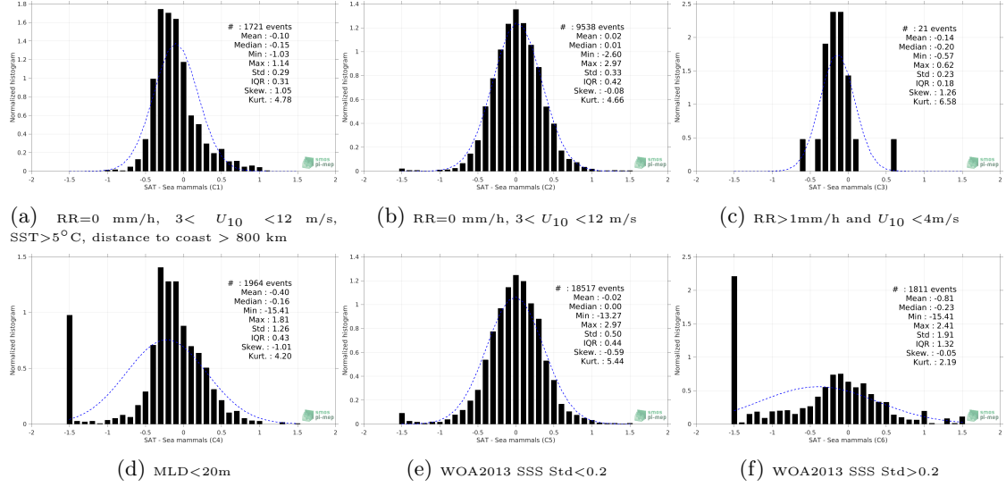
Figure 13: Normalized histogram of \Delta SSS (SMAP SSS L3 v4 - Monthly (RSS) - Sea mammals) for 6 different subdatasets corresponding to: RR=0 mm/h, 3 < U_{10} < 12 m/s, SST>5°C, distance to coast > 800 km (a), RR=0 mm/h, 3 < U_{10} < 12 m/s (b), RR>1mm/h and U_{10} < 4 m/s (c), MLD<20m (d), WOA2013 SSS Std<0.2 (e), WOA2013 SSS Std>0.2 (f).
