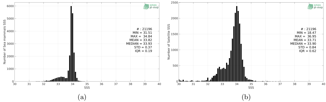
Figure 2: Histograms of SSS from Sea mammals (a) and SMAP SSS L3 v4 - Monthly (RSS) (b) considering all match-up pairs per bins of 0.1 over the Global Ocean Pi-MEP region and for the full satellite product period.
