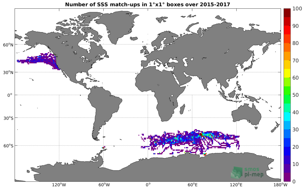
Figure 4: Number of SSS match-ups between Sea mammals SSS and the SMAP SSS L3 v4 - Monthly (RSS) SSS product for the Global Ocean Pi-MEP region over 1^\circ \times 1^\circ boxes and for the full satellite product period.
