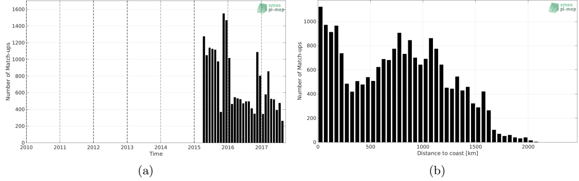
Figure 1: Number of match-ups between Sea mammals and SMAP SSS L3 v4 - Monthly (RSS) SSS as a function of time (a) and as function of the distance to coast (b) over the Global Ocean Pi-MEP region and for the full satellite product period.
