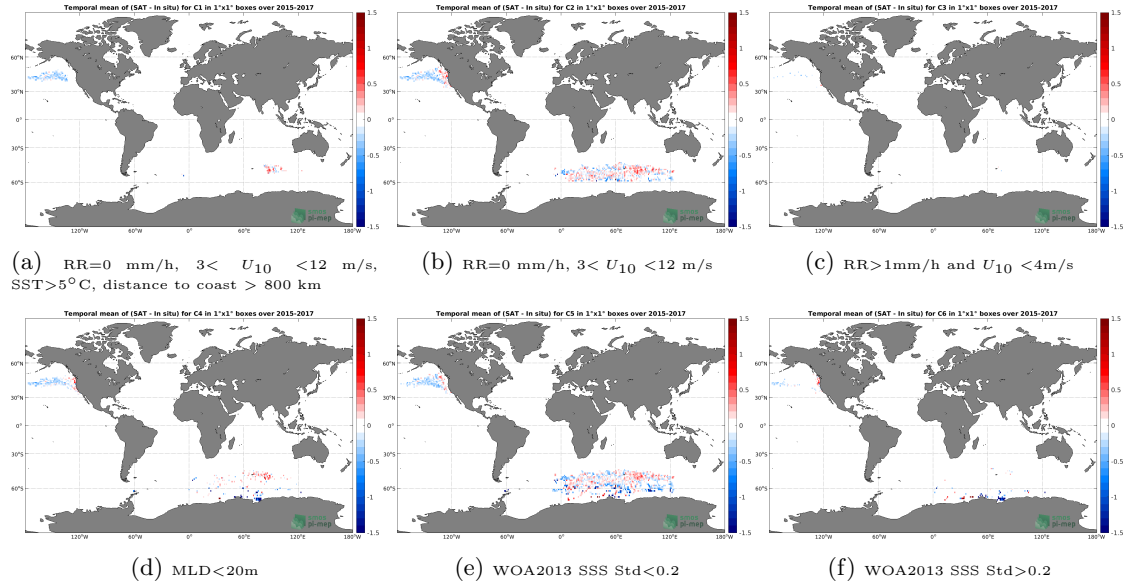
Figure 12: Temporal mean gridded over spatial boxes of size 1^\circ \times 1^\circ of \Delta SSS (SMAP SSS L3 v4 - Monthly (RSS) - Sea mammals) for 6 different subdatasets corresponding to: RR=0 mm/h, 3 < U_{10} < 12 m/s, SST >5^\circ\text{C} , distance to coast > 800 km (a), RR=0 mm/h, 3 < U_{10} < 12 m/s (b), RR >1 mm/h and U_{10} < 4 m/s (c), MLD <20 m (d), WOA2013 SSS Std <0.2 (e), WOA2013 SSS Std >0.2 (f).
