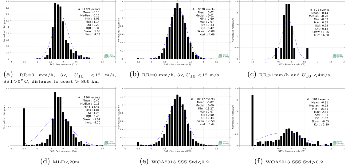
Figure 13: Normalized histogram of \Delta SSS (SMAP-L3-RSS-V4-MONTHLY - Sea mammals) for 6 different subdatasets corresponding to: RR=0 mm/h, 3 < U_{10} < 12 m/s, SST>5°C, distance to coast > 800 km (a), RR=0 mm/h, 3 < U_{10} < 12 m/s (b), RR>1mm/h and U_{10} < 4 m/s (c), MLD<20m (d), WOA2013 SSS Std<0.2 (e), WOA2013 SSS Std>0.2 (f).
