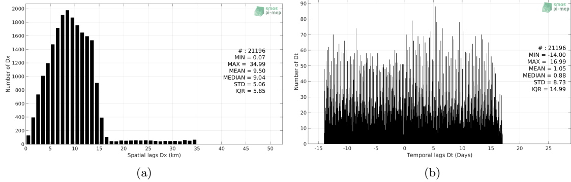
Figure 5: Histograms of the spatial (a) and temporal (b) lags between the time of the Sea mammals measurements and the date of the corresponding SMAP-L3-RSS-V4-MONTHLY SSS product.
