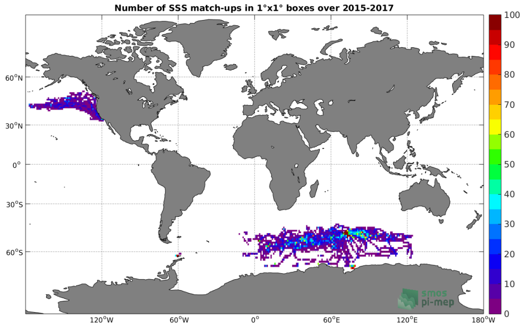
Figure 4: Number of SSS match-ups between Sea mammals SSS and the SMAP-L3-RSS-V4-MONTHLY SSS product for the Global Ocean Pi-MEP region over 1^\circ \times 1^\circ boxes and for the full satellite product period.
