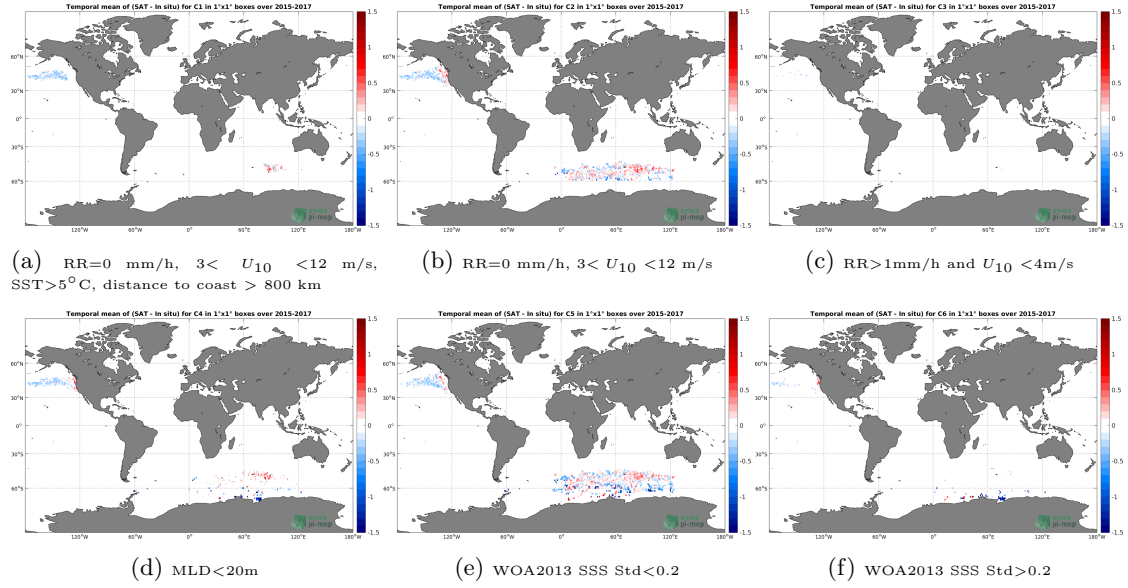
Figure 12: Temporal mean gridded over spatial boxes of size 1^\circ \times 1^\circ of \Delta SSS (SMAP-L3-RSS-V4-MONTHLY - Sea mammals) for 6 different subdatasets corresponding to: RR=0 mm/h, 3 < U_{10} < 12 m/s, SST > 5^\circ C , distance to coast > 800 km (a), RR=0 mm/h, 3 < U_{10} < 12 m/s (b), RR > 1 mm/h and U_{10} < 4 m/s (c), MLD < 20 m (d), WOA2013 SSS Std < 0.2 (e), WOA2013 SSS Std > 0.2 (f).
