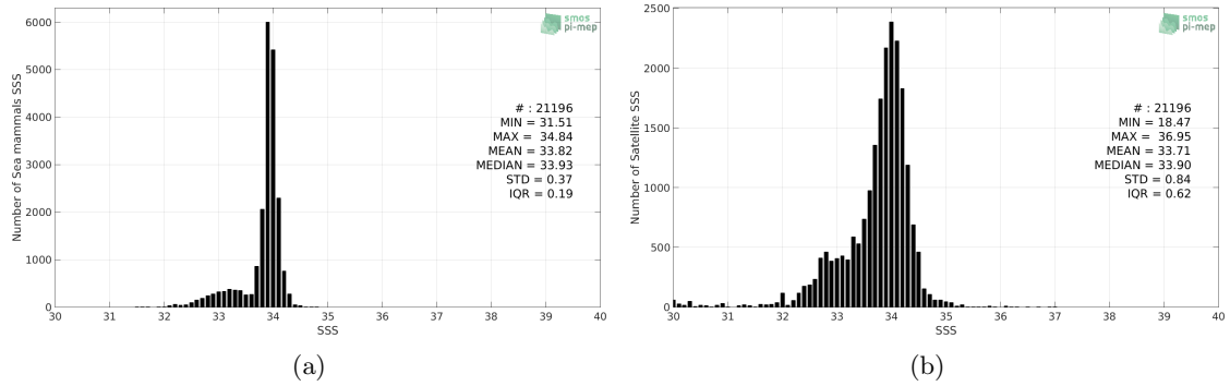
Figure 2: Histograms of SSS from Sea mammals (a) and SMAP-L3-RSS-V4-MONTHLY (b) considering all match-up pairs per bins of 0.1 over the Global Ocean Pi-MEP region and for the full satellite product period.
