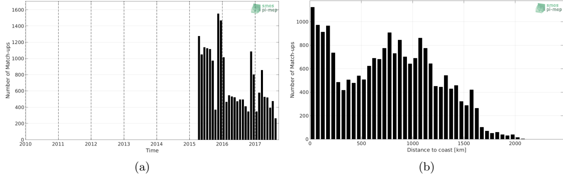
Figure 1: Number of match-ups between Sea mammals and SMAP-L3-RSS-V4-MONTHLY SSS as a function of time (a) and as function of the distance to coast (b) over the Global Ocean Pi-MEP region and for the full satellite product period.
