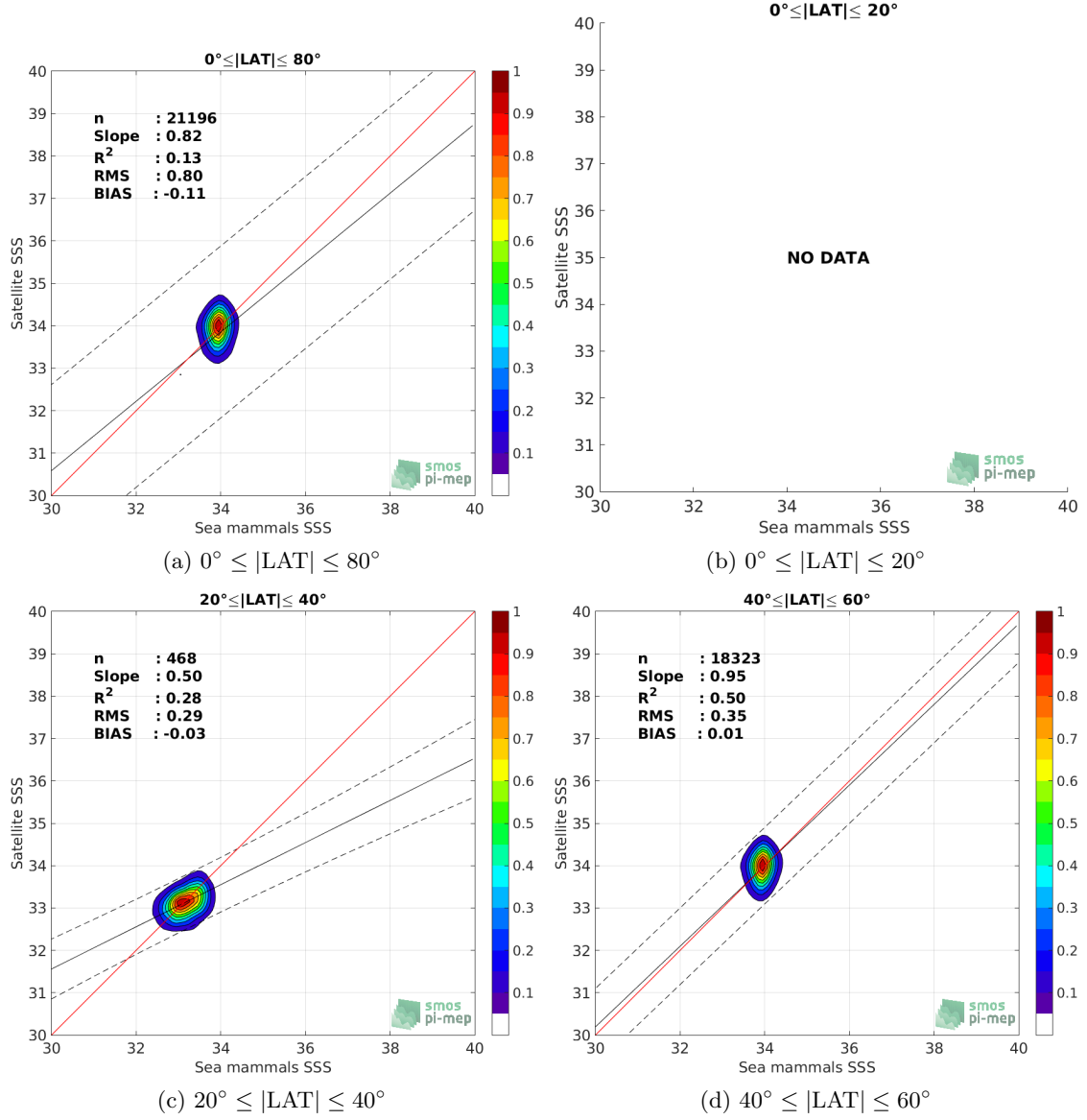
Figure 9: Contour maps of the concentration of SMAP-L3-RSS-V4-MONTHLY SSS (y-axis) versus Sea mammals SSS (x-axis) at match-up pairs for different latitude bands. For each plot, the red line shows x=y . The black thin and dashed lines indicate a linear fit through the data cloud and the \pm 95\% confidence levels, respectively. The number match-up pairs n , the slope and R^2 coefficient of the linear fit, the root mean square (RMS) and the mean bias between satellite and in situ data are indicated for each latitude band in each plots.
