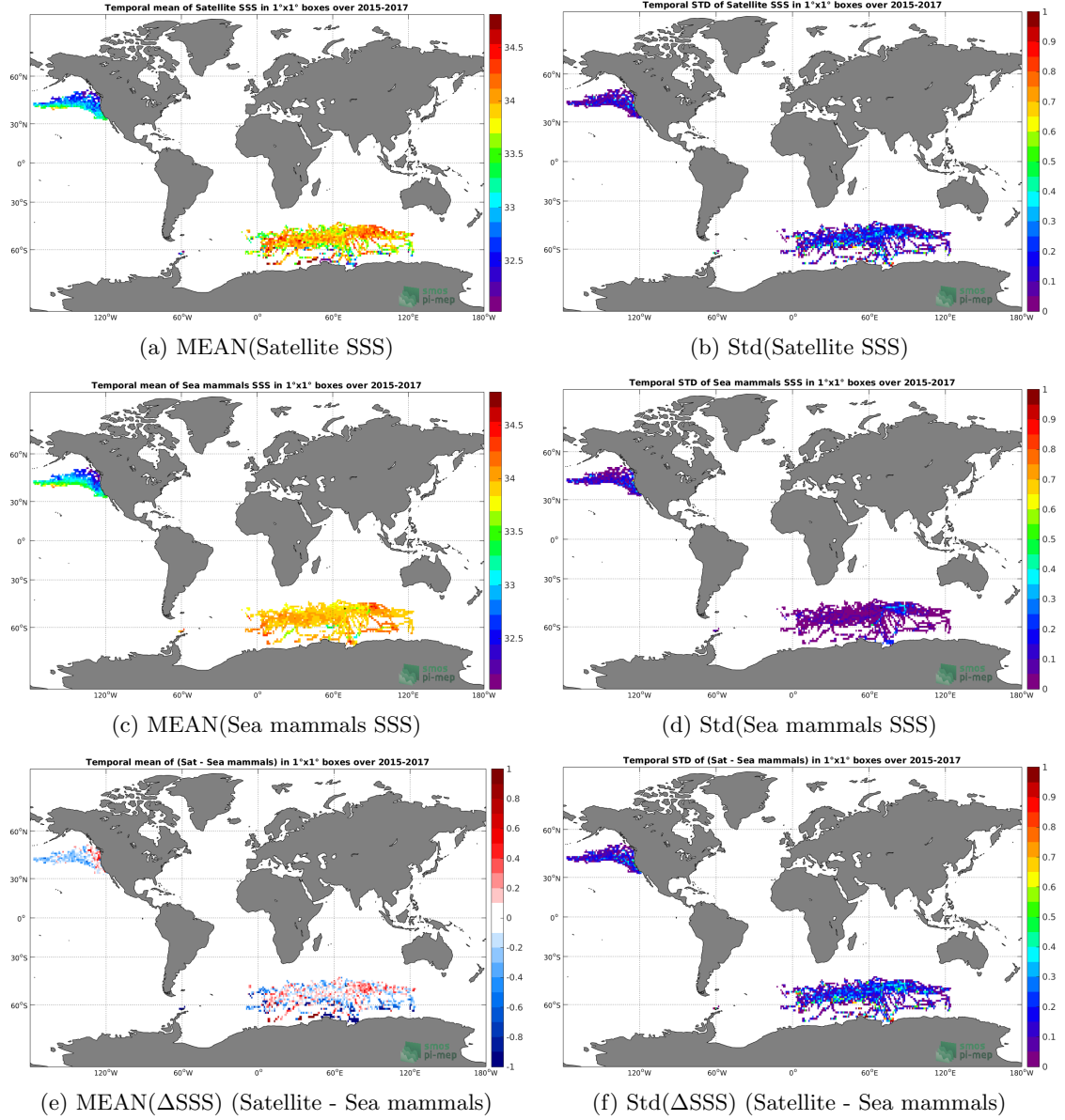
Figure 6: Temporal mean (left) and Std (right) of SSS from SMAP-L3-RSS-V4-MONTHLY (top), Sea mammals (middle), and of \Delta SSS (Satellite - Sea mammals). Only match-up pairs are used to generate these maps.
