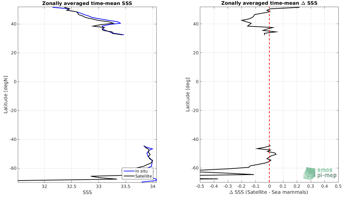
Figure 8: Left panel: Zonal mean SSS from SMAP-L3-RSS-V4-MONTHLY satellite product (black) and from Sea mammals (blue). Right panel: Zonal mean of \Delta SSS (Satellite - Sea mammals) for all the collected Pi-MEP match-up pairs estimated over the full satellite product period.
