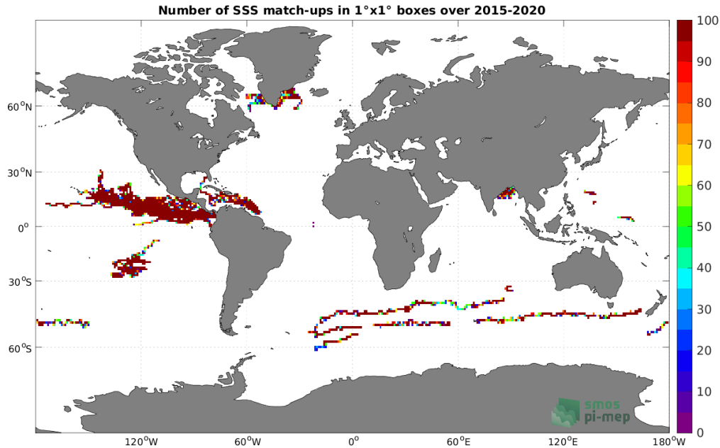
Figure 3: Number of SSS match-ups between Surface drifters SSS and the SMAP SSS L3 v4 - Monthly (RSS) SSS product for the Global Ocean Pi-MEP region over 1°×1° boxes and for the full satellite product period.
