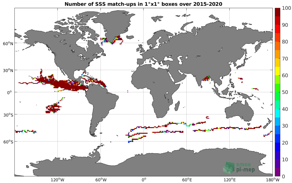
Figure 3: Number of SSS match-ups between Surface drifters SSS and the SMAP SSS L3 v4 - Monthly (RSS) SSS product for the Global Ocean Pi-MEP region over 1^\circ \times 1^\circ boxes and for the full satellite product period.
