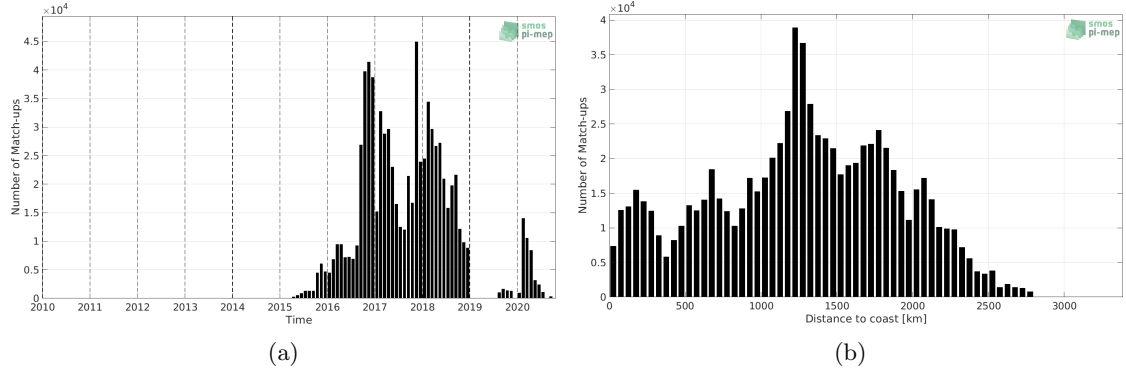
Figure 1: Number of match-ups between Surface drifters and SMAP SSS L3 v4 - Monthly (RSS) SSS as a function of time (a) and as function of the distance to coast (b) over the Global Ocean Pi-MEP region and for the full satellite product period.
