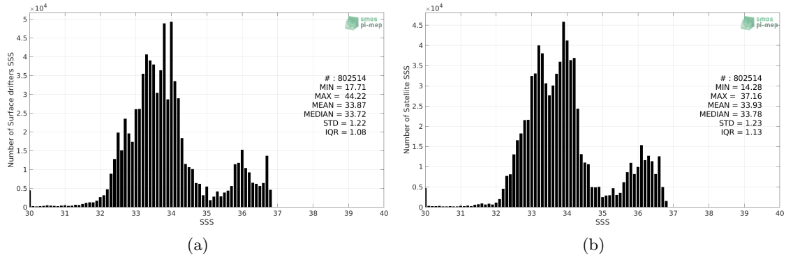
Figure 2: Histograms of SSS from Surface drifters (a) and SMAP SSS L3 v4 - Monthly (RSS) (b) considering all match-up pairs per bins of 0.1 over the Global Ocean Pi-MEP region and for the full satellite product period.
