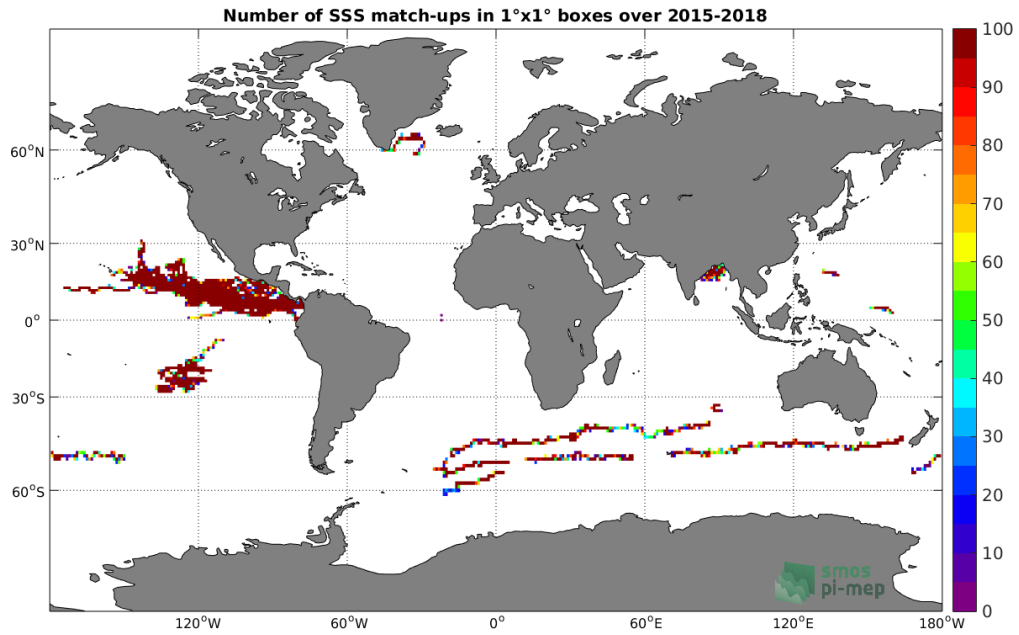
Figure 3: Number of SSS match-ups between Surface drifters SSS and the SMAP-L3-RSS-V4-MONTHLY SSS product for the Global Ocean Pi-MEP region over 1^\circ \times 1^\circ boxes and for the full satellite product period.
