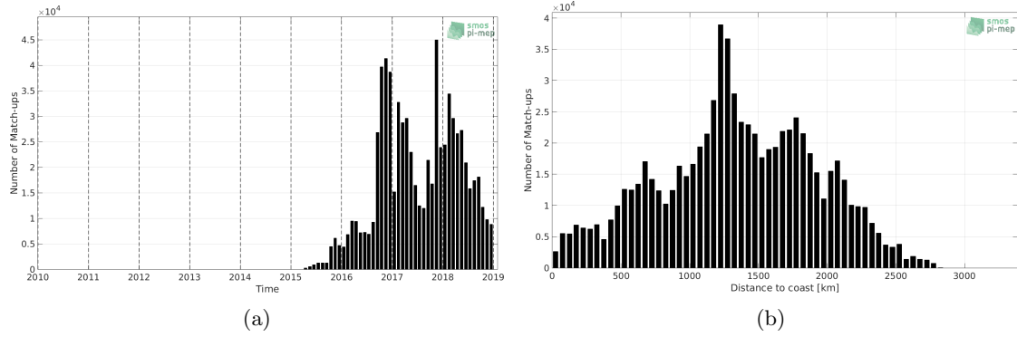
Figure 1: Number of match-ups between Surface drifters and SMAP-L3-RSS-V4-MONTHLY SSS as a function of time (a) and as function of the distance to coast (b) over the Global Ocean Pi-MEP region and for the full satellite product period.
