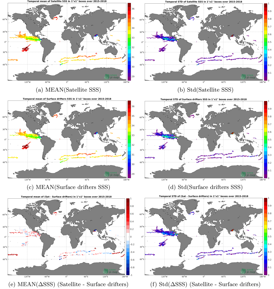
Figure 5: Temporal mean (left) and Std (right) of SSS from SMAP-L3-RSS-V4-MONTHLY (top), Surface drifters (middle), and of \Delta SSS (Satellite - Surface drifters). Only match-up pairs are used to generate these maps.
