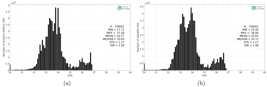
Figure 2: Histograms of SSS from Surface drifters (a) and SMAP-L3-RSS-V4-MONTHLY (b) considering all match-up pairs per bins of 0.1 over the Global Ocean Pi-MEP region and for the full satellite product period.
