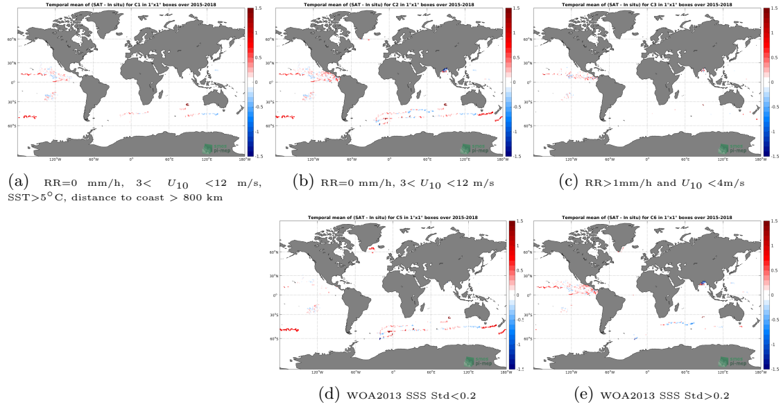
Figure 11: Temporal mean gridded over spatial boxes of size 1^\circ \times 1^\circ of \Delta SSS (SMAP-L3-RSS-V4-MONTHLY - Surface drifters) for 5 different subdatasets corresponding to:RR=0 mm/h, 3 < U_{10} < 12 m/s, SST >5^\circ C, distance to coast > 800 km (a), RR=0 mm/h, 3 < U_{10} < 12 m/s (b), RR >1 mm/h and U_{10} < 4 m/s (c), WOA2013 SSS Std <0.2 (d), WOA2013 SSS Std >0.2 (e).
