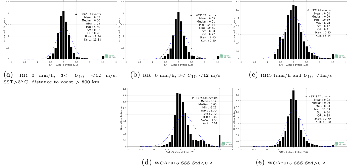
Figure 12: Normalized histogram of \Delta SSS (SMAP-L3-RSS-V4-MONTHLY - Surface drifters) for 5 different subdatasets corresponding to: RR=0 mm/h, 3 < U_{10} < 12 m/s, SST>5°C, distance to coast > 800 km (a), RR=0 mm/h, 3 < U_{10} < 12 m/s (b), RR>1mm/h and U_{10} < 4 m/s (c), WOA2013 SSS Std<0.2 (d), WOA2013 SSS Std>0.2 (e).
