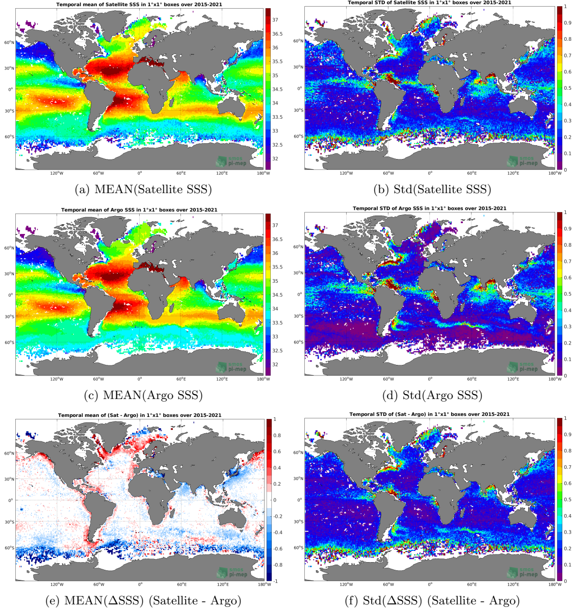
Figure 6: Temporal mean (left) and Std (right) of SSS from SMAP SSS L3 v4 - Monthly (RSS) (top), Argo (middle), and of \Delta SSS (Satellite - Argo). Only match-up pairs are used to generate these maps.
