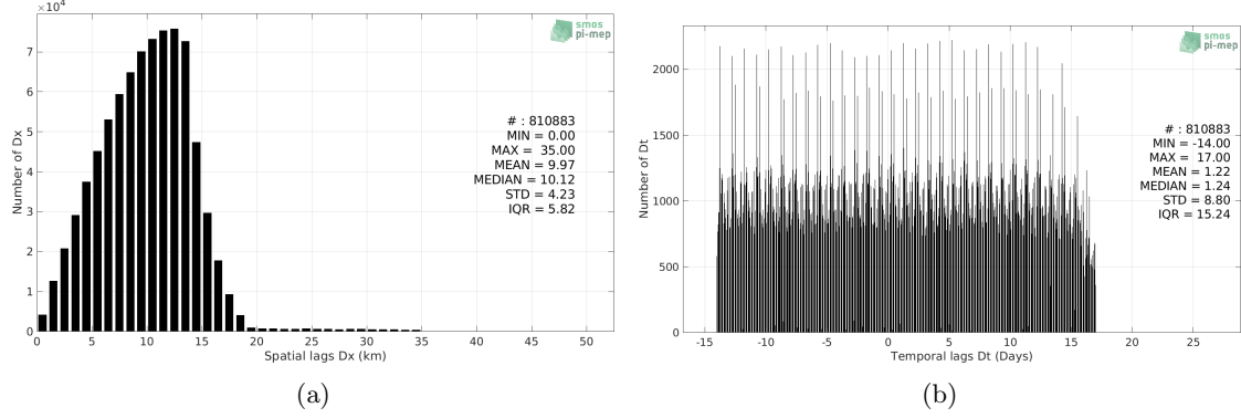
Figure 5: Histograms of the spatial (a) and temporal (b) lags between the location/time of the Argo measurement and the date of the corresponding SMAP SSS L3 v4 - Monthly (RSS) SSS pixel.
