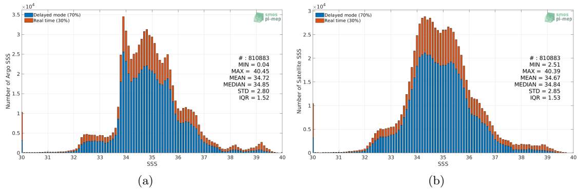
Figure 2: Histograms of SSS from Argo (a) and SMAP SSS L3 v4 - Monthly (RSS) (b) considering all match-up pairs per bins of 0.1 over the Global Ocean Pi-MEP region and for the full satellite product period.
