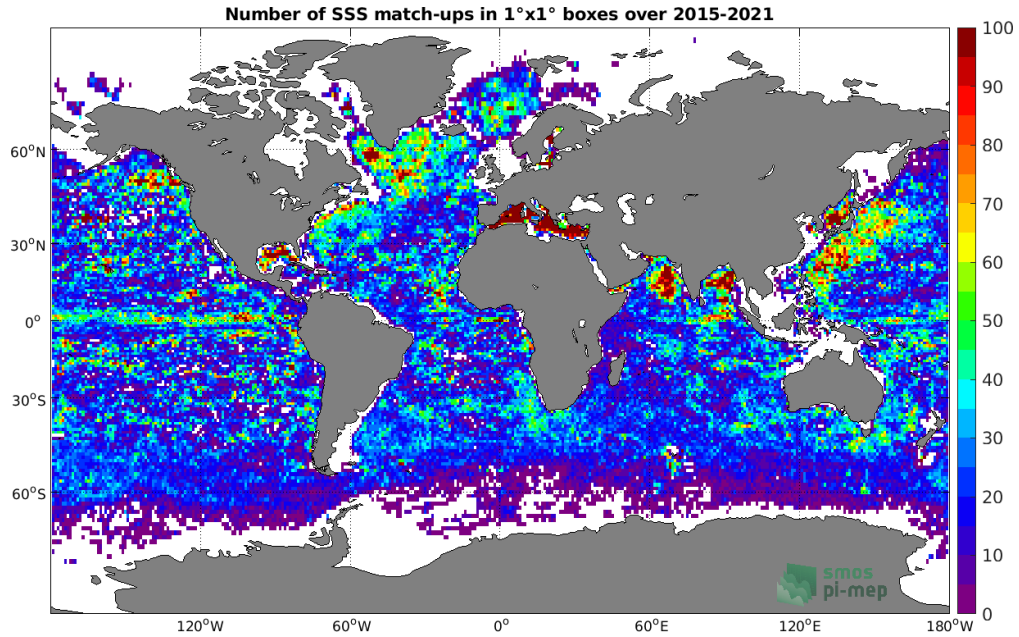
Figure 4: Number of SSS match-ups between Argo SSS and the SMAP SSS L3 v4 - Monthly (RSS) SSS product for the Global Ocean Pi-MEP region over 1^\circ \times 1^\circ boxes and for the full satellite product period.
