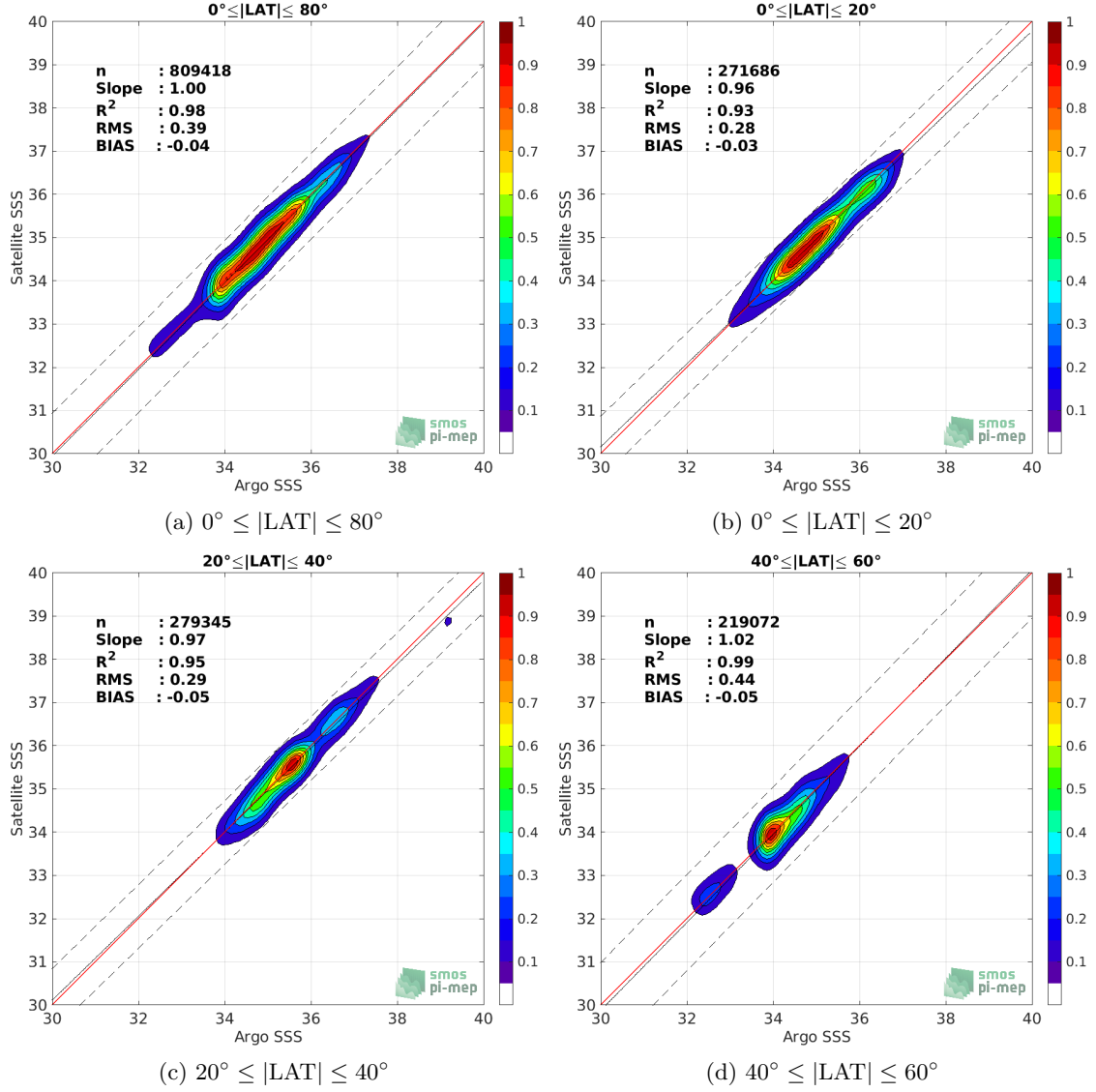
Figure 9: Contour maps of the concentration of SMAP SSS L3 v4 - Monthly (RSS) SSS (y-axis) versus Argo SSS (x-axis) at match-up pairs for different latitude bands. For each plot, the red line shows x=y . The black thin and dashed lines indicate a linear fit through the data cloud and the \pm 95\% confidence levels, respectively. The number match-up pairs n , the slope and R^2 coefficient of the linear fit, the root mean square (RMS) and the mean bias between satellite and in situ data are indicated for each latitude band in each plots.
