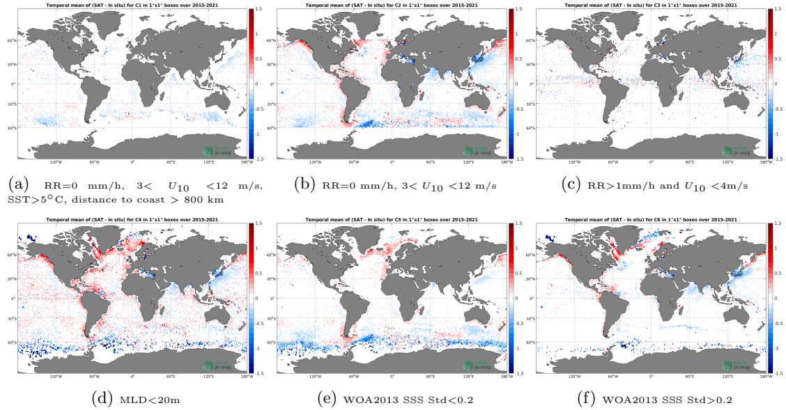
Figure 12: Temporal mean gridded over spatial boxes of size 1^\circ \times 1^\circ of \Delta SSS (SMAP SSS L3 v4 - Monthly (RSS) - Argo) for 6 different subdatasets corresponding to: RR=0 mm/h, 3 < U_{10} < 12 m/s, SST > 5^\circ\text{C} , distance to coast > 800 km (a), RR=0 mm/h, 3 < U_{10} < 12 m/s (b), RR > 1 mm/h and U_{10} < 4 m/s (c), MLD < 20 m (d), WOA2013 SSS Std < 0.2 (e), WOA2013 SSS Std > 0.2 (f).
