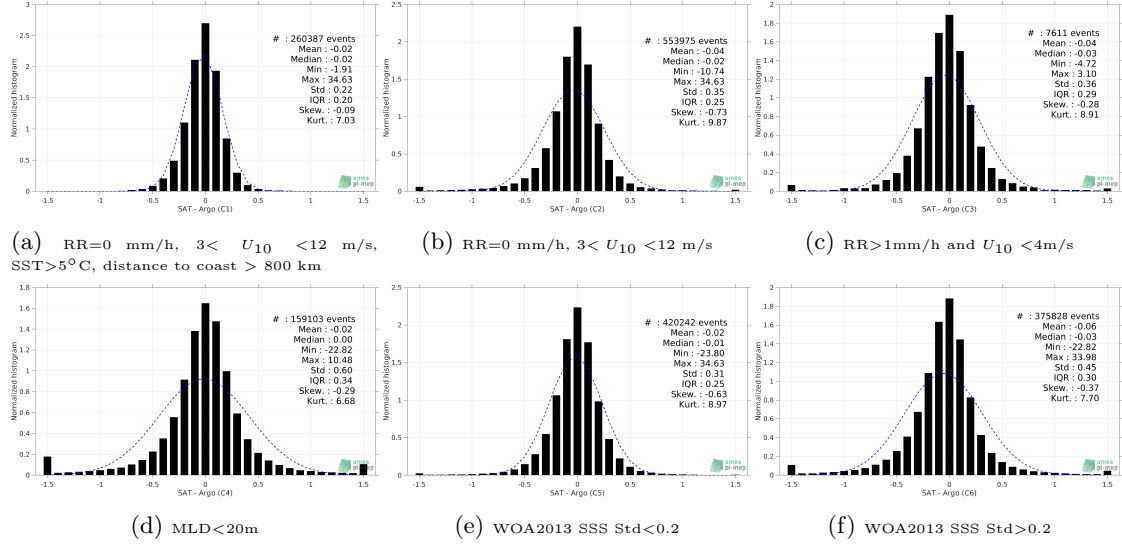
Figure 13: Normalized histogram of \Delta\text{SSS} (SMAP SSS L3 v4 - Monthly (RSS) - Argo) for 6 different subdatasets corresponding to: RR=0 mm/h, 3 < U_{10} < 12 m/s, SST>5°C, distance to coast > 800 km (a), RR=0 mm/h, 3 < U_{10} < 12 m/s (b), RR>1mm/h and U_{10} < 4 m/s (c), MLD<20m (d), WOA2013 SSS Std<0.2 (e), WOA2013 SSS Std>0.2 (f).
