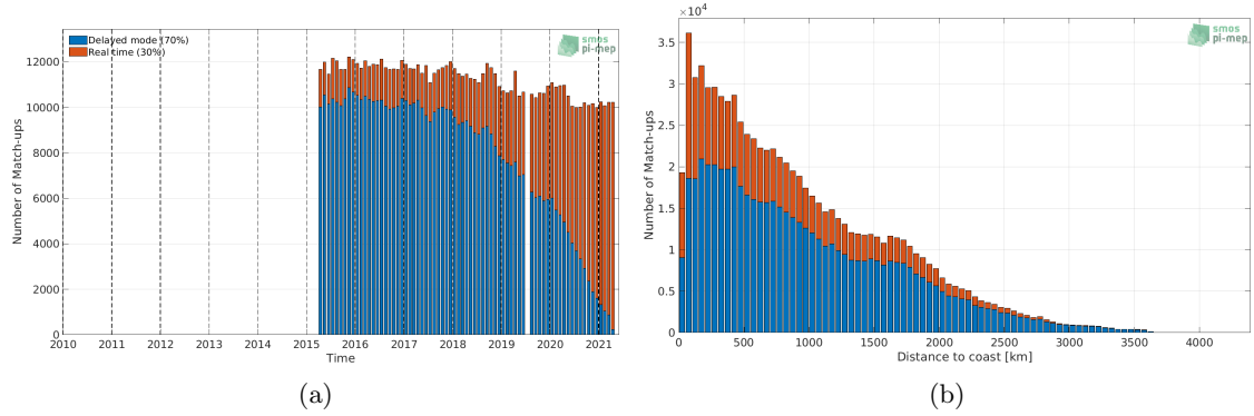
Figure 1: Number of match-ups between Argo and SMAP SSS L3 v4 - Monthly (RSS) SSS as a function of time (a) and as function of the distance to coast (b) over the Global Ocean Pi-MEP region and for the full satellite product period.
