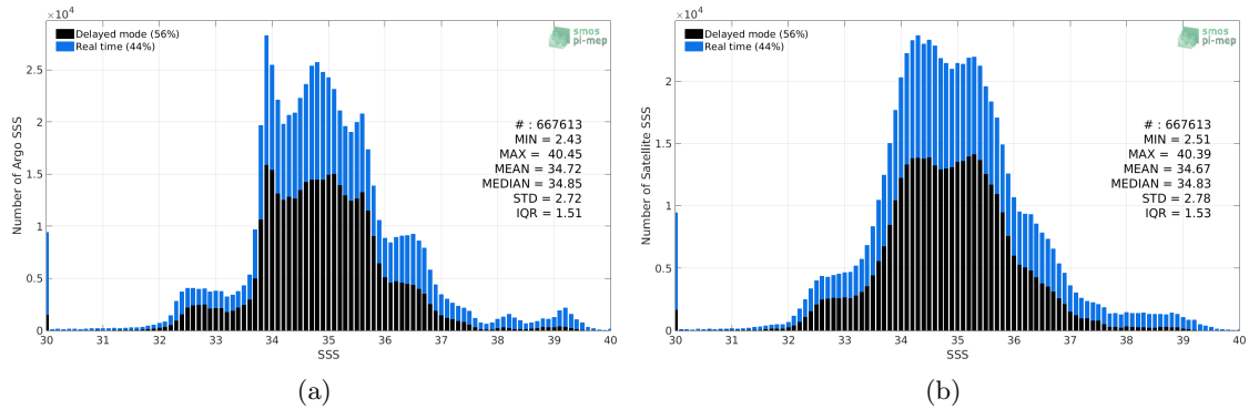
Figure 2: Histograms of SSS from Argo (a) and SMAP-L3-RSS-V4-MONTHLY (b) considering all match-up pairs per bins of 0.1 over the Global Ocean Pi-MEP region and for the full satellite product period.
