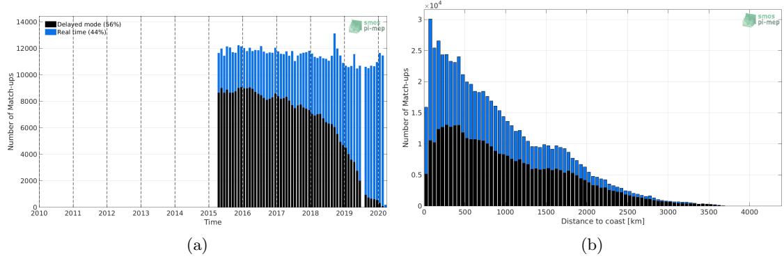
Figure 1: Number of match-ups between Argo and SMAP-L3-RSS-V4-MONTHLY SSS as a function of time (a) and as function of the distance to coast (b) over the Global Ocean Pi-MEP region and for the full satellite product period.
