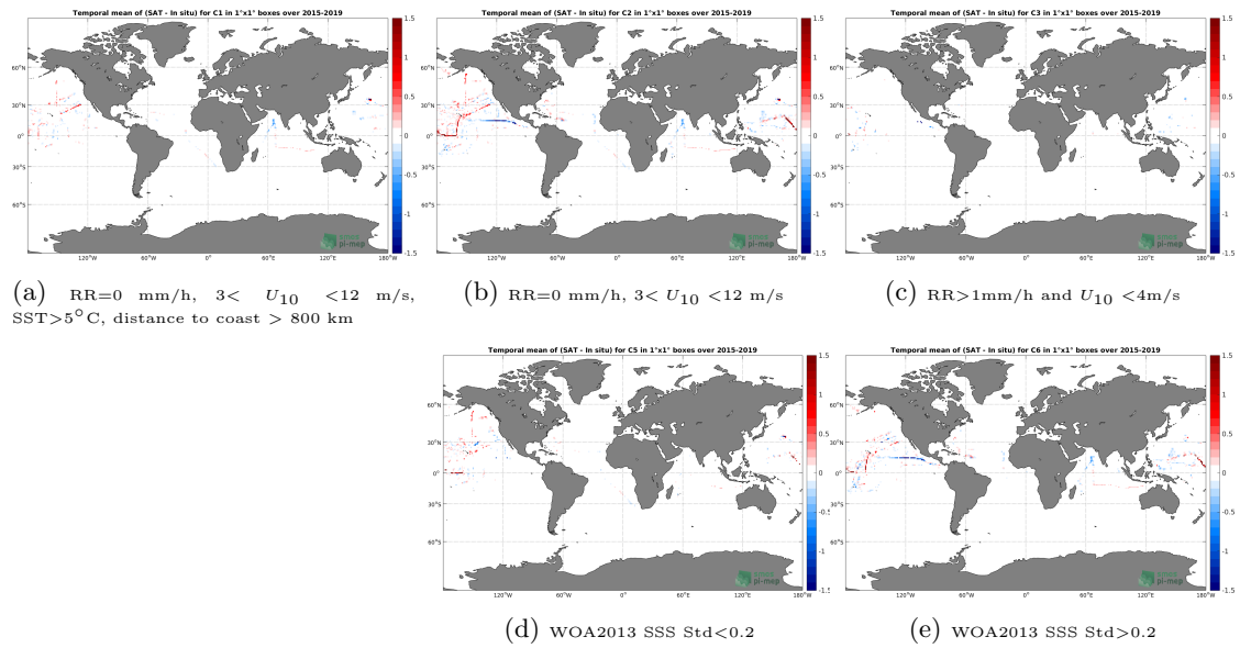
Figure 12: Temporal mean gridded over spatial boxes of size 1^\circ \times 1^\circ of \Delta SSS (SMAP-L3-RSS-V3-8DAY-RUNNING-70KM - TSG-SAMOS) for 5 different subdatasets corresponding to:RR=0 mm/h, 3 < U_{10} < 12 m/s, SST > 5^\circ\text{C} , distance to coast > 800 km (a), RR=0 mm/h, 3 < U_{10} < 12 m/s (b), RR > 1 mm/h and U_{10} < 4 m/s (c), WOA2013 SSS Std < 0.2 (d), WOA2013 SSS Std > 0.2 (e).
