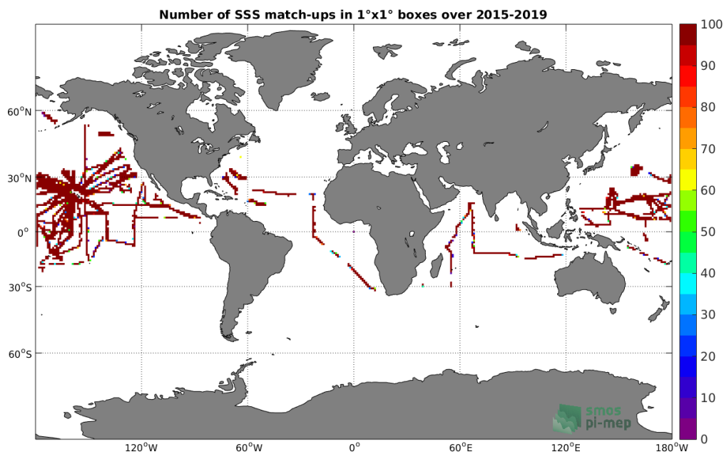
Figure 4: Number of SSS match-ups between TSG-SAMOS SSS and the SMAP-L3-RSS-V3-8DAY-RUNNING-70KM SSS product for the Global Ocean Pi-MEP region over 1^\circ \times 1^\circ boxes and for the full satellite product period.
