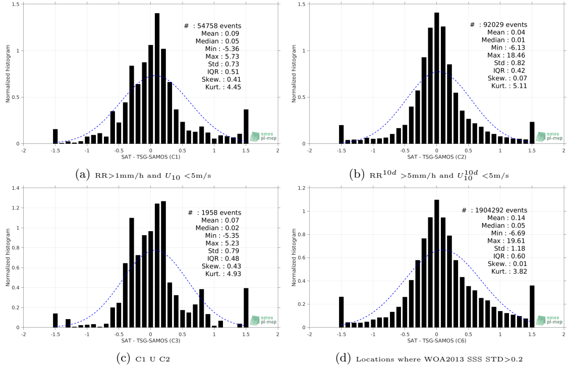
Figure 13: Normalized histogram of \Delta SSS (SMAP-L3-RSS-V3-8DAY-RUNNING-70KM - TSG-SAMOS) for 6 different subdatasets corresponding to: RR > 1mm/h and U_{10} < 5 m/s (a), RR^{10d} > 5 mm/h and U_{10}^{10d} < 5 m/s (b), C1 U C2 (c), Locations where WOA2013 SSS STD > 0.2 (d).
