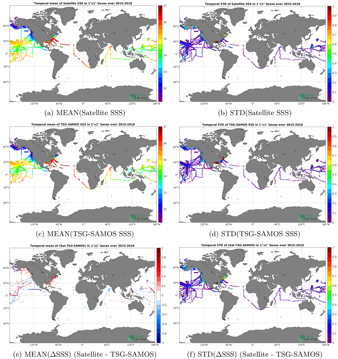
Figure 6: Temporal mean (left) and STD (right) of SSS from SMAP-L3-RSS-V3-8DAY-RUNNING-70KM (top), TSG-SAMOS (middle), and of \Delta SSS (Satellite - TSG-SAMOS). Only match-up pairs are used to generate these maps.
