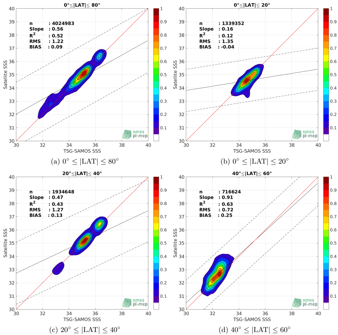
Figure 9: Contour maps of the concentration of SMAP-L3-RSS-V3-8DAY-RUNNING-70KM SSS (y-axis) versus TSG-SAMOS SSS (x-axis) at match-up pairs for different latitude bands. For each plot, the red line shows x=y . The black thin and dashed lines indicate a linear fit through the data cloud and the \pm 95\% confidence levels, respectively. The number match-up pairs n , the slope and R^2 coefficient of the linear fit, the root mean square (RMS) and the mean bias between satellite and in situ data are indicated for each latitude band in each plots.
