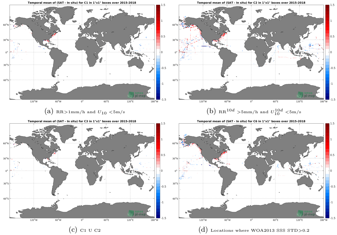
Figure 12: Temporal mean gridded over spatial boxes of size 1^\circ \times 1^\circ of \Delta SSS (SMAP-L3-RSS-V3-8DAY-RUNNING-70KM - TSG-SAMOS) for 4 different subdatasets corresponding to: RR > 1\text{mm/h} and U_{10} < 5\text{m/s} (a), RR^{10d} > 5\text{mm/h} and U_{10}^{10d} < 5\text{m/s} (b), C1 U C2 (c), Locations where WOA2013 SSS STD > 0.2 (d).
