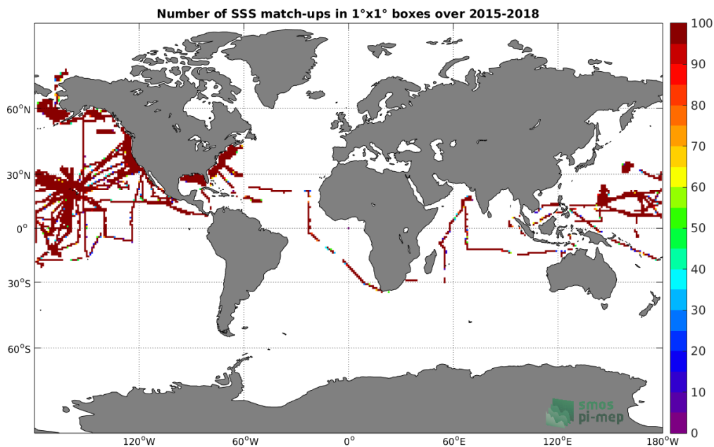
Figure 4: Number of SSS match-ups between TSG-SAMOS SSS and the SMAP-L3-RSS-V3-8DAY-RUNNING-70KM SSS product for the Global Ocean Pi-MEP region over 1^{\circ} \times 1^{\circ} boxes and for the full satellite product period.
