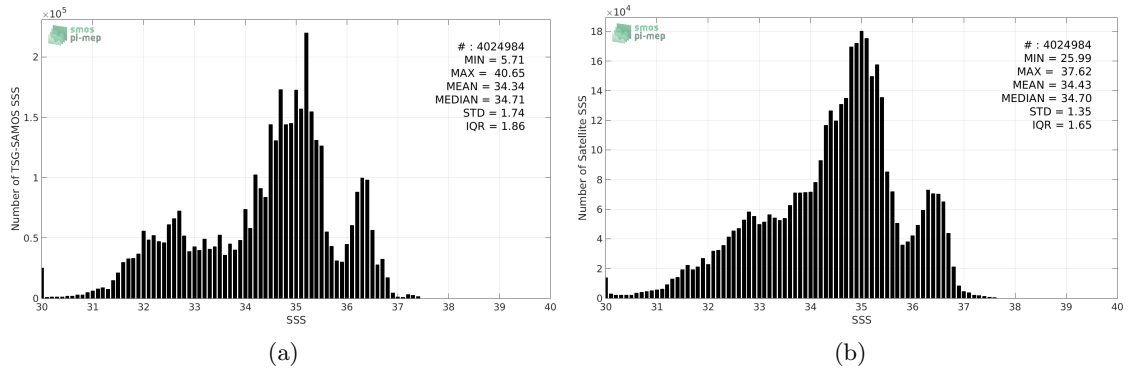
Figure 2: Histograms of SSS from TSG-SAMOS (a) and SMAP-L3-RSS-V3-8DAY-RUNNING-70KM (b) considering all match-up pairs per bins of 0.1 over the Global Ocean Pi-MEP region and for the full satellite product period.
