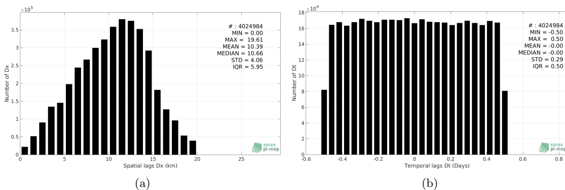
Figure 5: Histograms of the spatial (a) and temporal (b) lags between the time of the TSG-SAMOS measurements and the date of the corresponding SMAP-L3-RSS-V3-8DAY-RUNNING-70KM SSS product.
