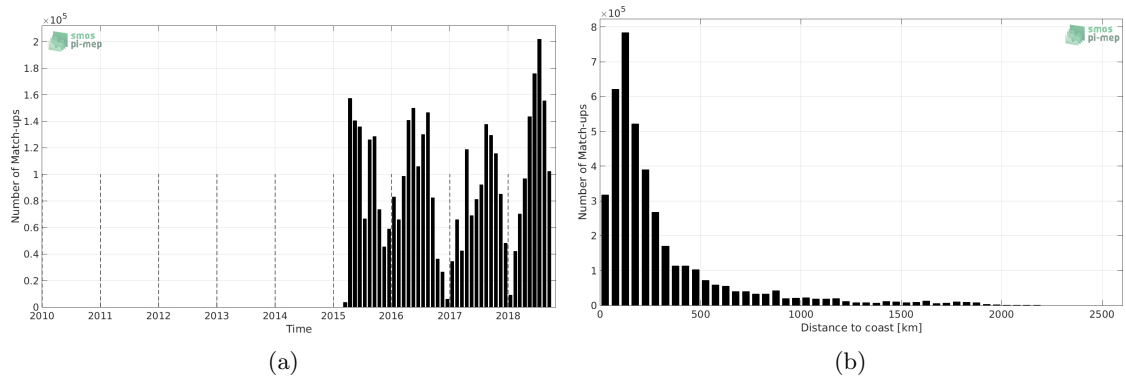
Figure 1: Number of match-ups between TSG-SAMOS and SMAP-L3-RSS-V3-8DAY-RUNNING-70KM SSS as a function of time (a) and as function of the distance to coast (b) over the Global Ocean Pi-MEP region and for the full satellite product period.
