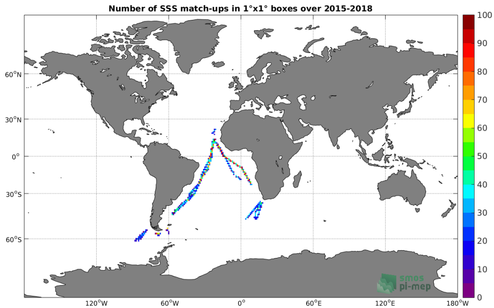
Figure 4: Number of SSS match-ups between TSG-POLARSTERN SSS and the SMAP-L3-RSS-V3-8DAY-RUNNING-70KM SSS product for the Global Ocean Pi-MEP region over 1^\circ \times 1^\circ boxes and for the full satellite product period.
