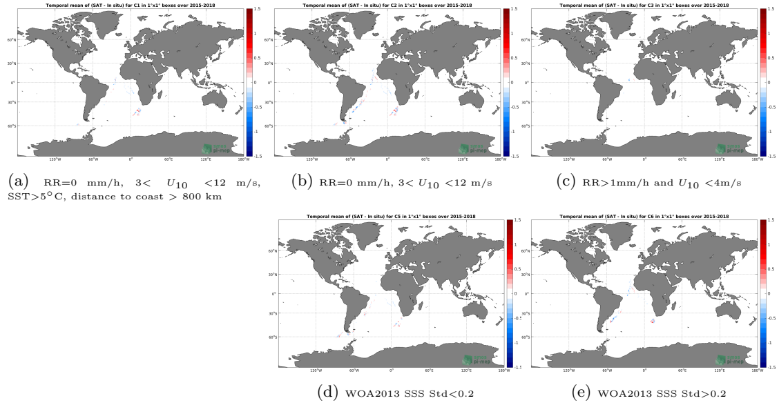
Figure 12: Temporal mean gridded over spatial boxes of size 1^\circ \times 1^\circ of \Delta SSS (SMAP-L3-RSS-V3-8DAY-RUNNING-70KM - TSG-POLARSTERN) for 5 different subdatasets corresponding to:RR=0 mm/h, 3 < U_{10} < 12 m/s, SST >5^\circ\text{C} , distance to coast > 800 km (a), RR=0 mm/h, 3 < U_{10} < 12 m/s (b), RR >1 mm/h and U_{10} < 4 m/s (c), WOA2013 SSS Std <0.2 (d), WOA2013 SSS Std >0.2 (e).
