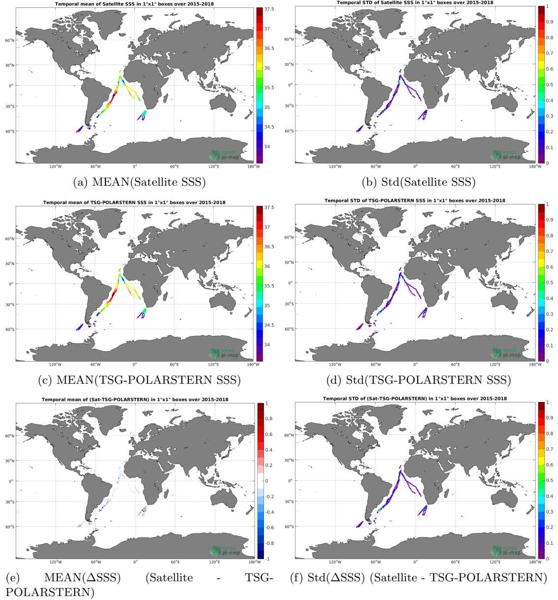
Figure 6: Temporal mean (left) and Std (right) of SSS from SMAP-L3-RSS-V3-8DAY-RUNNING-70KM (top), TSG-POLARSTERN (middle), and of \Delta SSS (Satellite - TSG-POLARSTERN). Only match-up pairs are used to generate these maps.
