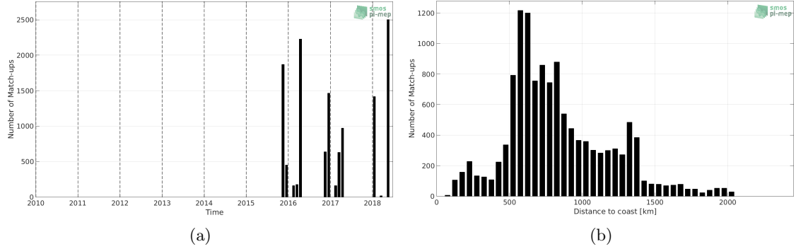
Figure 1: Number of match-ups between TSG-POLARSTERN and SMAP-L3-RSS-V3-8DAY-RUNNING-70KM SSS as a function of time (a) and as function of the distance to coast (b) over the Global Ocean Pi-MEP region and for the full satellite product period.
