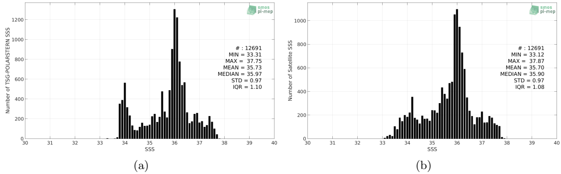
Figure 2: Histograms of SSS from TSG-POLARSTERN (a) and SMAP-L3-RSS-V3-8DAY-RUNNING-70KM (b) considering all match-up pairs per bins of 0.1 over the Global Ocean Pi-MEP region and for the full satellite product period.
