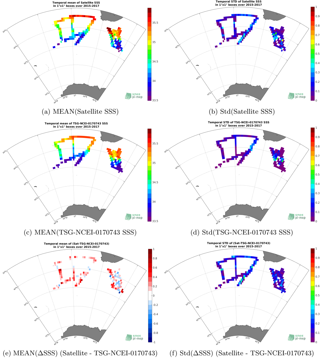
Figure 6: Temporal mean (left) and Std (right) of SSS from SMAP-L3-RSS-V3-8DAY-RUNNING-70KM (top), TSG-NCEI-0170743 (middle), and of \Delta SSS (Satellite - TSG-NCEI-0170743). Only match-up pairs are used to generate these maps.
