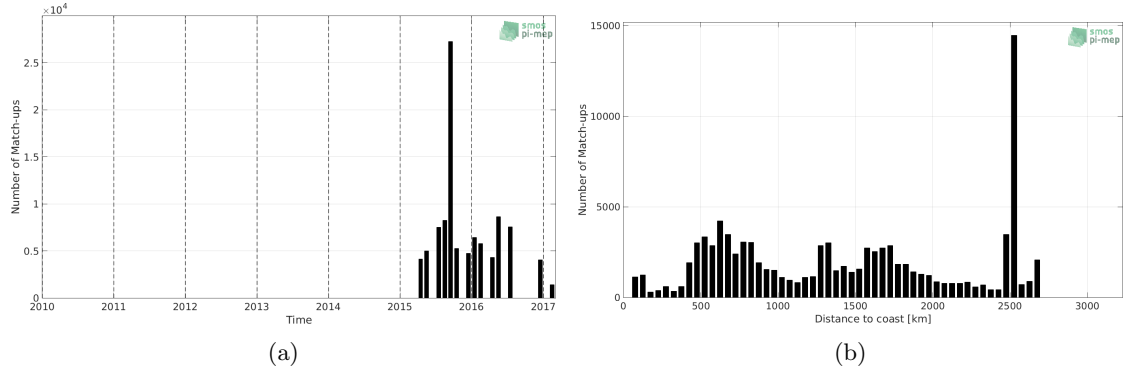
Figure 1: Number of match-ups between TSG-NCEI-0170743 and SMAP-L3-RSS-V3-8DAY-RUNNING-70KM SSS as a function of time (a) and as function of the distance to coast (b) over the Global Ocean Pi-MEP region and for the full satellite product period.
