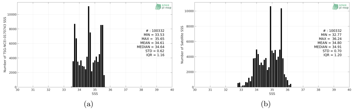
Figure 2: Histograms of SSS from TSG-NCEI-0170743 (a) and SMAP-L3-RSS-V3-8DAY-RUNNING-70KM (b) considering all match-up pairs per bins of 0.1 over the Global Ocean Pi-MEP region and for the full satellite product period.
