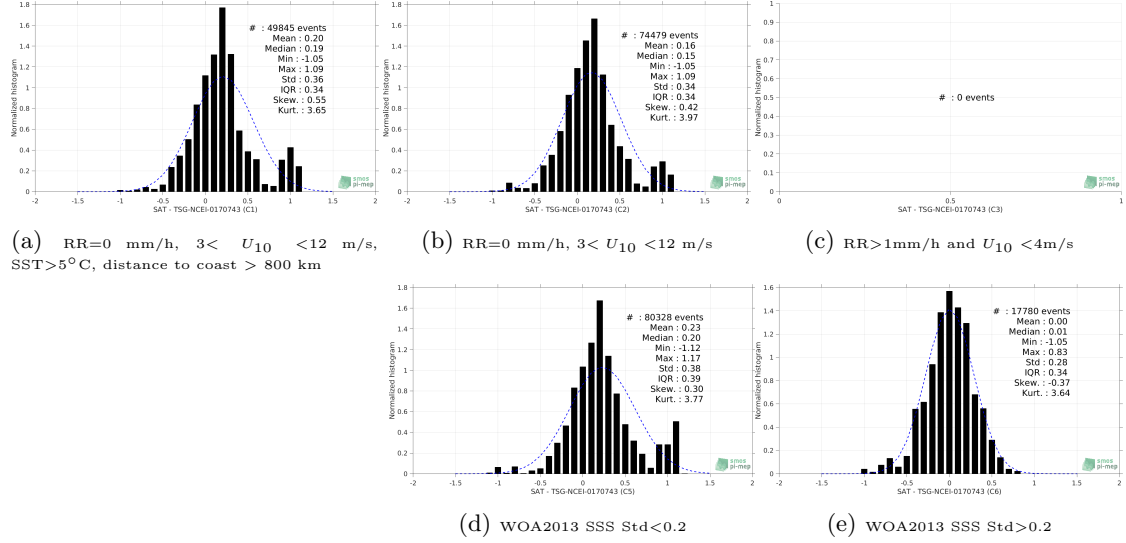
Figure 13: Normalized histogram of \Delta SSS (SMAP-L3-RSS-V3-8DAY-RUNNING-70KM - TSG-NCEI-0170743) for 5 different subdatasets corresponding to: RR=0 mm/h, 3 < U_{10} < 12 m/s, SST>5°C, distance to coast > 800 km (a), RR=0 mm/h, 3 < U_{10} < 12 m/s (b), RR>1mm/h and U_{10} < 4 m/s (c), WOA2013 SSS Std<0.2 (d), WOA2013 SSS Std>0.2 (e).
