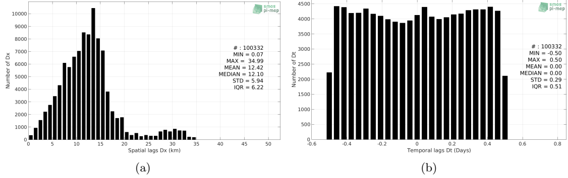
Figure 5: Histograms of the spatial (a) and temporal (b) lags between the time of the TSG-NCEI-0170743 measurements and the date of the corresponding SMAP-L3-RSS-V3-8DAY-RUNNING-70KM SSS product.
