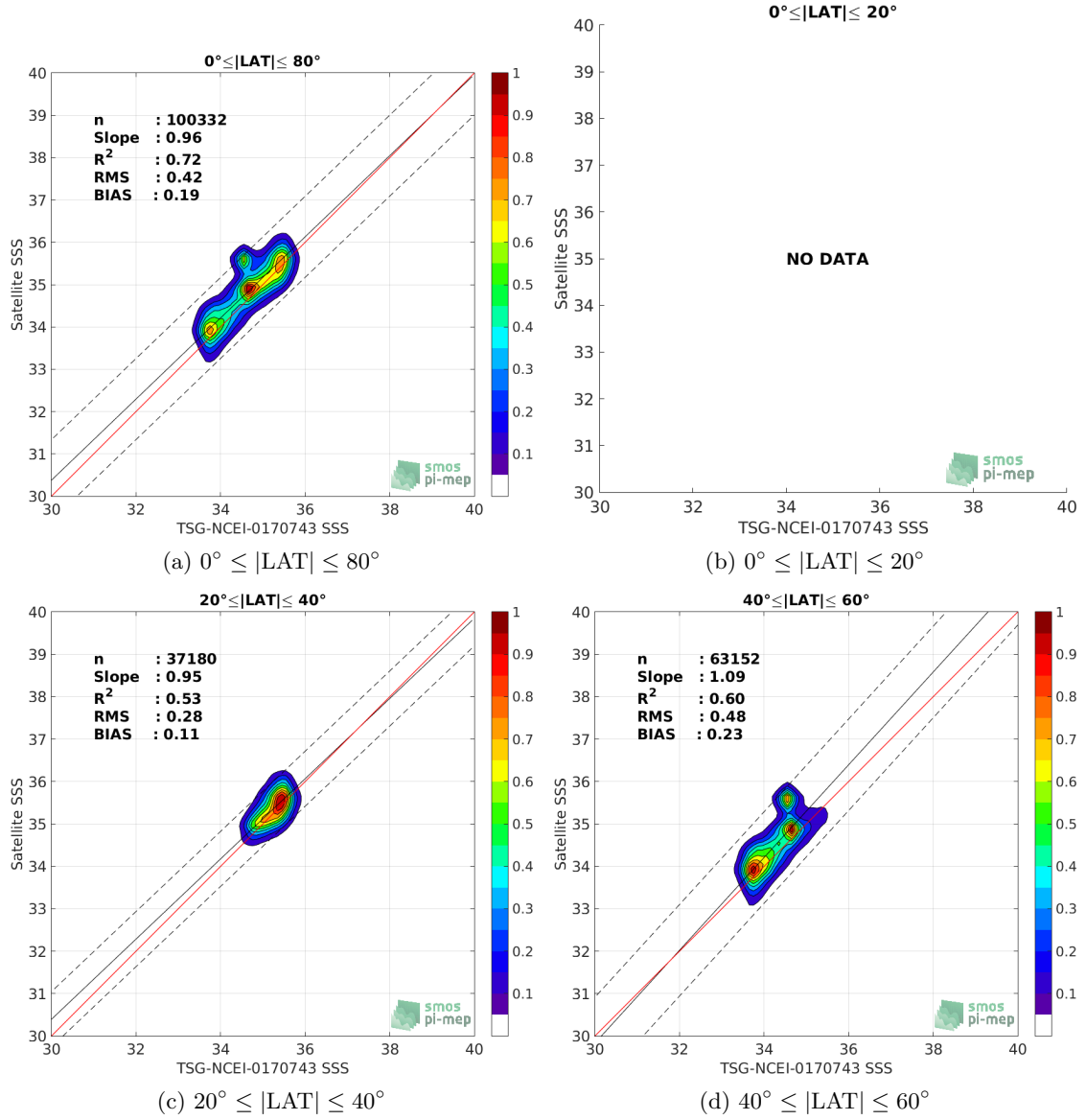
Figure 9: Contour maps of the concentration of SMAP-L3-RSS-V3-8DAY-RUNNING-70KM SSS (y-axis) versus TSG-NCEI-0170743 SSS (x-axis) at match-up pairs for different latitude bands. For each plot, the red line shows x=y . The black thin and dashed lines indicate a linear fit through the data cloud and the \pm 95\% confidence levels, respectively. The number match-up pairs n , the slope and R^2 coefficient of the linear fit, the root mean square (RMS) and the mean bias between satellite and in situ data are indicated for each latitude band in each plots.
