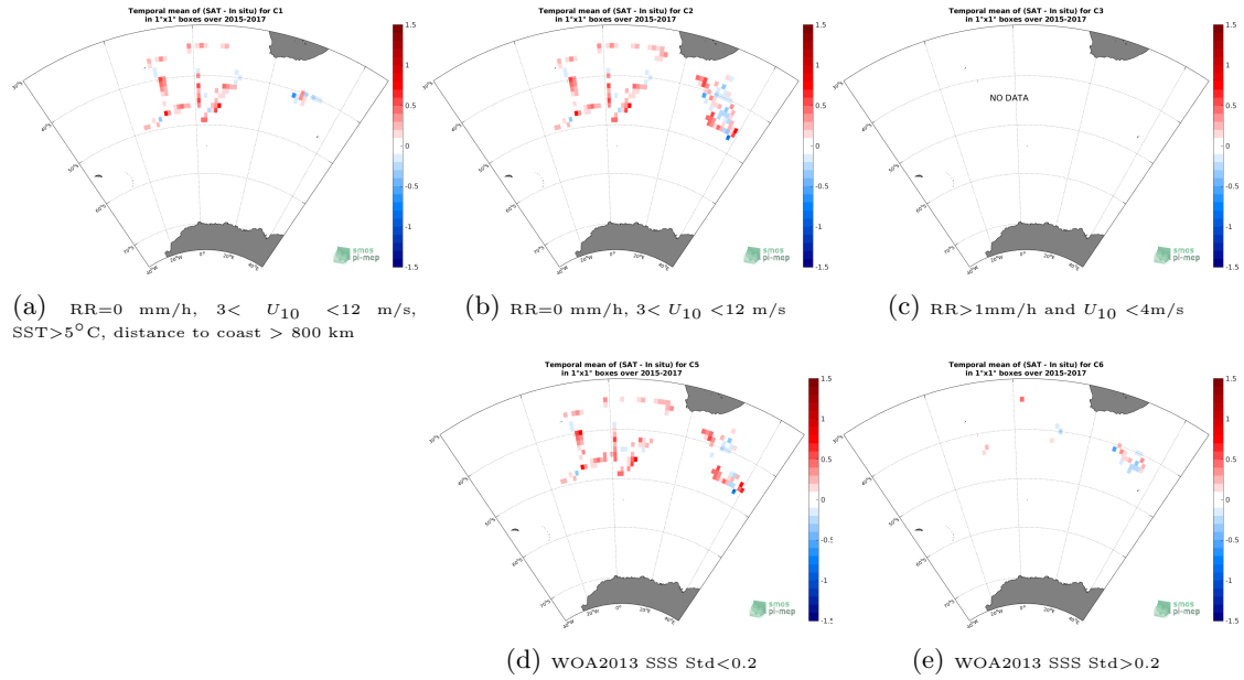
Figure 12: Temporal mean gridded over spatial boxes of size 1^\circ \times 1^\circ of \Delta SSS (SMAP-L3-RSS-V3-8DAY-RUNNING-70KM - TSG-NCEI-0170743) for 5 different subdatasets corresponding to: RR=0 mm/h, 3 < U_{10} < 12 m/s, SST > 5^\circ\text{C} , distance to coast > 800 km (a), RR=0 mm/h, 3 < U_{10} < 12 m/s (b), RR > 1\text{mm/h} and U_{10} < 4\text{m/s} (c), WOA2013 SSS Std < 0.2 (d), WOA2013 SSS Std > 0.2 (e).
