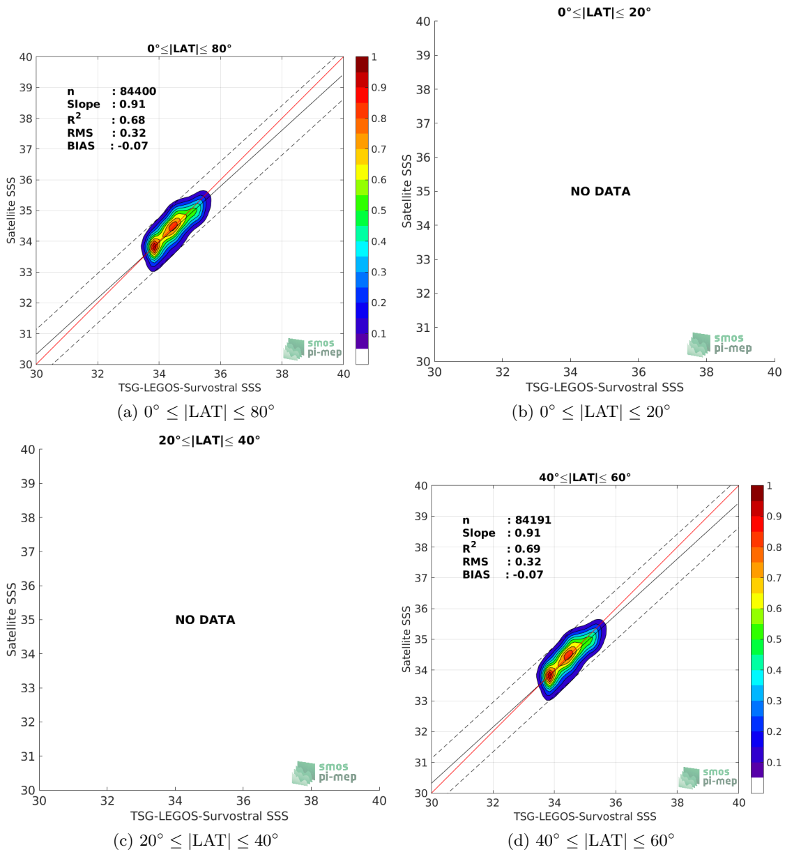
Figure 9: Contour maps of the concentration of SMAP-L3-RSS-V3-8DAY-RUNNING-70KM SSS (y-axis) versus TSG-LEGOS-Survostral SSS (x-axis) at match-up pairs for different latitude bands. For each plot, the red line shows x=y . The black thin and dashed lines indicate a linear fit through the data cloud and the \pm 95\% confidence levels, respectively. The number match-up pairs n , the slope and R^2 coefficient of the linear fit, the root mean square (RMS) and the mean bias between satellite and in situ data are indicated for each latitude band in each plots.
