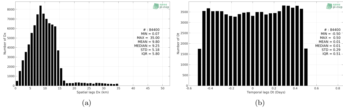
Figure 5: Histograms of the spatial (a) and temporal (b) lags between the time of the TSG-LEGOS-Survostral measurements and the date of the corresponding SMAP-L3-RSS-V3-8DAY-RUNNING-70KM SSS product.
