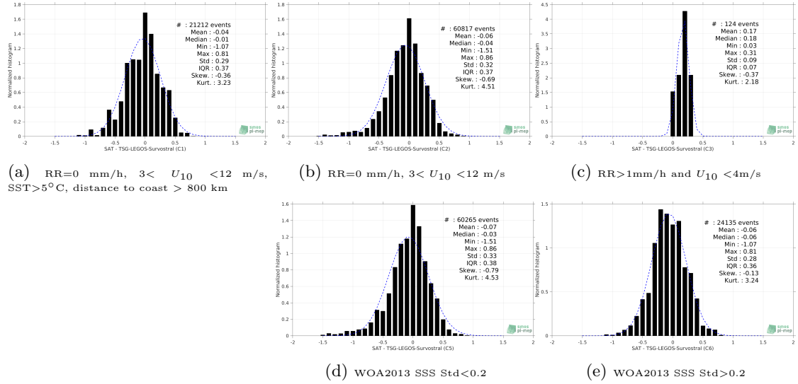
Figure 13: Normalized histogram of \Delta SSS (SMAP-L3-RSS-V3-8DAY-RUNNING-70KM - TSG-LEGOS-Survostral) for 5 different subdatasets corresponding to: RR=0 mm/h, 3 < U_{10} < 12 m/s, SST>5°C, distance to coast > 800 km (a), RR=0 mm/h, 3 < U_{10} < 12 m/s (b), RR>1mm/h and U_{10} < 4 m/s (c), WOA2013 SSS Std<0.2 (d), WOA2013 SSS Std>0.2 (e).
