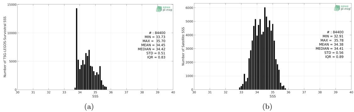
Figure 2: Histograms of SSS from TSG-LEGOS-Survostral (a) and SMAP-L3-RSS-V3-8DAY-RUNNING-70KM (b) considering all match-up pairs per bins of 0.1 over the Global Ocean Pi-MEP region and for the full satellite product period.
