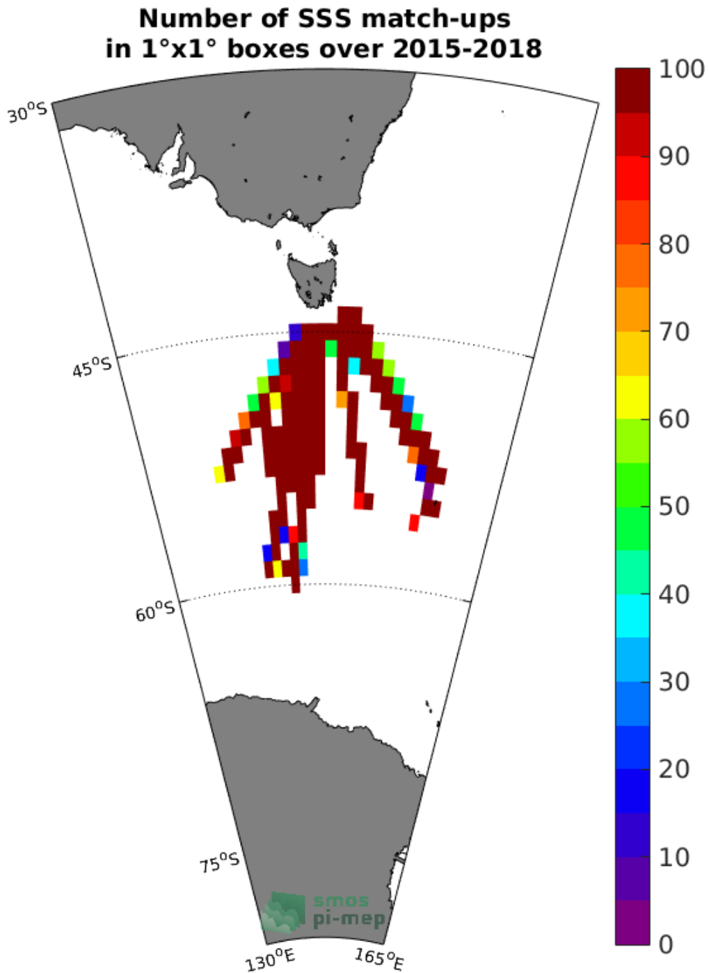
Figure 4: Number of SSS match-ups between TSG-LEGOS-Survostral SSS and the SMAP-L3-RSS-V3-8DAY-RUNNING-70KM SSS product for the Global Ocean Pi-MEP region over 1°x1° boxes and for the full satellite product period.
