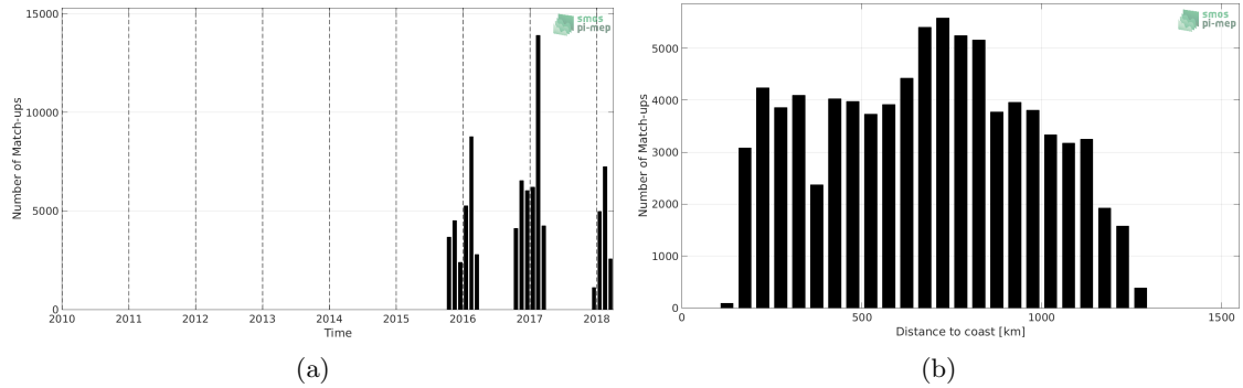
Figure 1: Number of match-ups between TSG-LEGOS-Survostral and SMAP-L3-RSS-V3-8DAY-RUNNING-70KM SSS as a function of time (a) and as function of the distance to coast (b) over the Global Ocean Pi-MEP region and for the full satellite product period.
