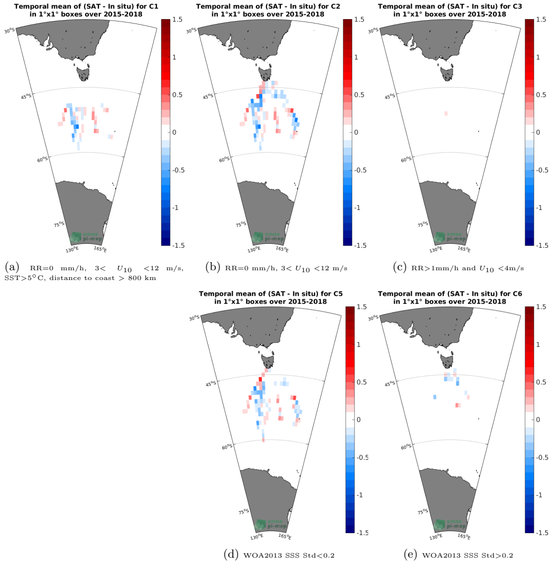
Figure 12: Temporal mean gridded over spatial boxes of size 1°x1° of \Delta SSS (SMAP-L3-RSS-V3-8DAY-RUNNING-70KM - TSG-LEGOS-Survostral) for 5 different subdatasets corresponding to:RR=0 mm/h, 3 < U_{10} < 12 m/s, SST>5°C, distance to coast > 800 km (a), RR=0 mm/h, 3 < U_{10} < 12 m/s (b), RR>1mm/h and U_{10} < 4 m/s (c), WOA2013 SSS Std<0.2 (d), WOA2013 SSS Std>0.2 (e).
