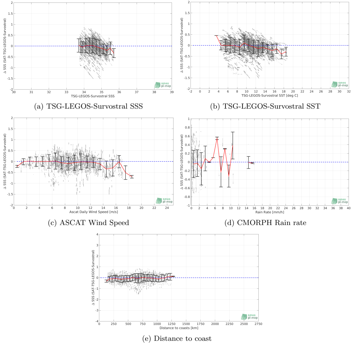
Figure 11: \Delta SSS (Satellite - TSG-LEGOS-Survostral) sorted as function of TSG-LEGOS-Survostral SSS values a), TSG-LEGOS-Survostral SST b), ASCAT Wind speed c), CMORPH rain rate d) and distance to coast (e). In all plots the mean and Std of \Delta SSS for each bin is indicated by the red curves and black vertical thick bars ( \pm 1 Std)
