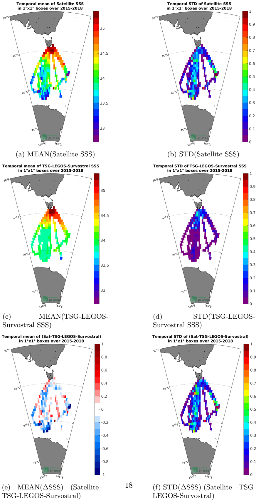
Figure 6: Temporal mean (left) and STD (right) of SSS from SMAP-L3-RSS-V3-8DAY-RUNNING-70KM (top), TSG-LEGOS-Survostral (middle), and of \Delta SSS (Satellite - TSG-LEGOS-Survostral). Only match-up pairs are used to generate these maps.
