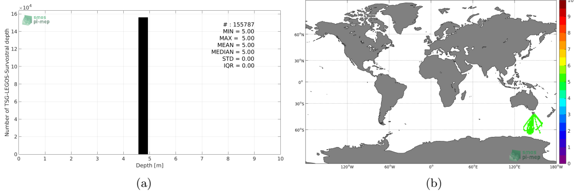
Figure 3: Histograms of the depth of the upper level SSS measurements from TSG-LEGOS-Survostral in the Match-up DataBase for the Global Ocean Pi-MEP region (a) and temporal mean spatial distribution of pressure of the in situ SSS data over 1^\circ \times 1^\circ boxes and for the full satellite product period (b).
