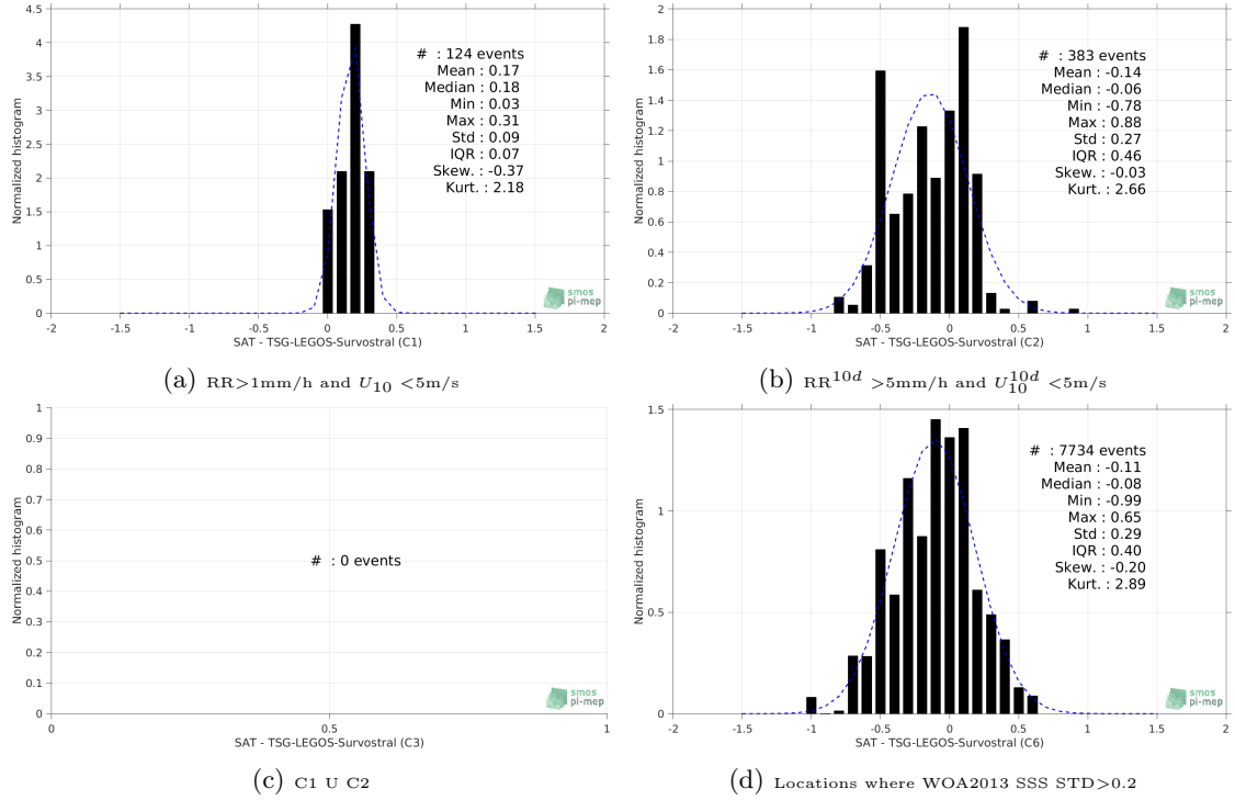
Figure 13: Normalized histogram of \Delta\text{SSS} (SMAP-L3-RSS-V3-8DAY-RUNNING-70KM - TSG-LEGOS-Survostral) for 6 different subdatasets corresponding to: RR > 1mm/h and U_{10} < 5\text{m/s} (a), RR^{10d} > 5\text{mm/h} and U_{10}^{10d} < 5\text{m/s} (b), C1 U C2 (c), Locations where WOA2013 SSS STD > 0.2 (d).
