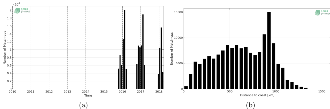
Figure 1: Number of match-ups between TSG-LEGOS-Survostral and SMAP-L3-RSS-V3-8DAY-RUNNING-70KM SSS as a function of time (a) and as function of the distance to coast (b) over the Global Ocean Pi-MEP region and for the full satellite product period.
