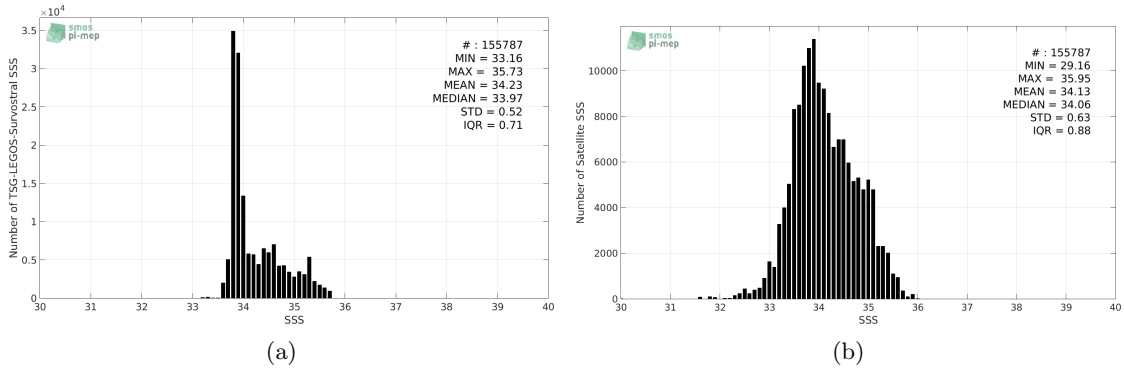
Figure 2: Histograms of SSS from TSG-LEGOS-Survostral (a) and SMAP-L3-RSS-V3-8DAY-RUNNING-70KM (b) considering all match-up pairs per bins of 0.1 over the Global Ocean Pi-MEP region and for the full satellite product period.
