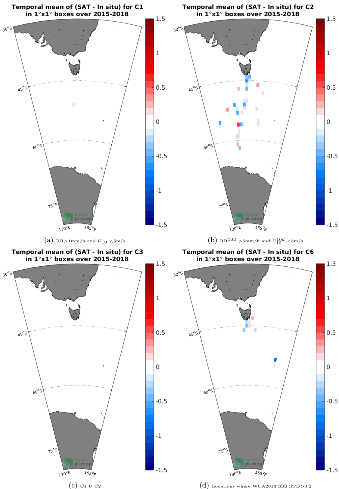
Figure 12: Temporal mean gridded over spatial boxes of size 1°x1° of \Delta\text{SSS} (SMAP-L3-RSS-V3-8DAY-RUNNING-70KM - TSG-LEGOS-Survostral) for 4 different subdatasets corresponding to: RR > 1\text{mm/h} and U_{10} < 5\text{m/s} (a), RR^{10d} > 5\text{mm/h} and U_{10}^{10d} < 5\text{m/s} (b), C1 U C2 (c), Locations where WOA2013 SSS STD > 0.2 (d).
