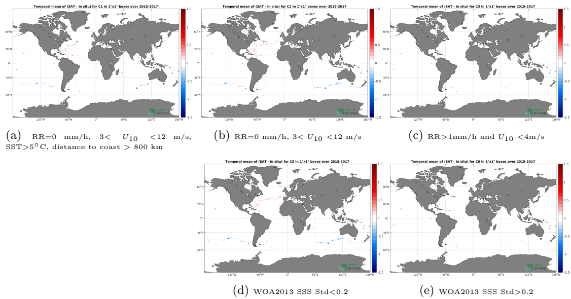
Figure 12: Temporal mean gridded over spatial boxes of size 1^\circ \times 1^\circ of \Delta SSS (SMAP-L3-RSS-V3-8DAY-RUNNING-70KM - TSG-GOSUD-Sailing-ship) for 5 different subdatasets corresponding to:RR=0 mm/h, 3 < U_{10} < 12 m/s, SST >5^\circ C, distance to coast > 800 km (a), RR=0 mm/h, 3 < U_{10} < 12 m/s (b), RR >1 mm/h and U_{10} < 4 m/s (c), WOA2013 SSS Std <0.2 (d), WOA2013 SSS Std >0.2 (e).
