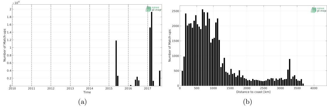
Figure 1: Number of match-ups between TSG-GOSUD-Sailing-ship and SMAP-L3-RSS-V3-8DAY-RUNNING-70KM SSS as a function of time (a) and as function of the distance to coast (b) over the Global Ocean Pi-MEP region and for the full satellite product period.
