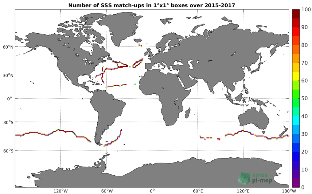
Figure 4: Number of SSS match-ups between TSG-GOSUD-Sailing-ship SSS and the SMAP-L3-RSS-V3-8DAY-RUNNING-70KM SSS product for the Global Ocean Pi-MEP region over 1^\circ \times 1^\circ boxes and for the full satellite product period.
