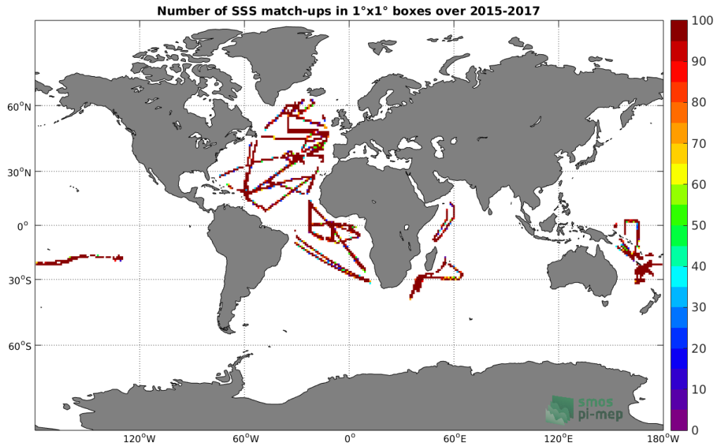
Figure 4: Number of SSS match-ups between TSG-GOSUD-Research-vessel SSS and the SMAP-L3-RSS-V3-8DAY-RUNNING-70KM SSS product for the Global Ocean Pi-MEP region over 1^\circ \times 1^\circ boxes and for the full satellite product period.
