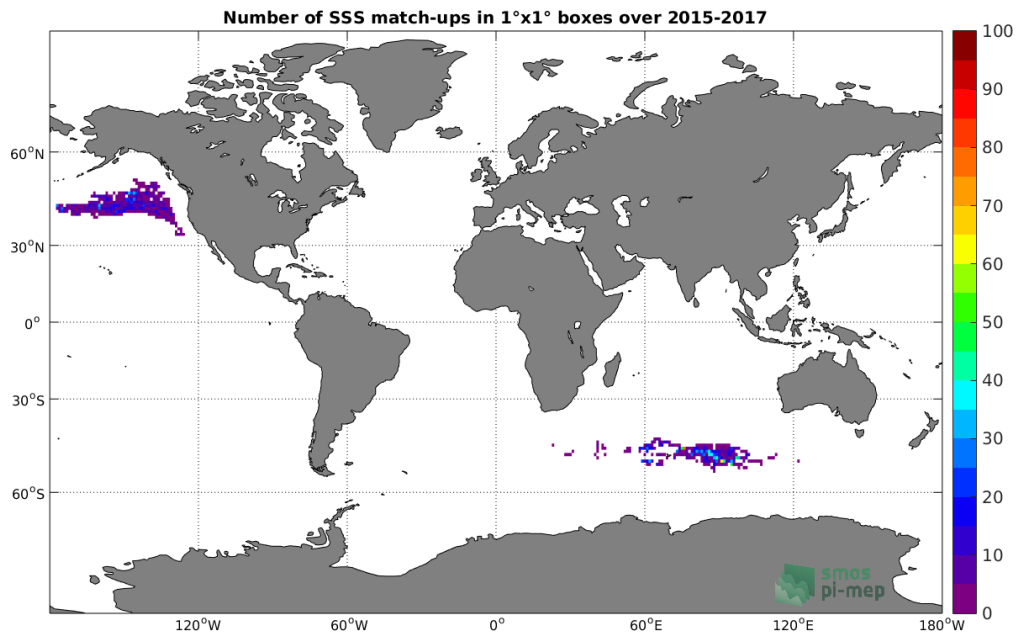
Figure 4: Number of SSS match-ups between Sea mammals SSS and the SMAP-L3-RSS-V3-8DAY-RUNNING-70KM SSS product for the Global Ocean Pi-MEP region over 1^\circ \times 1^\circ boxes and for the full satellite product period.
