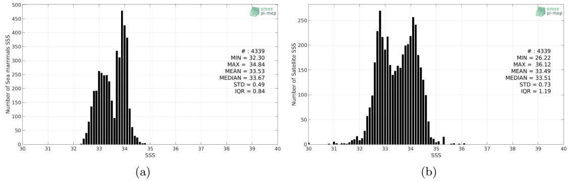
Figure 2: Histograms of SSS from Sea mammals (a) and SMAP-L3-RSS-V3-8DAY-RUNNING-70KM (b) considering all match-up pairs per bins of 0.1 over the Global Ocean Pi-MEP region and for the full satellite product period.
