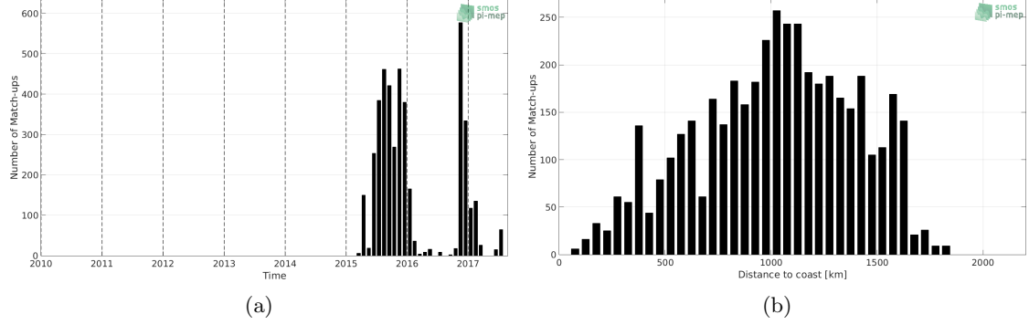
Figure 1: Number of match-ups between Sea mammals and SMAP-L3-RSS-V3-8DAY-RUNNING-70KM SSS as a function of time (a) and as function of the distance to coast (b) over the Global Ocean Pi-MEP region and for the full satellite product period.
