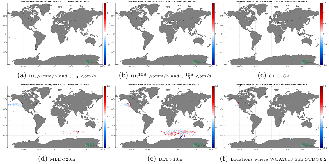
Figure 12: Temporal mean gridded over spatial boxes of size 1^\circ \times 1^\circ of \Delta\text{SSS} (SMAP-L3-RSS-V3-8DAY-RUNNING-70KM - Sea mammals) for 6 different subdatasets corresponding to: RR > 1\text{mm/h} and U_{10} < 5\text{m/s} (a), RR^{10d} > 5\text{mm/h} and U_{10}^{10d} < 5\text{m/s} (b), C1 U C2 (c), MLD < 20\text{m} (d), BLT > 10\text{m} (e), Locations where WOA2013 SSS STD > 0.2 (f).
