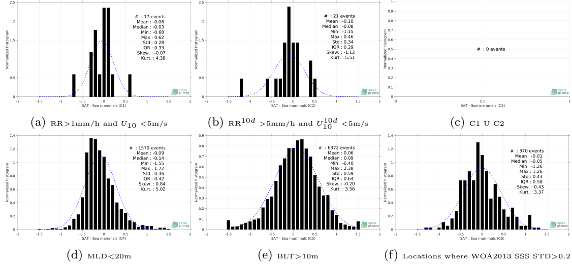
Figure 13: Normalized histogram of \Delta\text{SSS} (SMAP-L3-RSS-V3-8DAY-RUNNING-70KM - Sea mammals) for 6 different subdatasets corresponding to: \text{RR}>1\text{mm/h} and U_{10}<5\text{m/s} (a), \text{RR}^{10d}>5\text{mm/h} and U_{10}^{10d}<5\text{m/s} (b), \text{C1 U C2} (c), \text{MLD}<20\text{m} (d), \text{BLT}>10\text{m} (e), Locations where WOA2013 SSS \text{STD}>0.2 (f).
