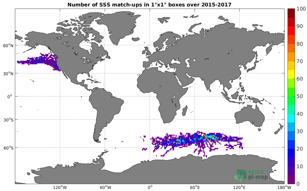
Figure 4: Number of SSS match-ups between Sea mammals SSS and the SMAP-L3-RSS-V3-8DAY-RUNNING-70KM SSS product for the Global Ocean Pi-MEP region over 1°x1° boxes and for the full satellite product period.
