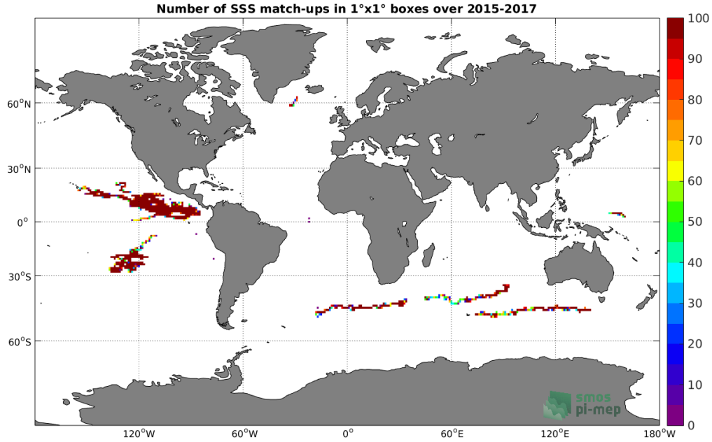
Figure 3: Number of SSS match-ups between Surface drifters SSS and the SMAP-L3-RSS-V3-8DAY-RUNNING-70KM SSS product for the Global Ocean Pi-MEP region over 1°x1° boxes and for the full satellite product period.
