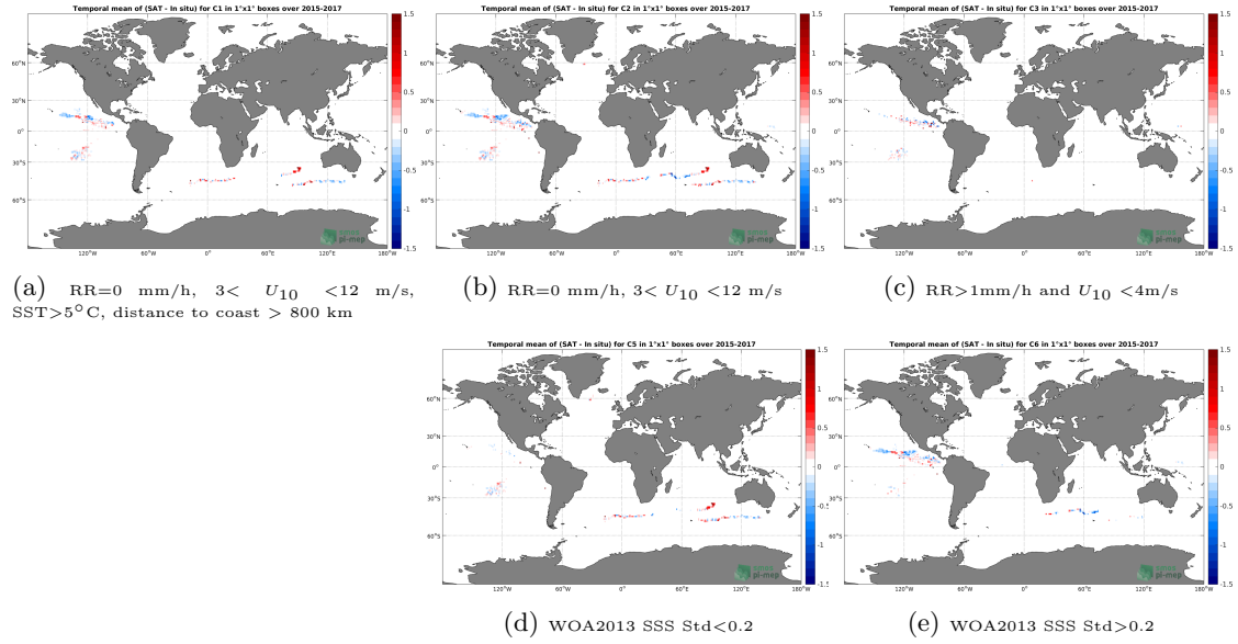
Figure 11: Temporal mean gridded over spatial boxes of size 1^\circ \times 1^\circ of \Delta SSS (SMAP-L3-RSS-V3-8DAY-RUNNING-70KM - Surface drifters) for 5 different subdatasets corresponding to:RR=0 mm/h, 3 < U_{10} < 12 m/s, SST >5^\circ\text{C} , distance to coast > 800 km (a), RR=0 mm/h, 3 < U_{10} < 12 m/s (b), RR >1 mm/h and U_{10} < 4 m/s (c), WOA2013 SSS Std <0.2 (d), WOA2013 SSS Std >0.2 (e).
