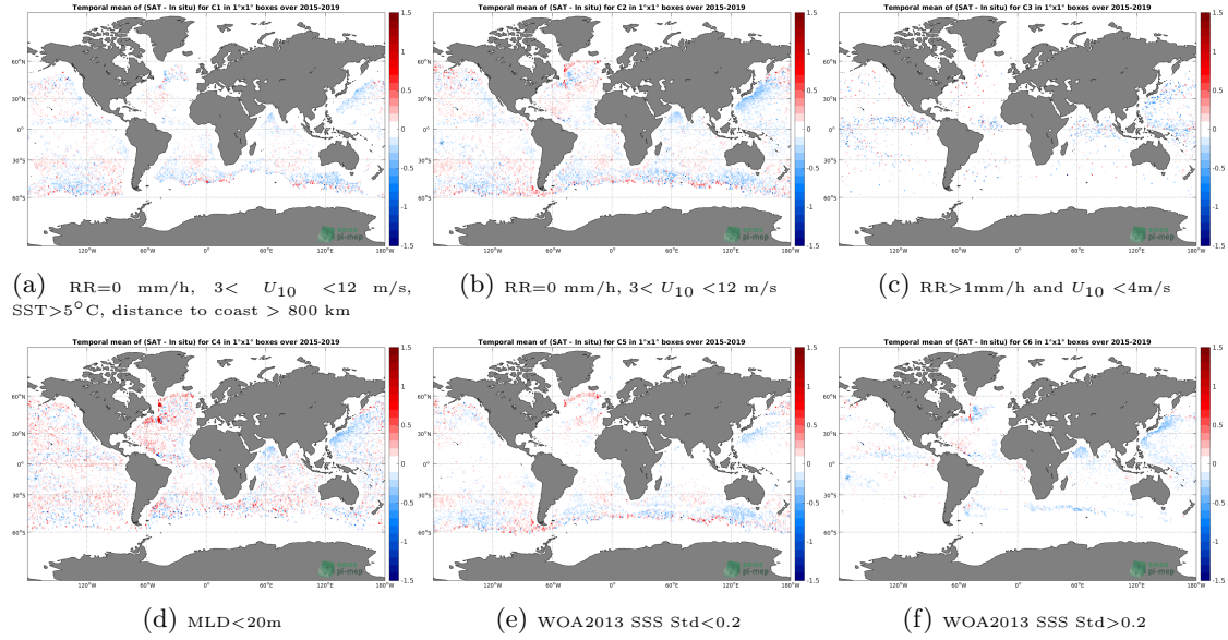
Figure 12: Temporal mean gridded over spatial boxes of size 1^\circ \times 1^\circ of \Delta SSS (SMAP-L3-RSS-V3-8DAY-RUNNING-70KM - Argo) for 6 different subdatasets corresponding to: RR=0 mm/h, 3 < U_{10} < 12 m/s, SST > 5^\circ C , distance to coast > 800 km (a), RR=0 mm/h, 3 < U_{10} < 12 m/s (b), RR > 1 mm/h and U_{10} < 4 m/s (c), MLD < 20 m (d), WOA2013 SSS Std < 0.2 (e), WOA2013 SSS Std > 0.2 (f).
