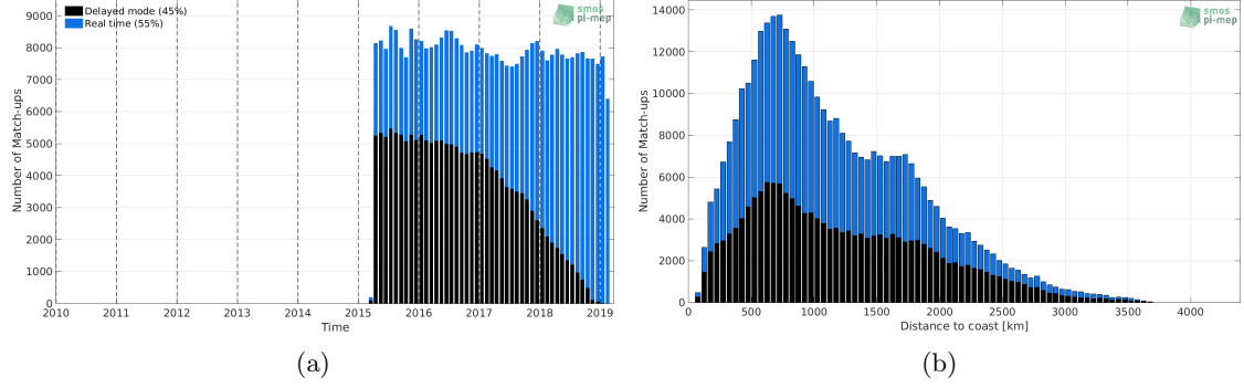
Figure 1: Number of match-ups between Argo and SMAP-L3-RSS-V3-8DAY-RUNNING-70KM SSS as a function of time (a) and as function of the distance to coast (b) over the Global Ocean Pi-MEP region and for the full satellite product period.
