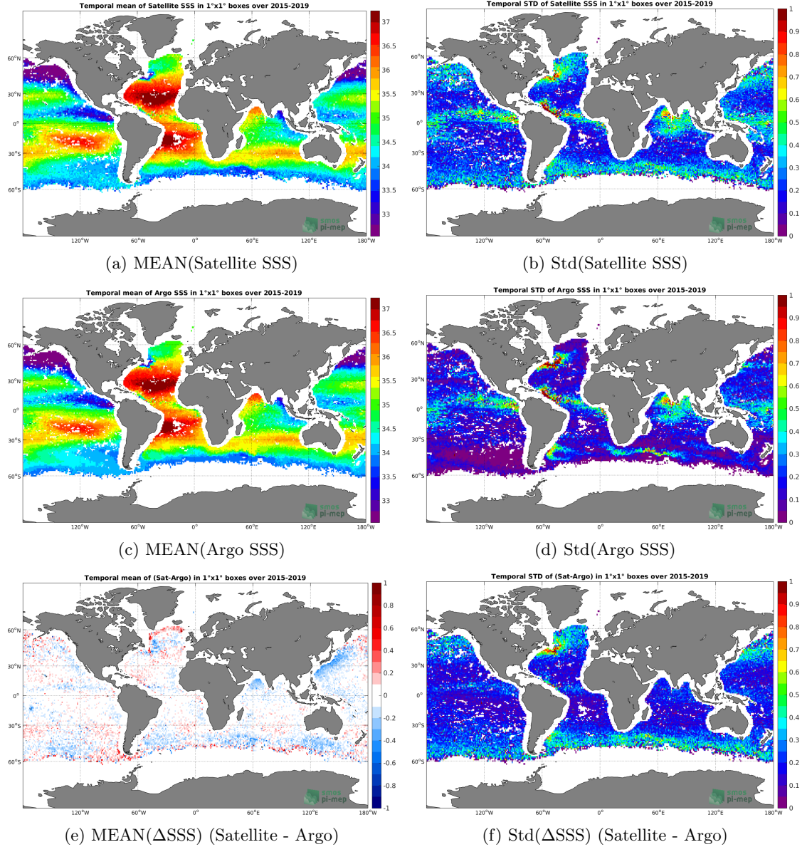
Figure 6: Temporal mean (left) and Std (right) of SSS from SMAP-L3-RSS-V3-8DAY-RUNNING-70KM (top), Argo (middle), and of \Delta SSS (Satellite - Argo). Only match-up pairs are used to generate these maps.
