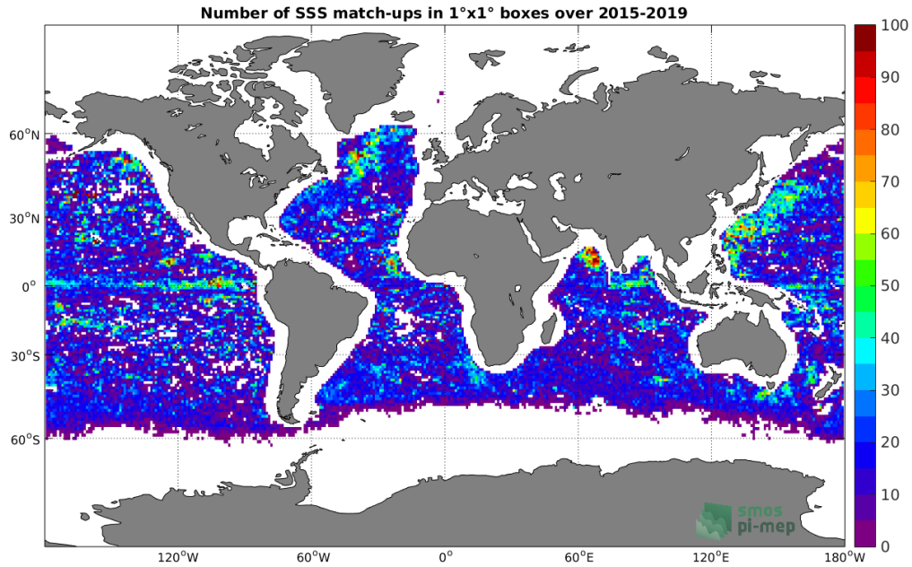
Figure 4: Number of SSS match-ups between Argo SSS and the SMAP-L3-RSS-V3-8DAY-RUNNING-70KM SSS product for the Global Ocean Pi-MEP region over 1^\circ \times 1^\circ boxes and for the full satellite product period.
