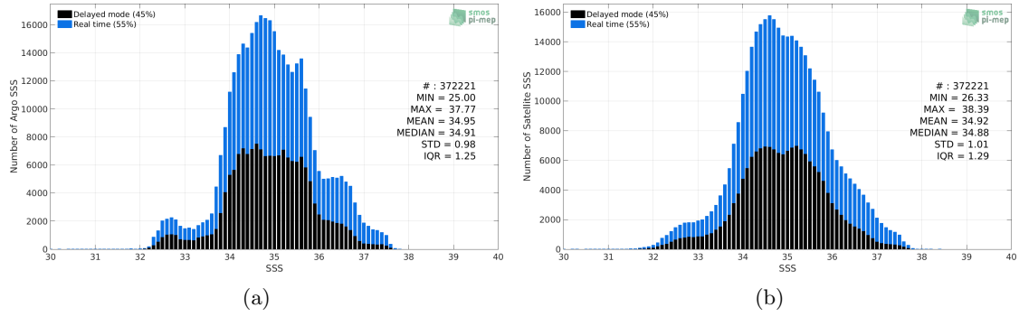
Figure 2: Histograms of SSS from Argo (a) and SMAP-L3-RSS-V3-8DAY-RUNNING-70KM (b) considering all match-up pairs per bins of 0.1 over the Global Ocean Pi-MEP region and for the full satellite product period.
